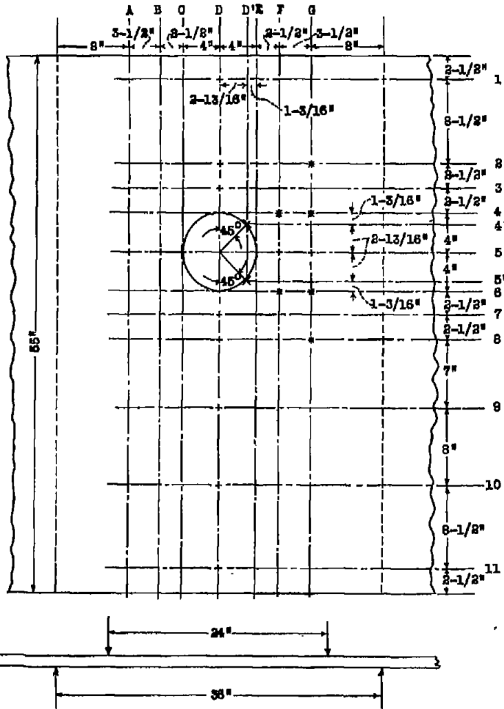
Figure 3.- Location of strain-measurement stations.
