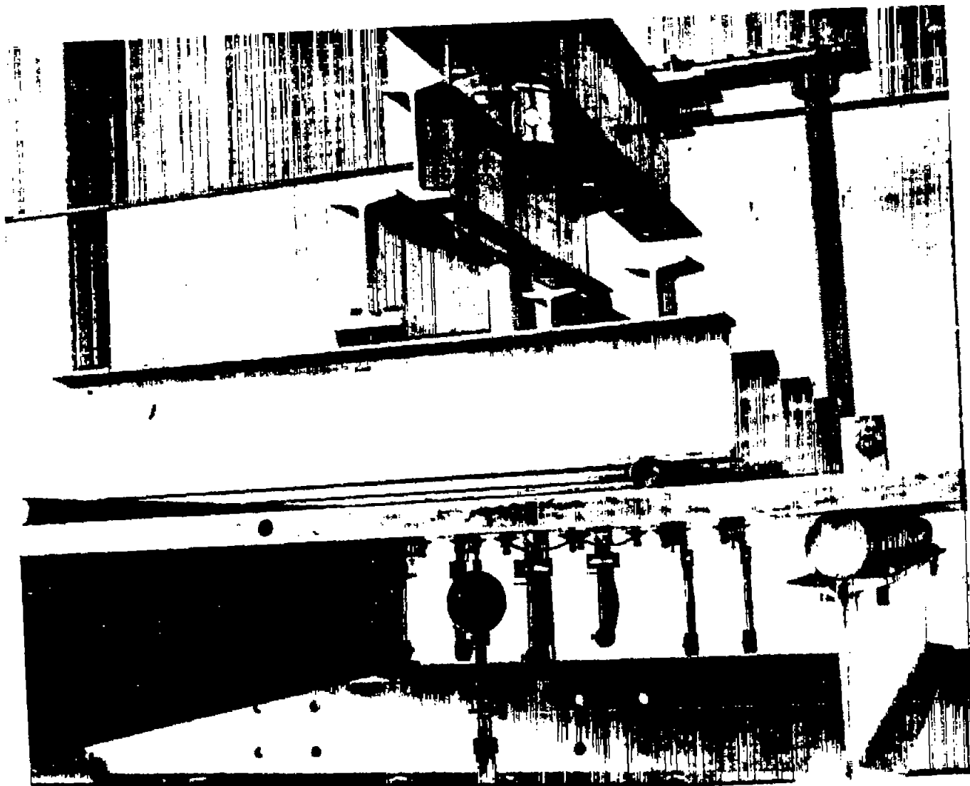
Figure 5. View of plate test showing Huggenberger tensiometers attached to bottom of plate and dial gage used for measuring deflection.
