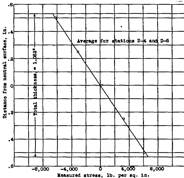
Figure 14.- Stress distribution through thickness of plate.
