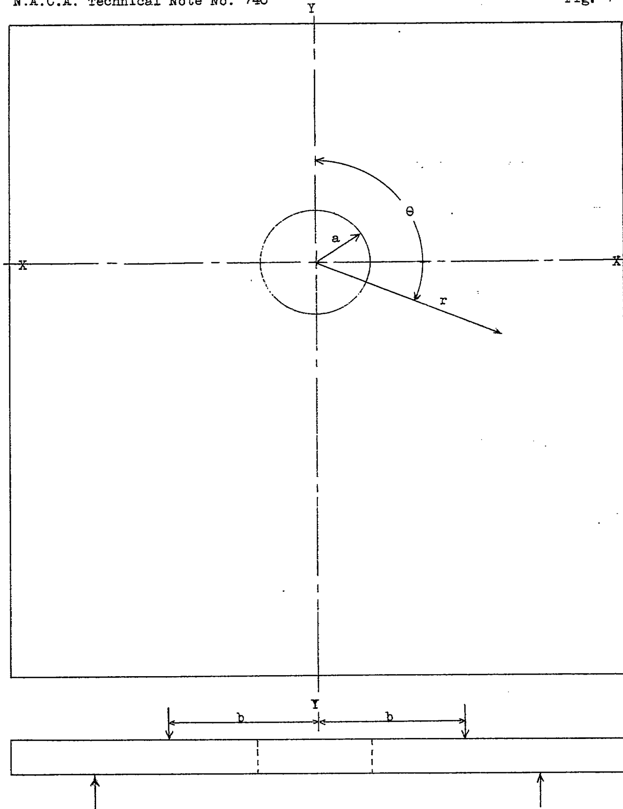
Figure 7.- Coordinate axes of plate..
