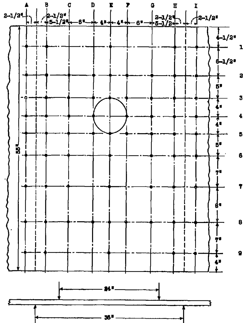
Figure 4.- Location of deflection-measurement stations.
