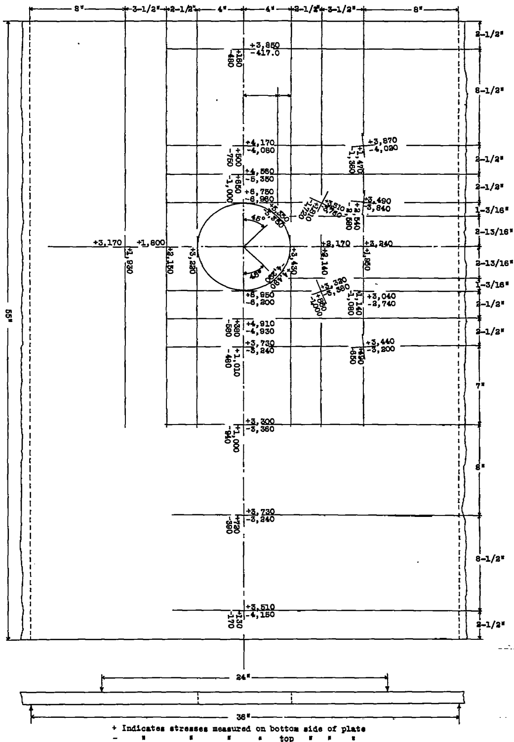
Figure 8.- Stresses measured at various locations on plate.
