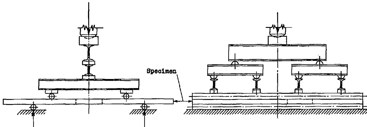
Figure 3.- Method used to support and load plate.
