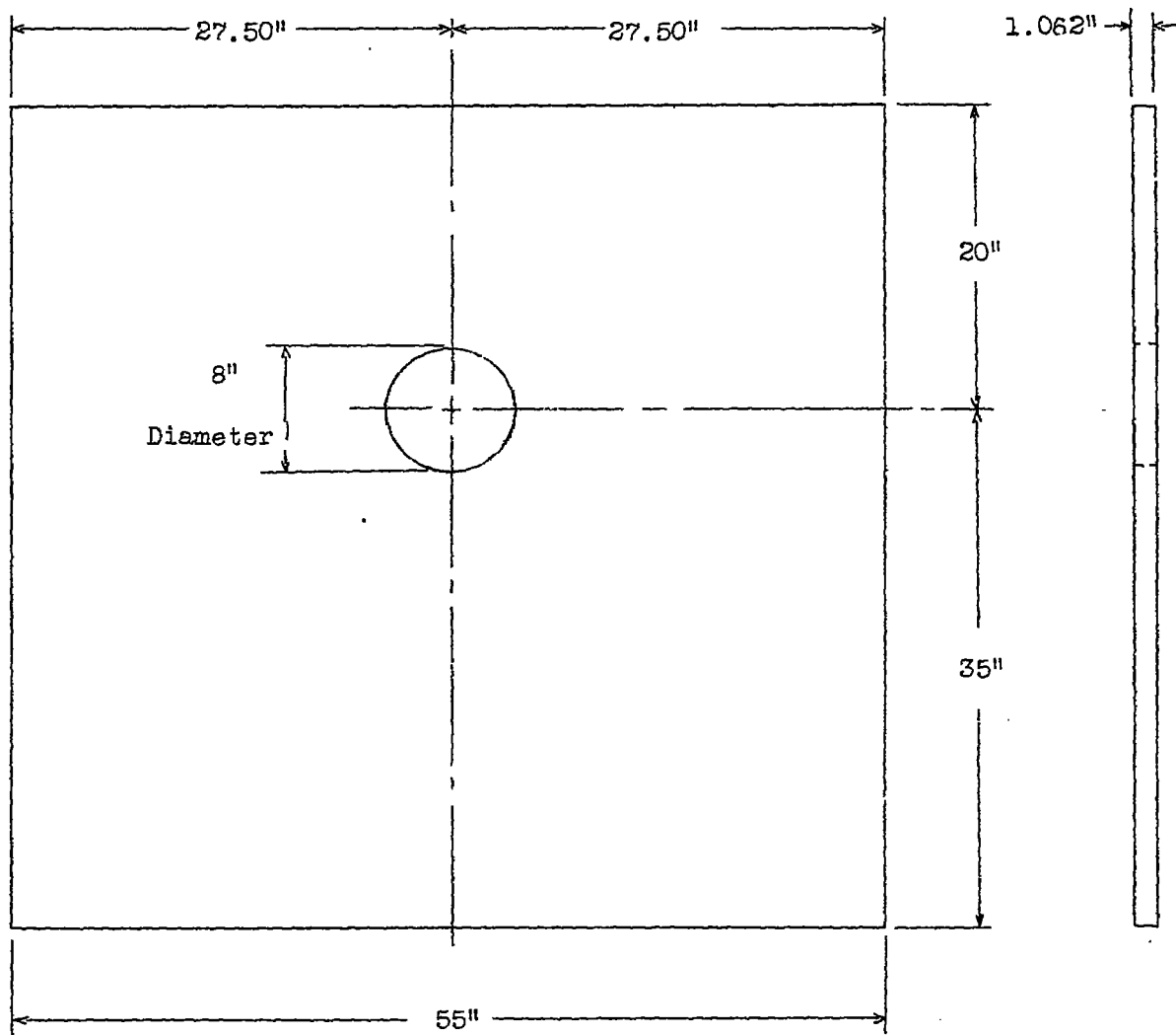
Figure 1.- Detail of plate specimen.
