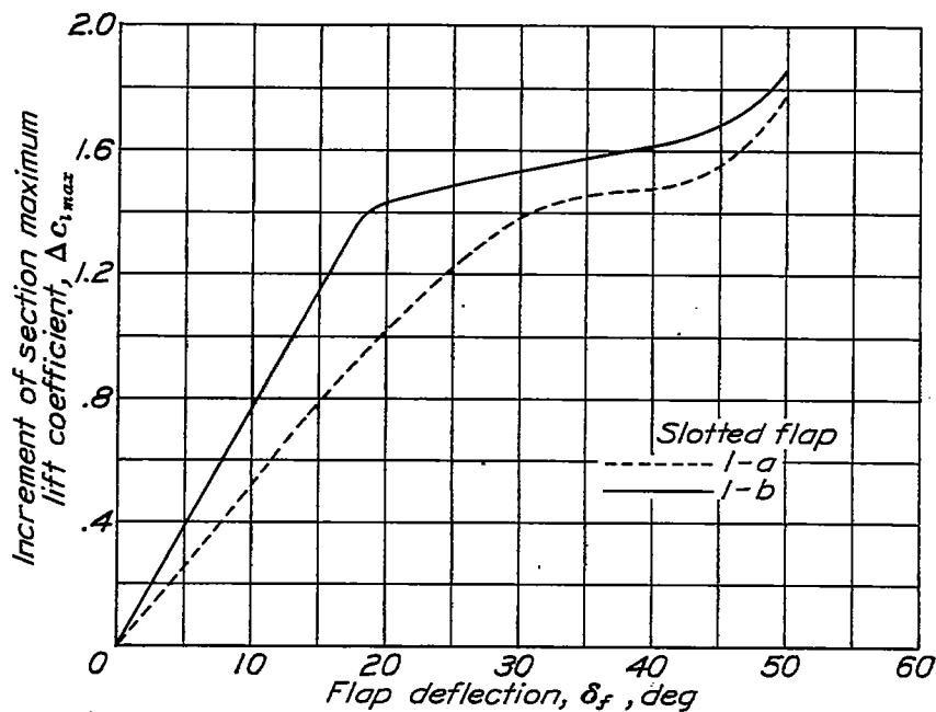
Figure 20.- Comparison of increments of section maximum lift coefficient for flaps 1-a and 1-b when moved and deflected along the selected optimum paths. The N.A.C.A. 23030 airfoil with 0.40c slotted flaps.
