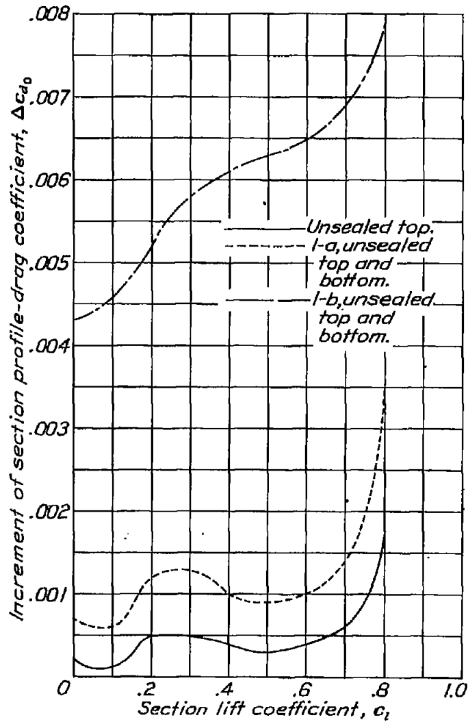
Figure 4.- Effect of slot openings in surface of airfoil on section profile-drag coefficient. The 0.40c slotted flap; \delta_f = 0^\circ
