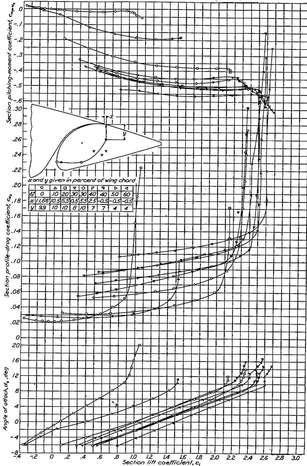
Figure 17.- Section aerodynamic characteristics of N.A.C.A. 23030 airfoil with 0.256c slotted flap I-b.
