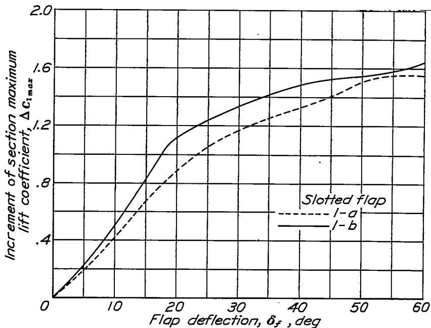
Figure 21.- Comparison of increments of section maximum lift coefficient for flaps 1-a and 1-b when moved and deflected along the selected optimum paths. The N.A.C.A. 23030 airfoil with 0.2566c slotted flaps.
