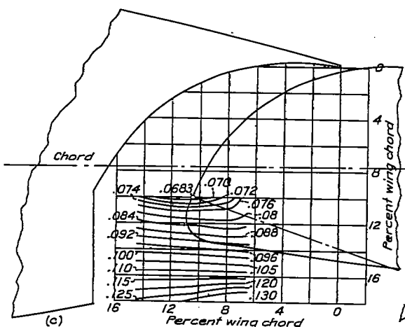
(a) \delta_f = 1.0; c_l = 1.0 ; (b) \delta_f = 10^\circ; c_l = 1.5 . (c) \delta_f = 20^\circ; c_l = 1.5 .
