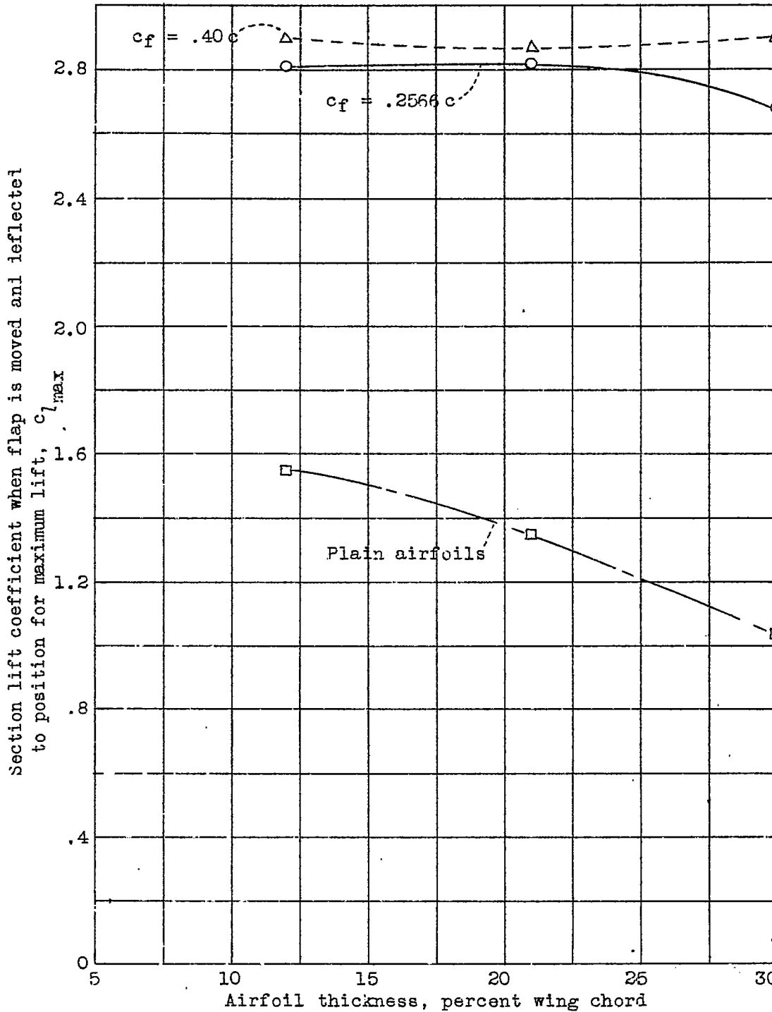
Figure 27.- Effect of airfoil thickness on maximum lift coefficient of N.A.C.A. 230 airfoils with and without slotted flaps.
