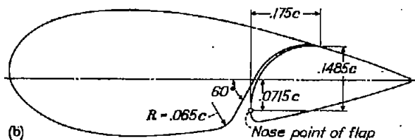
(a) Flap 1-a (b) Flap 1-b Figure 1.- Sections of N.A.C.A. 23030 airfoil with arrangements of 0.40c slotted flap 1.
