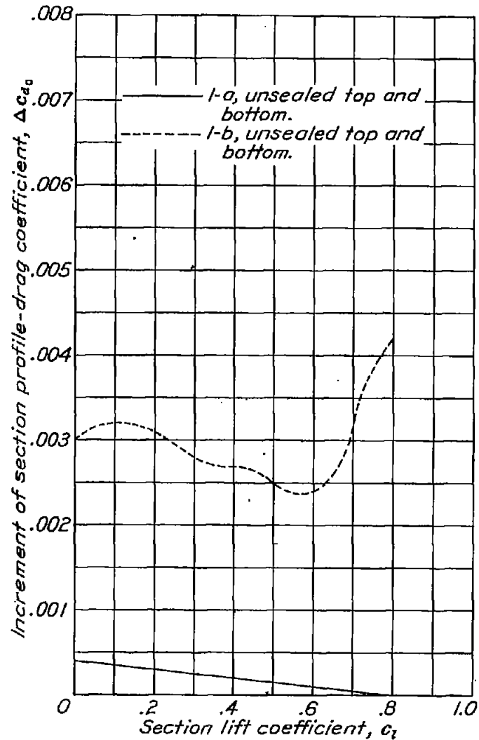
Figure 5.- Effect of slot openings in surface of airfoil on section profile-drag coefficient. The 0.2588c slotted flap; \delta_f = 0^\circ
