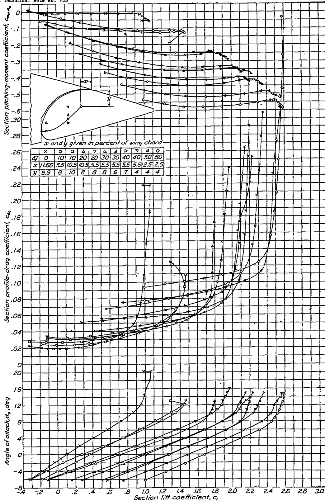
Figure 16.- Section aerodynamic characteristics of W.A.C.A. 23030 airfoil with 0.256c slotted flap 1-a.
