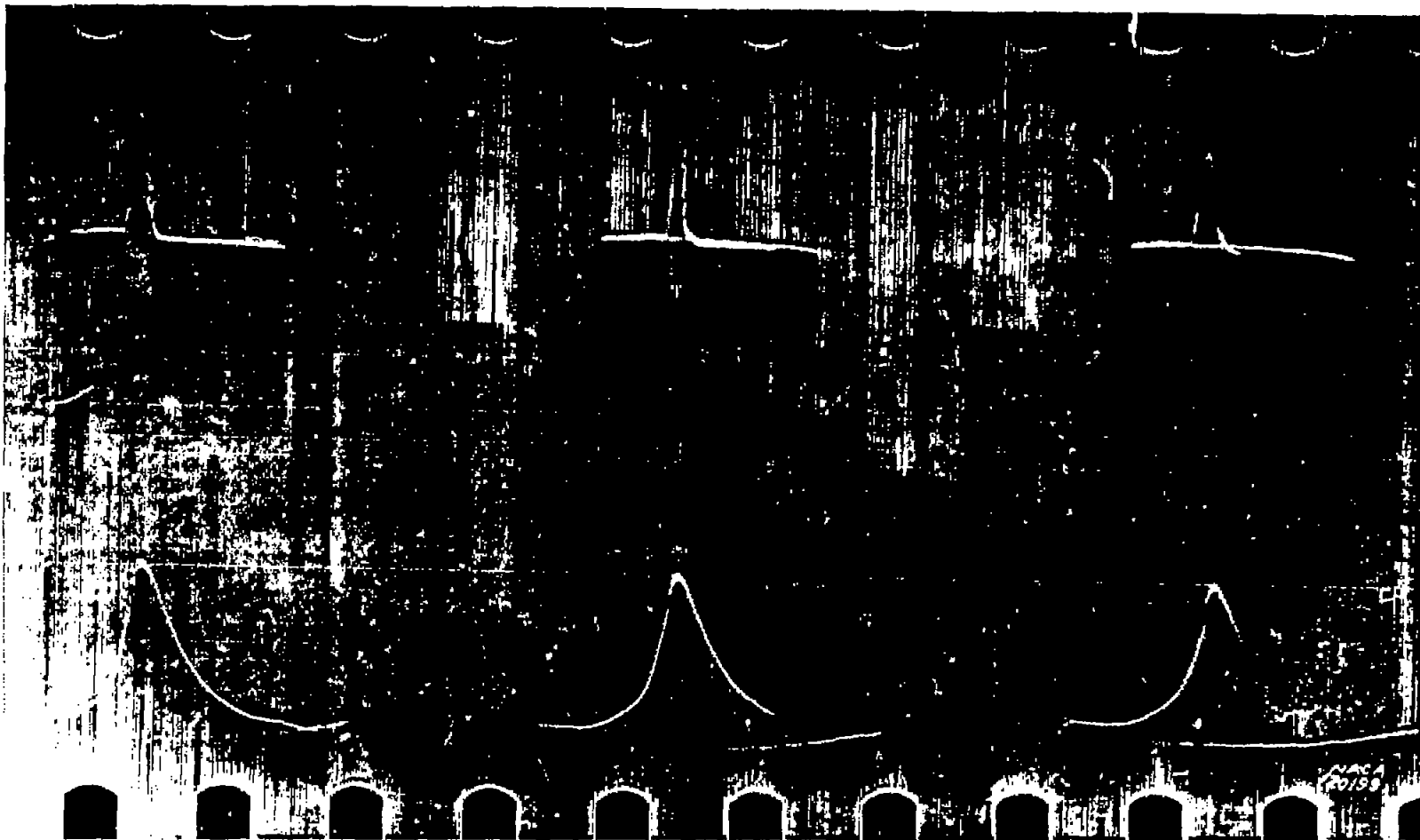
Figure 10.- Ionization-current and cylinder-pressure records of three successive cycles. Hard knock; fuel, commercial gasoline (69 octane); mixture temperature, 200° F.
