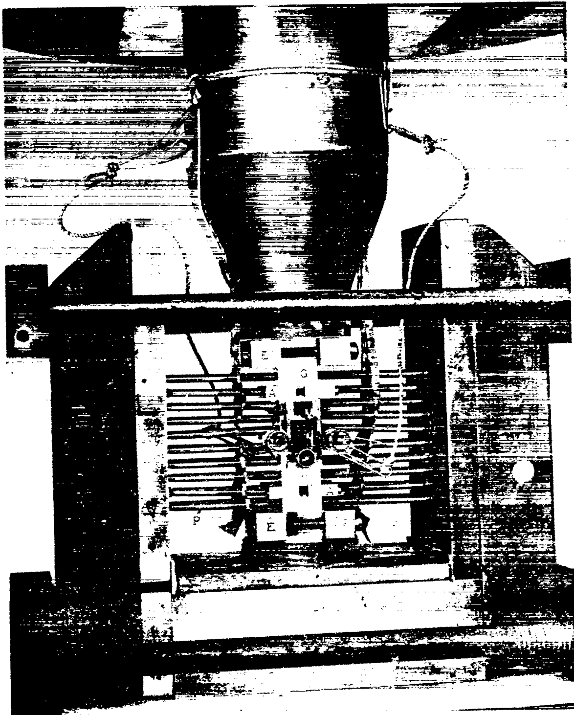
Figure 1 - Pack ready for test.
