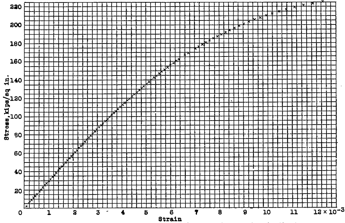
Figure 5.- Stress-strain graph for a pack of 31 specimens taken in the transverse direction from 0.02-inch-thick sheet.
