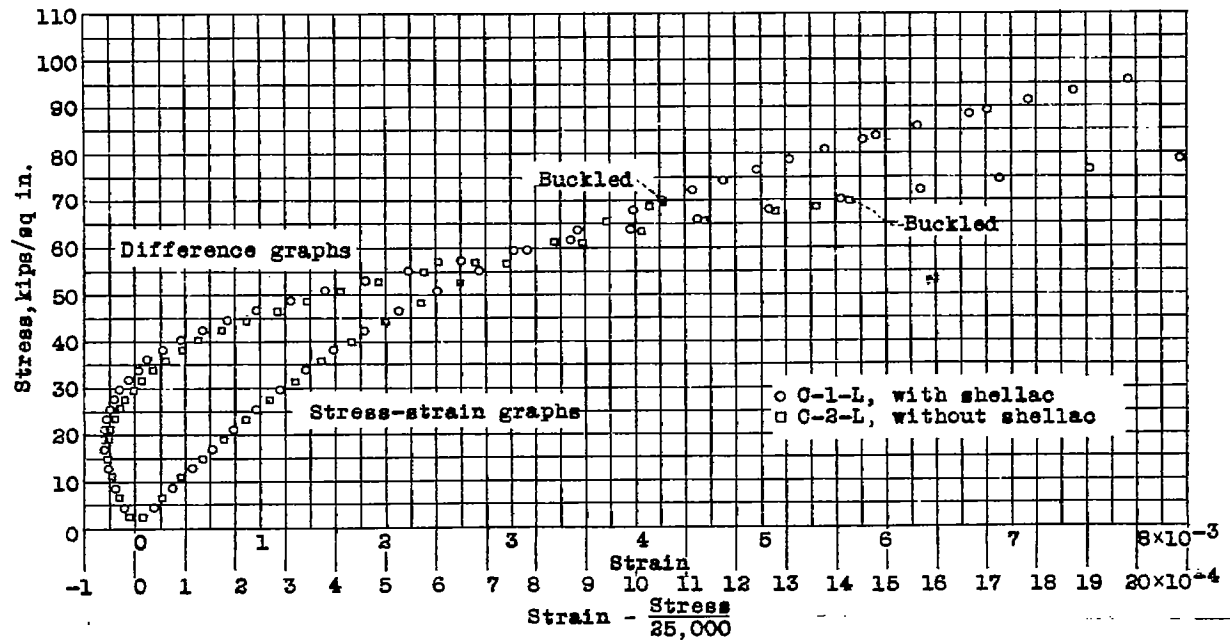
Figure 6.- Stress-strain and difference graphs for packs C1L and C2L from pack compressive tests.
