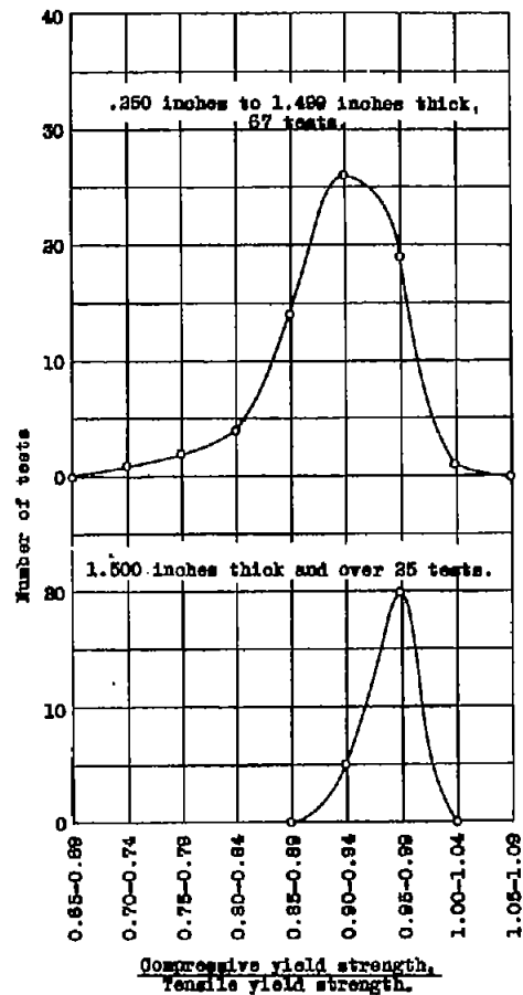
Figure 7.- Frequency curves showing the ratio of compressive yield strength to tensile yield strength for the 67 extruded shapes between 0.250 inches and 1.499 inches thick and the 25 extruded shapes 1.500 inches thick and over.
