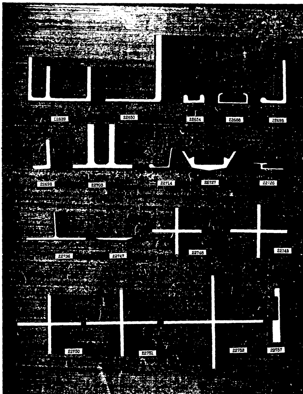
Figure 1e.- Cross sections of 24S-T Extruded Shapes Tested - Die Nos. 22639 to 22757
