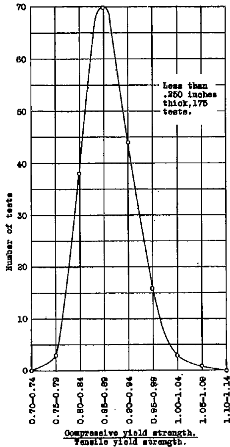
Figure 6.- Frequency curves showing the ratio of compressive yield strength to tensile yield strength for the 175 extruded shapes less than 0.250 inches thick.
