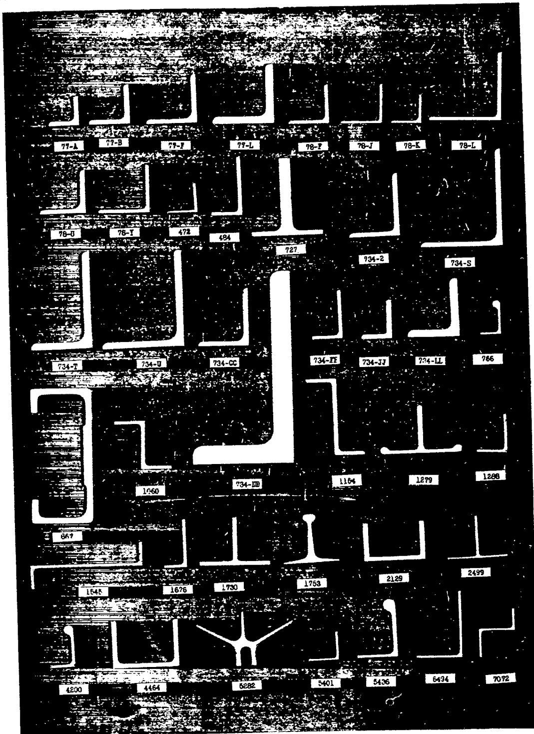
Figure 1a.-Cross sections of 24S-T Extruded Shapes Tested - Die Nos. 77-A to 7072
