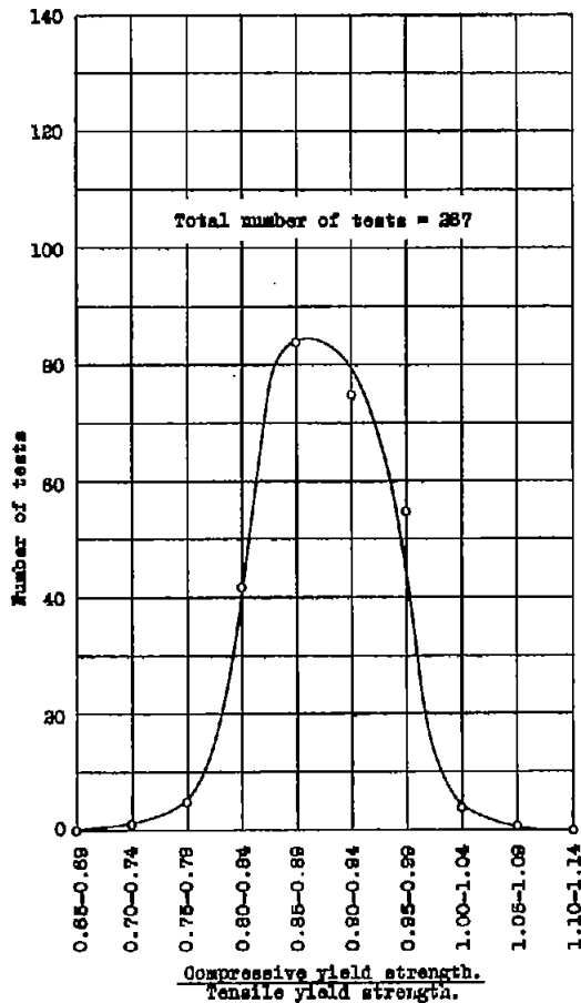
Figure 5.- Frequency curves showing the ratio of compressive yield strength to tensile yield strength for the 287 extruded shapes of 248T aluminum alloy tested.
