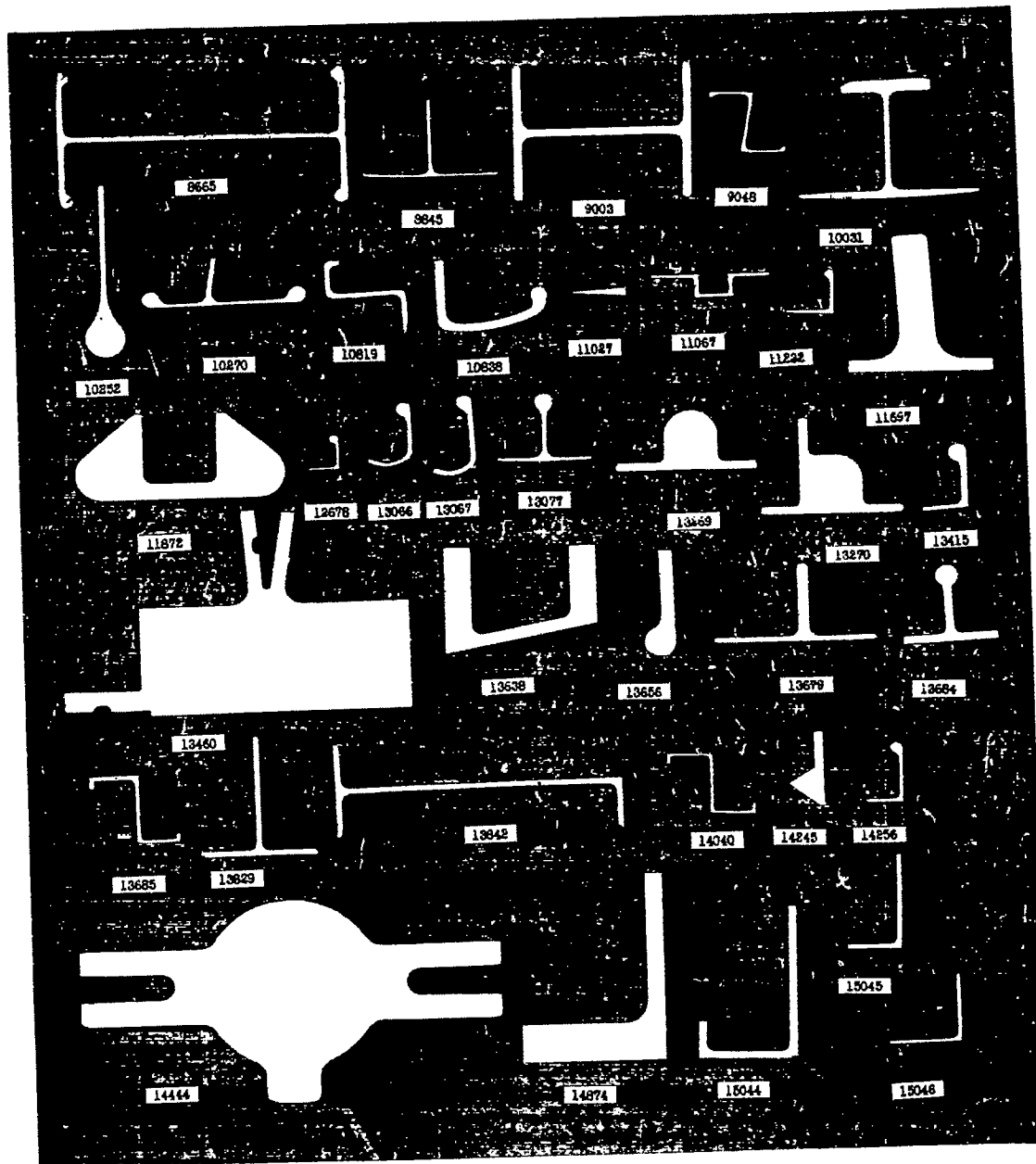
Figure 1b.-Cross sections of 24S-T Extruded Shapes Tested - Die Nos. 8665 to 15046
