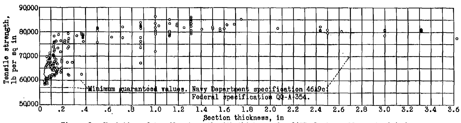
Figure 2.- Variation of tensile strength with thickness for 24ST aluminum alloy extruded shapes.
