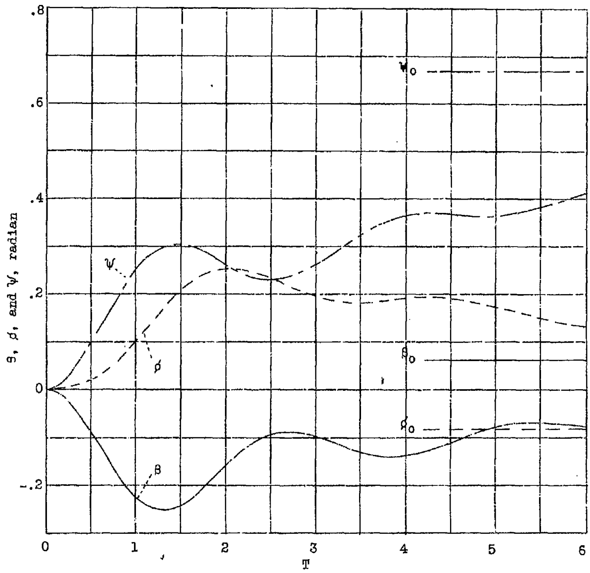
Figure 3.- Resultant motions for case 3.
