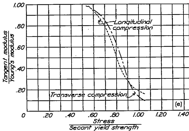
Figure 2.- Sheet 8. Aluminum alloy 178-T; thickness, 0.051 inch.
