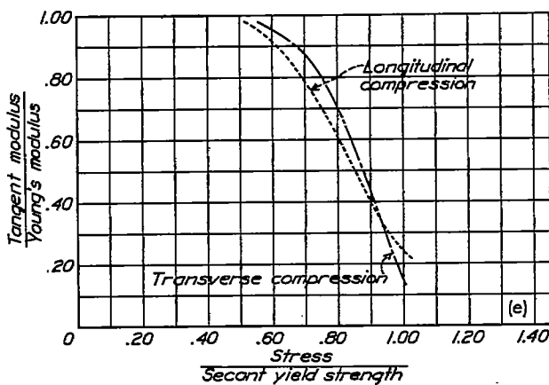
Figure 10.- Sheet 10. Aluminum alloy 24S-RT; thickness, 0.081 inch.
