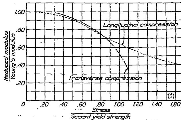
Figure 19.- Sheet 19. Chromium-nickel steel full hard; thickness, 0.024 inch.
