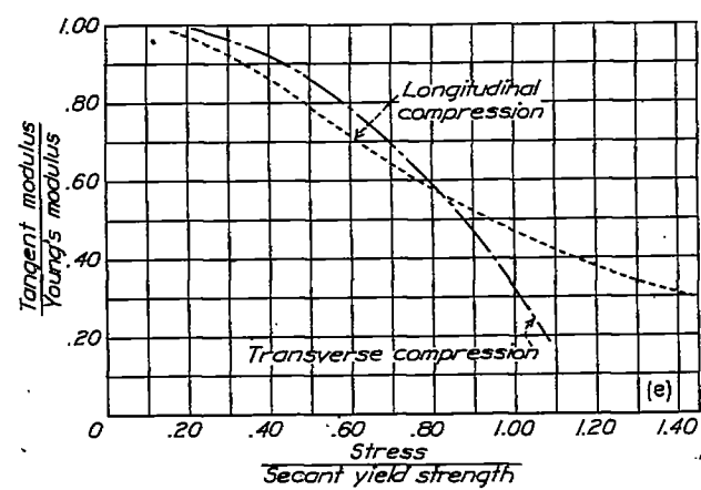
Figure 17.- Sheet 17. Chromium-nickel steel full hard; thickness, 0.020 inch.
