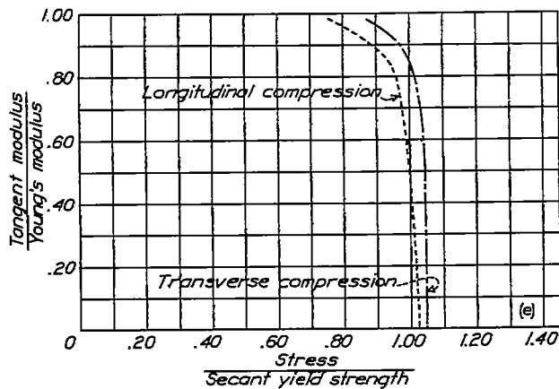
Figure 12.- Sheet 12. 1025 carbon steel; thickness, 0.054 inch.
