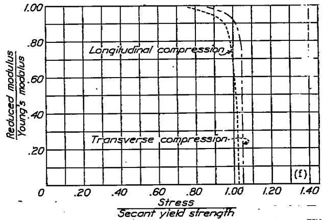
Figure 12.- Sheet 12. 1025 carbon steel; thickness, 0.054 inch.
