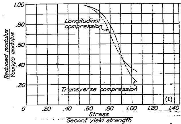
Figure 2.- Sheet 8. Aluminum alloy 178-T; thickness, 0.051 inch.
