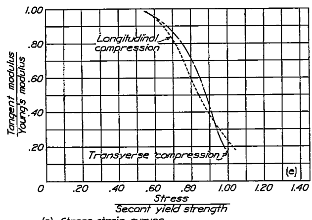
Figure 8.- Sheet 8. Aluminum alloy 24S-RT; thickness, 0.051 inch.
