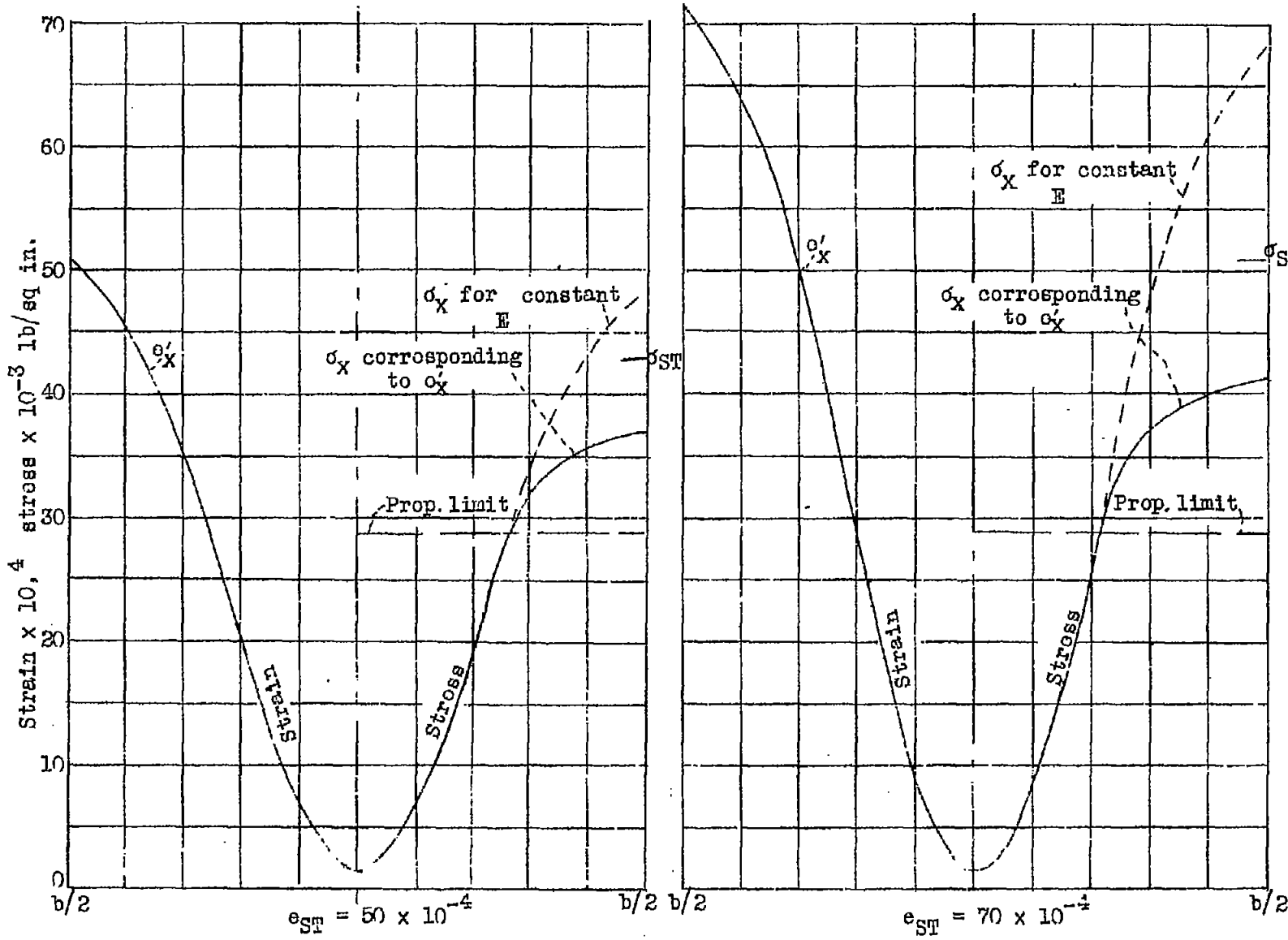
Figure 20.- Axial strain and stress distribution beyond proportional limit
