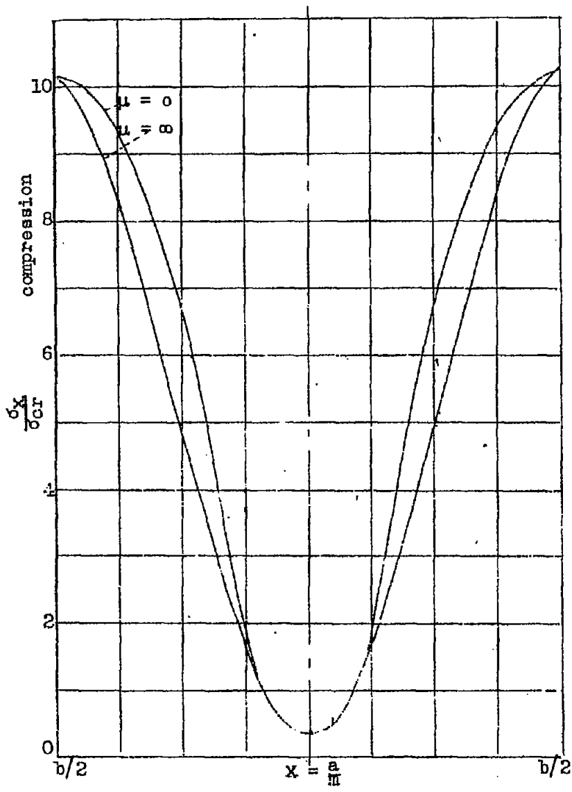
Figure 14.- Axial stress distribution for \frac{\sigma_{SF}}{\sigma_{cr}} = 10 .
