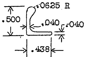
Bulb angle No. 1
