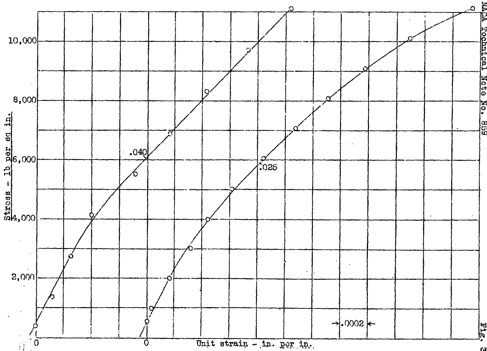
Figure 39.- Bulb angle 1, 24ST sheet, panel width, = 15 in., total stringer area = 0.1150 sq in.
