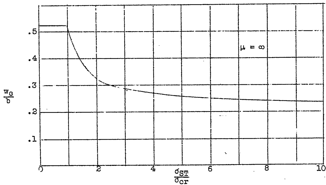
Figure 17.- Mean effective width as a function of \frac{\sigma_{ST}}{\sigma_{cr}} ( E_S = E_{ST} )
