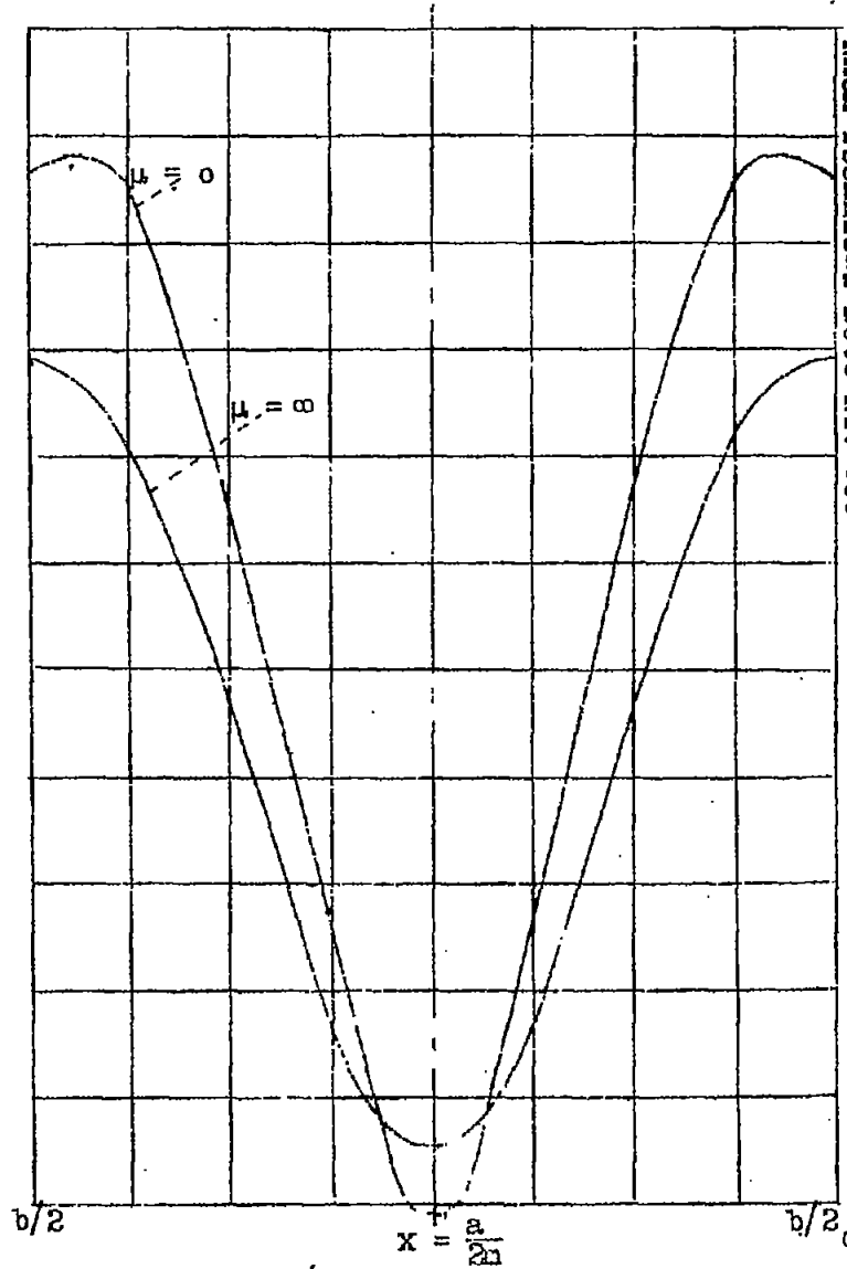
Figure 14.- Axial stress distribution for \frac{\sigma_{SF}}{\sigma_{cr}} = 10 .
