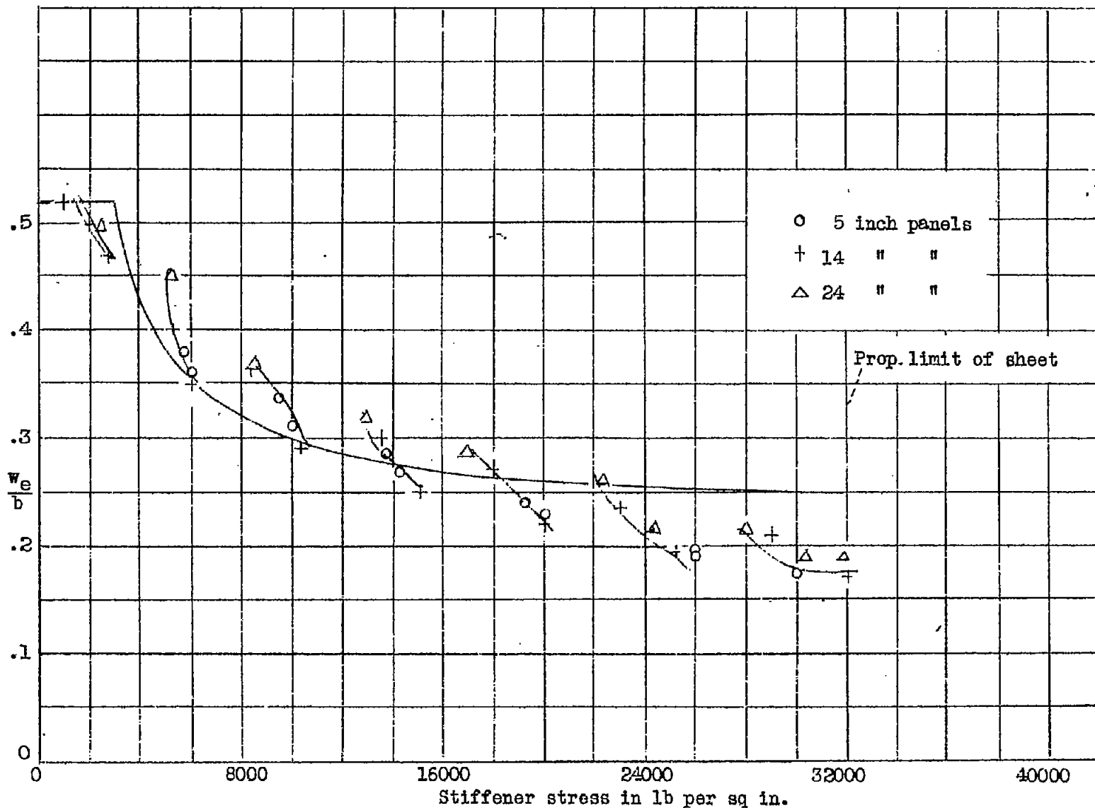
Figure 18.- Effective width curve, 3 stiffener panels, 040 24ST alclad sheet, J-section 161
