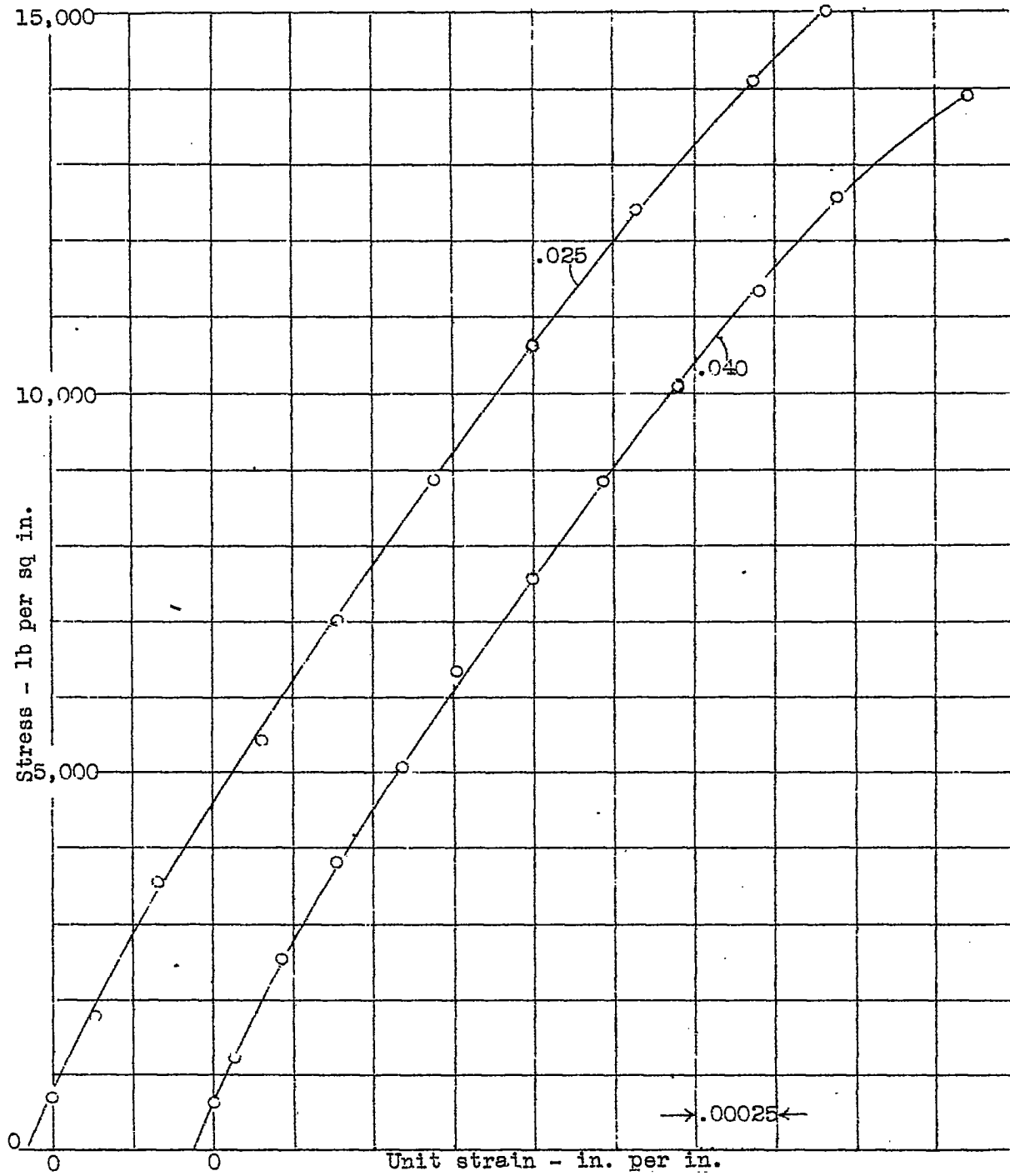
Figure 38.- Bulb angle 10265, 24ST sheet, panel width = 15 in., total stringer area = 0.1910 sq in.
