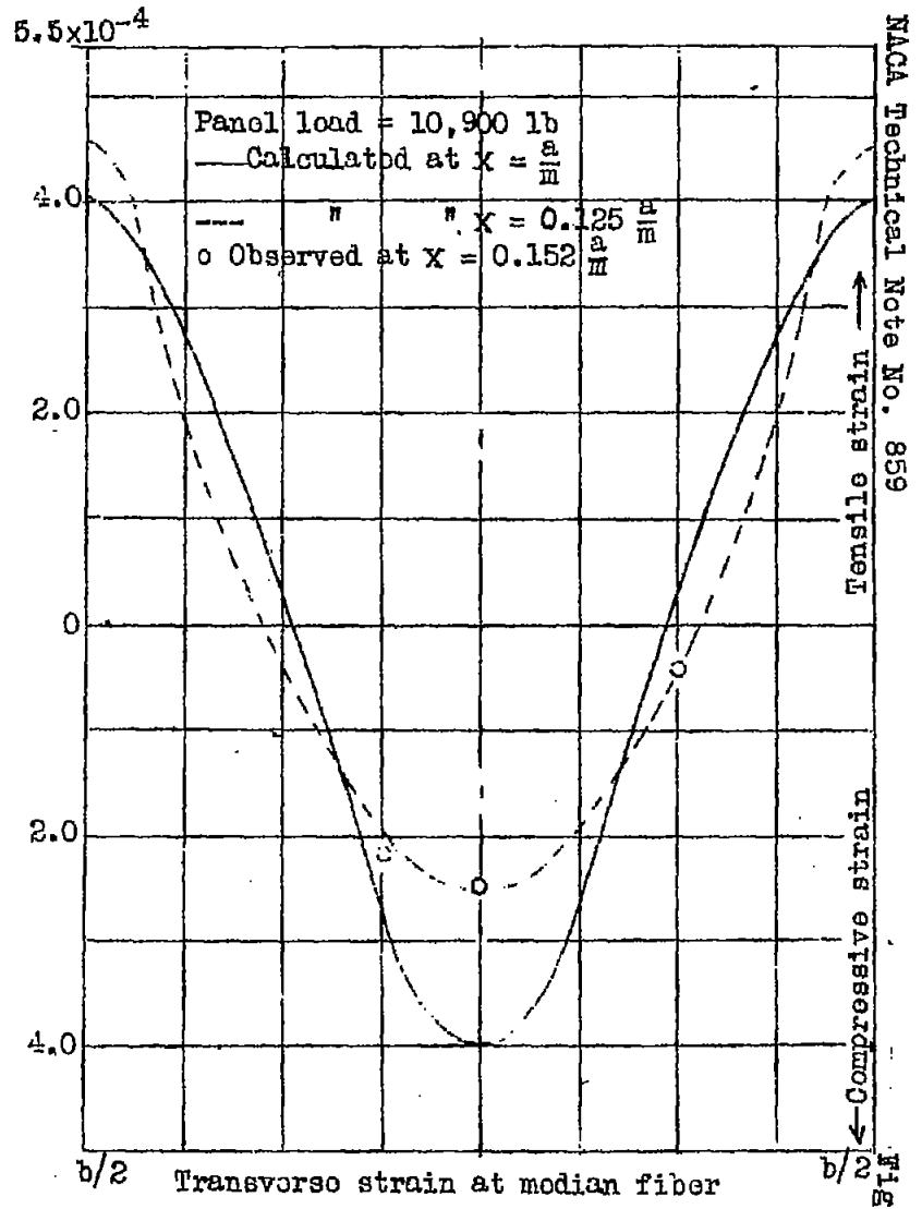
Figure 25.- Comparison of calculated strain distribution with experimental results given in ref. 4.
