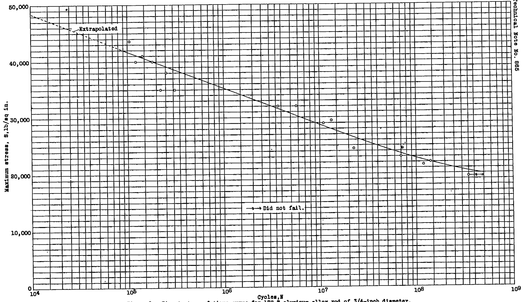
Figure 1.- Direct-stress fatigue curve for 17S-T aluminum-alloy rod of 3/4-inch diameter. Nominal ratio of minimum to maximum stress is equal to zero.
