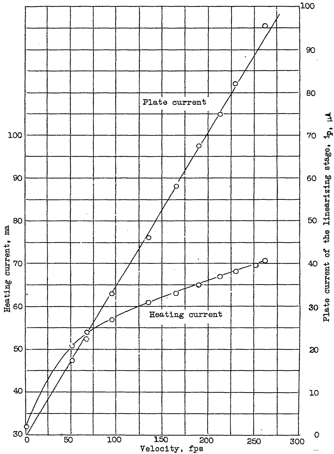
Figure 5.- Calibration curve of the circuit adjusted to linear characteristic.
