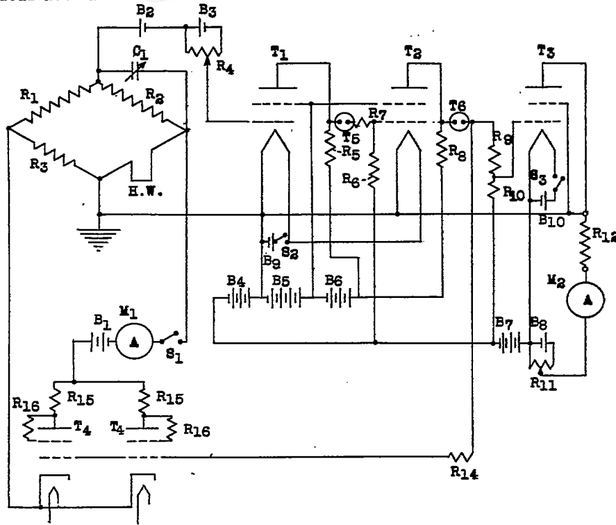
Figure 2.- Hot-wire circuit.
