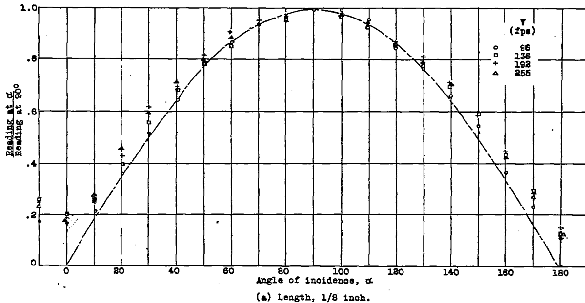
Figure 7.- Directional characteristics for constant-resistance operation and adjustment to linearity of reading. Nickel wire, 0.0005 inch in diameter.
