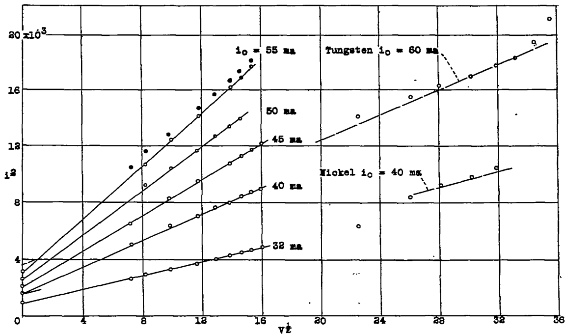
Figure 4.- Heating current for constant-resistance operation plotted for check of conformity with King's relation.
