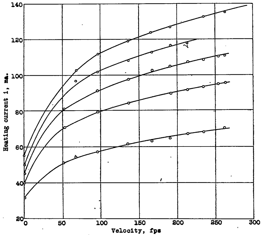
Figure 3.- Heating current of a hot wire at constant-resistance operation.
