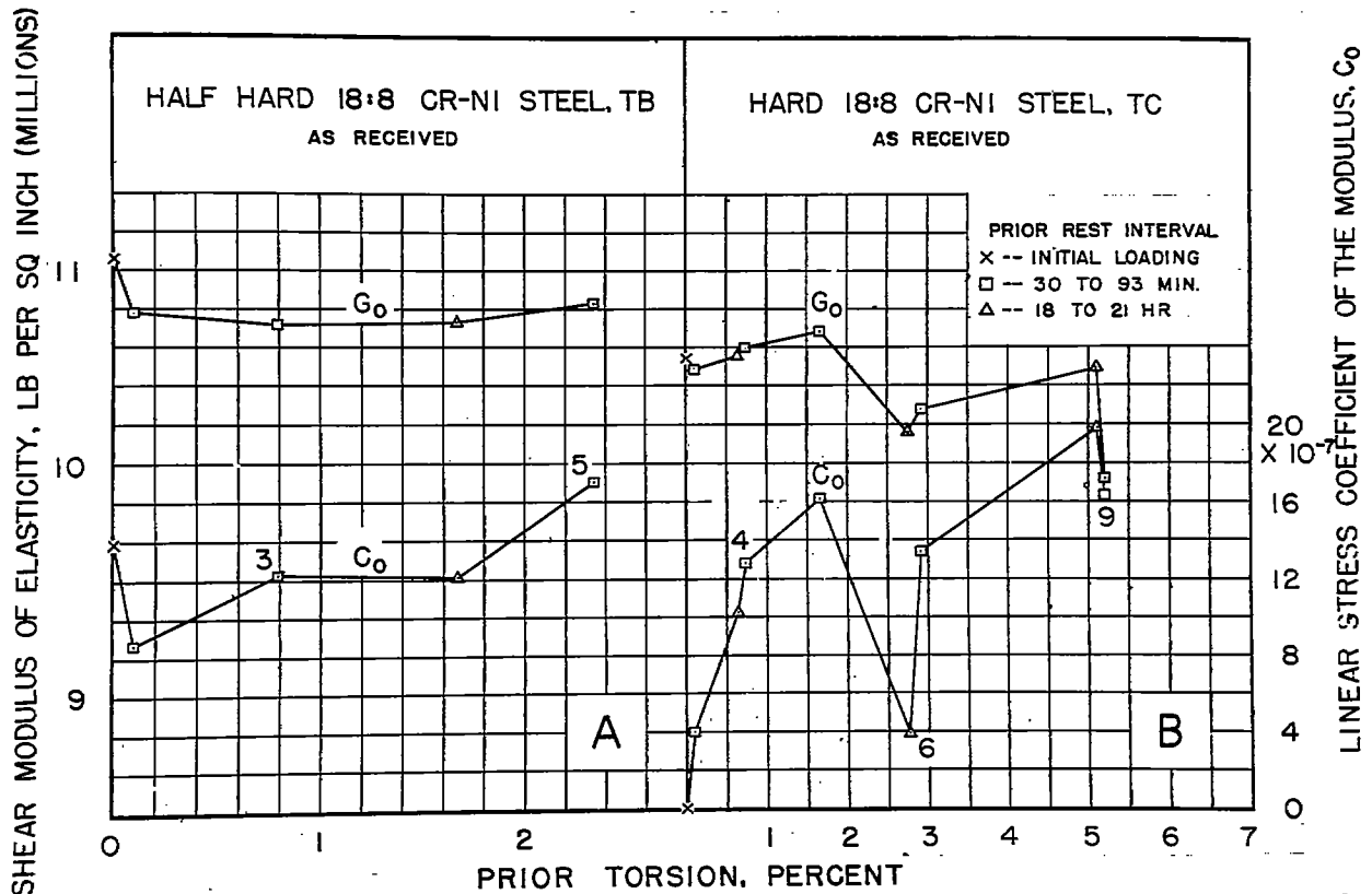
Figure 15. Variation of the shear modulus of elasticity and of its linear stress coefficient with prior torsion for cold-drawn 18:8 chromium-nickel steel.
