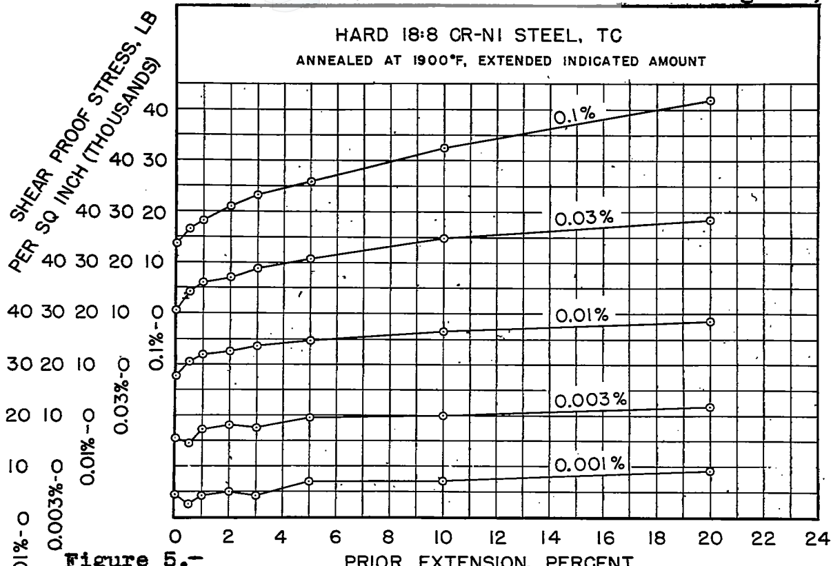
Figure 5.- Variation of shear proof stresses with prior extension for fully annealed 18:8 chromium-nickel steel TC-19. (Measure with 1/50")
