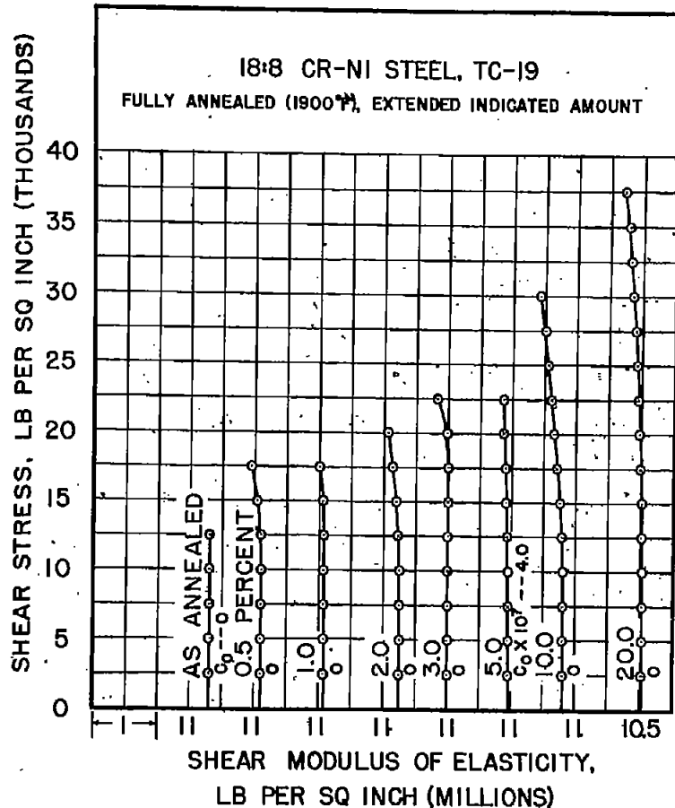
Figure 4.- Shear stress-modulus lines for fully annealed 18:8 chromium-nickel steel TC-19 as influenced by prior extension. (Measure with \frac{1}{50} ").
