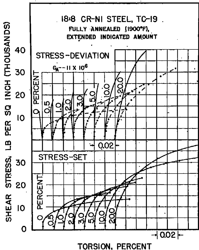
Figure 3.- Shear stress-deviation and stress-set curves for fully annealed 18:8 chromium-nickel steel TC-19 as influenced by prior extension.
