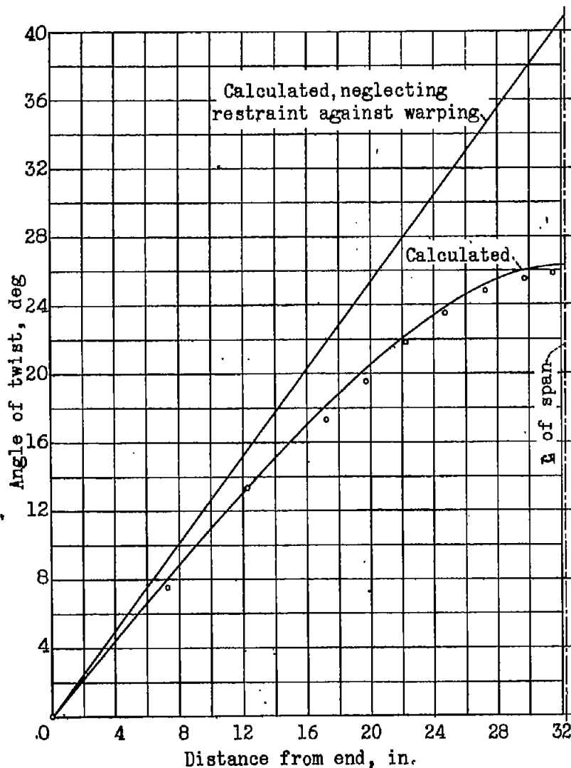
Specimen, I-beam of X74S-T aluminum alloy; torque, 780 inch-pounds.
