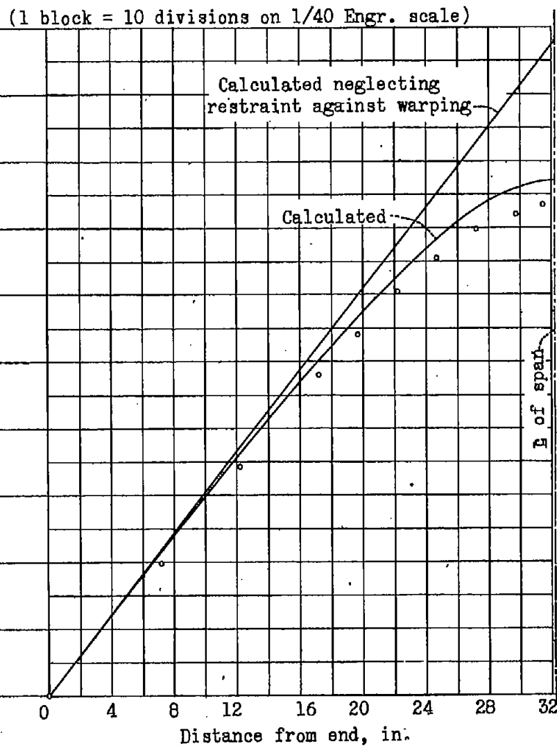
Specimen, channel of X74S-T aluminum alloy; torque, 488 inch-pounds.
