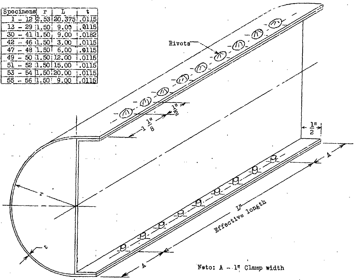
Figure 1.- Details of "D" sections.
