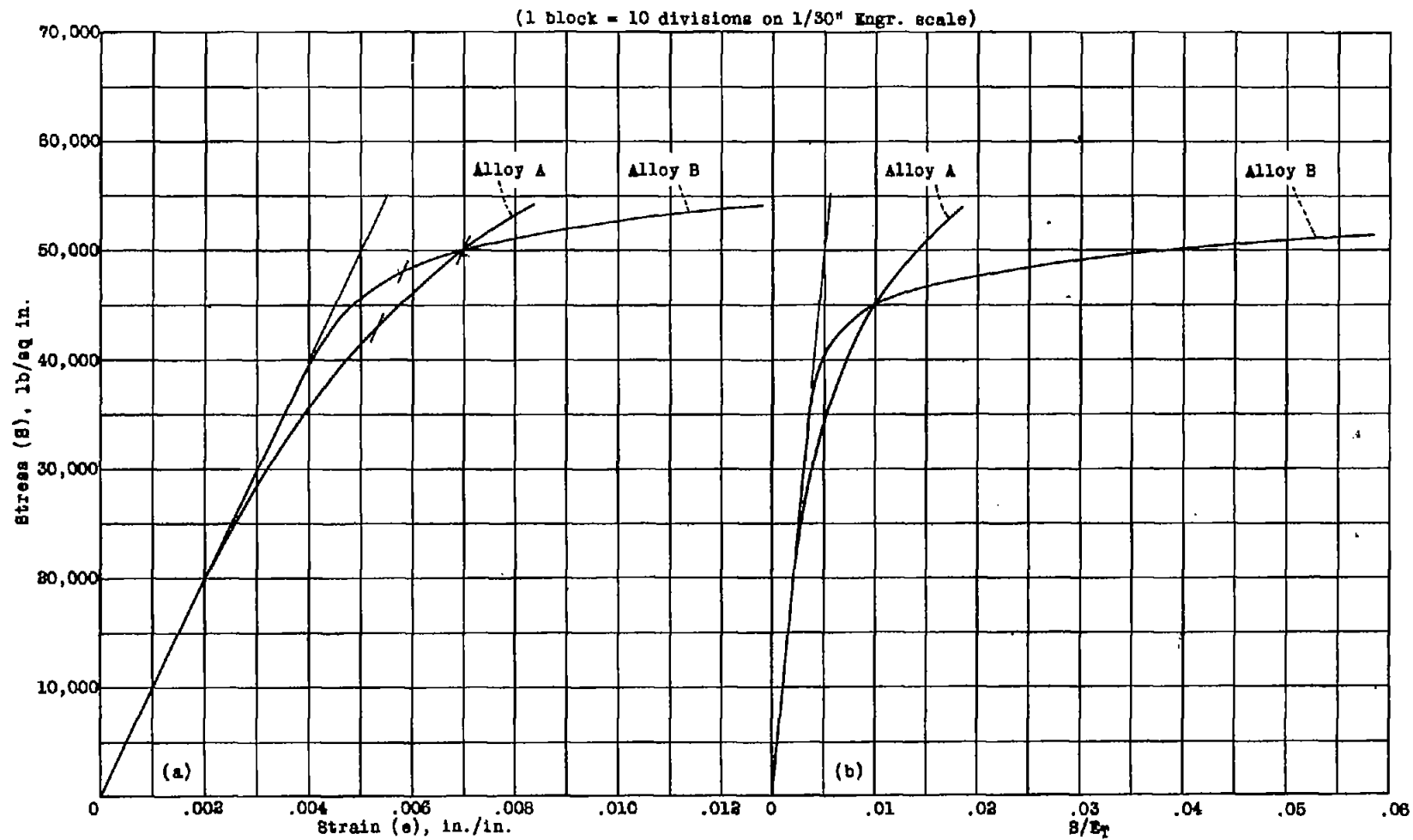
Figure 1.- Stress-strain and stress- B/Et curves for two alloys having the same modulus and the same yield strength (0.003 offset), but with different stress-strain curves.
