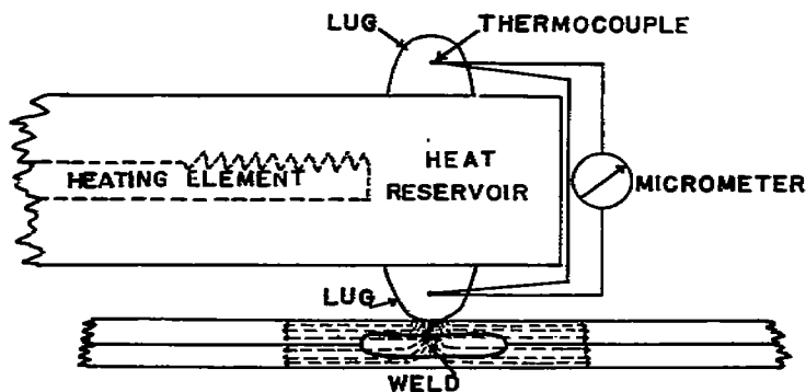
FIG. 26.- HEAT RESERVOIR THERMAL TEST OF THE BONDED AREA AT THE FAYING PLANE OF THE SPOTWELD.
