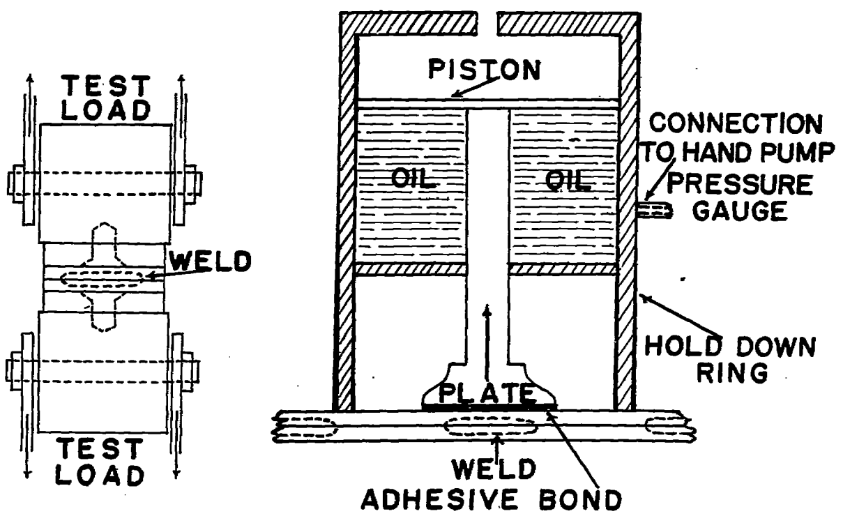
B. TENSION TESTING OF WELD
