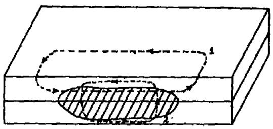
FIG. 19.—EFFECT OF PLANE OF FLOW OF EDDY CURRENT UPON MEASUREMENT OF BONDED AREA AT THE FAYING PLANE OF THE SPOTWELD. A. EDDY CURRENTS FLOWING IN PATH 1 PARALLEL TO THE FAYING SURFACE DO NOT MEASURE AREA OF BONDING. B. EDDY CURRENTS FLOWING IN PATH 2 NORMAL TO THE FAYING SURFACE DO MEASURE AREA OF BONDING.
