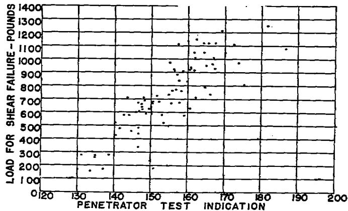
B. 135 TAYLOR WINFIELD SPOTWELDS MADE ON LABORATORY WELDER AT UNIVERSITY OF SOUTHERN CALIFORNIA IN .040" 24ST ALCLAD. [COMPARE WITH FIG. 41 H.]
