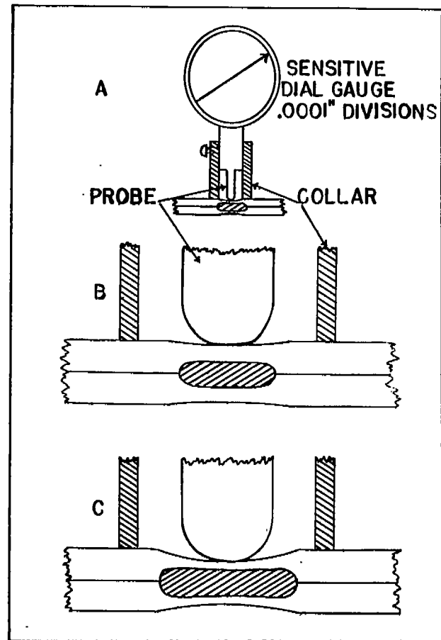
A. DIAL GAUGE WITH COLLAR B. SMALL INDENTATION OVER SMALL WELD C. LARGE INDENTATION OVER LARGE WELD D. RESULTS OF INDENTATION TESTS ON 141 SCIAYKY WELDS IN .040" 24ST ALCLAD.
