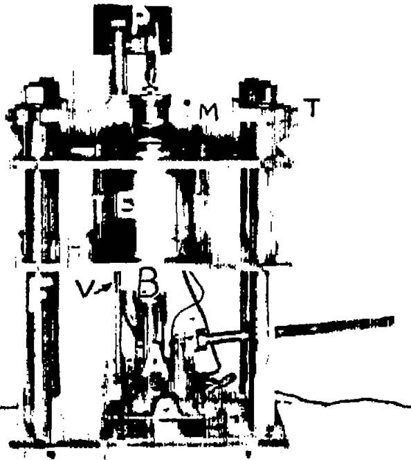
FIG. 38a. - SIDE VIEW OF ASSEMBLED MACHINE.
