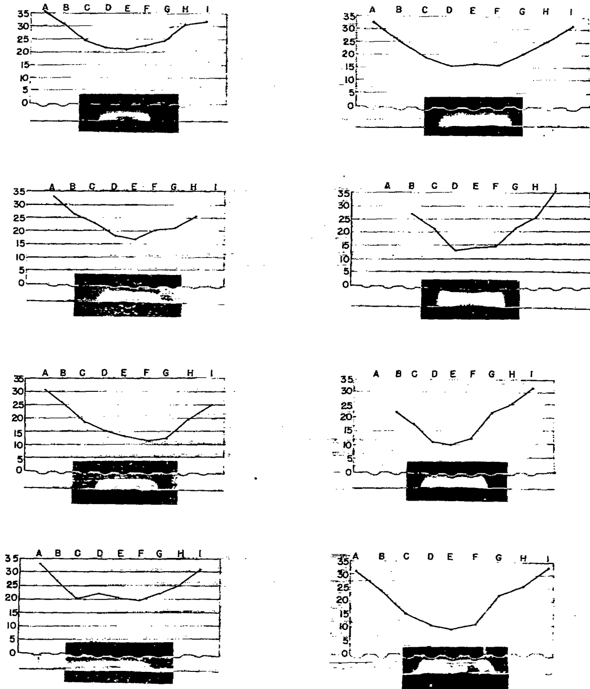
FIG. 34.-CHARACTERISTIC PENETRATOR PROFILES OF SPOTWELDS
