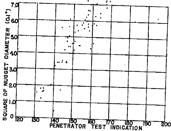
D. 105 TAYLOR WINFIELD SPOTWELDS MADE ON THE LABORATORY WELDER AT THE UNIVERSITY OF SOUTHERN CALIFORNIA IN .040" 24ST ALCLAD.
