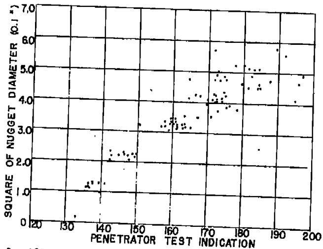
C. 105 TAYLOR WINFIELD SPOTWELDS MADE ON THE LABORATORY WELDER AT THE UNIVERSITY OF SOUTHERN CALIFORNIA IN .040" 24ST ALCLAD.
