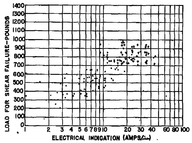
B. 141 WELDS IN .040" 24ST ALCLAD MADE ON SCIACKY WELDER AT LOCKHEED AIRCRAFT CORPORATION.
