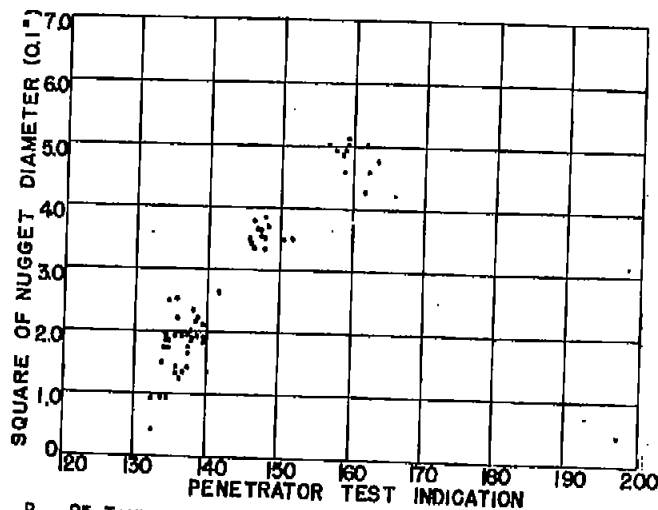
B. 85 TAYLOR WINFIELD SPOTWELDS MADE ON THE LABORATORY WELDER AT THE UNIVERSITY OF SOUTHERN CALIFORNIA IN .040" 24ST ALCLAD.
