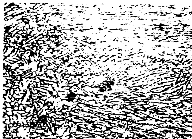
(c I ). DENDRITIC ZONE OF NUGGET. 500X.
