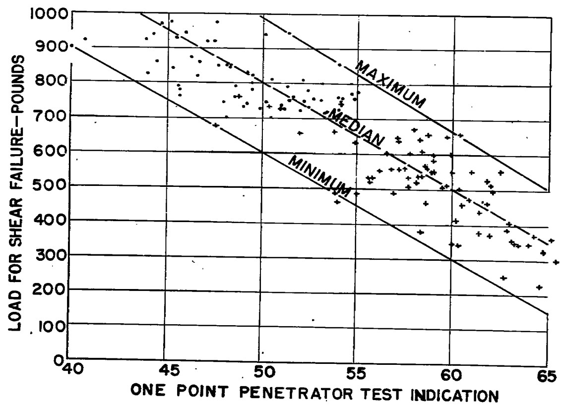
FIG. 33.— RESULTS OF ONE POINT ONE SIDE PENETRATOR TEST OF 141 SCIAYK WELDS IN .040" 24ST ALCLAD.
