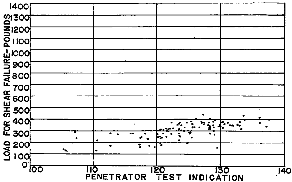
FIG. 44.- RESULTS OF PENETRATOR TESTS USING 3 BALL PENETRATOR ADJUSTED FOR .040" 24ST SHEET ON:
