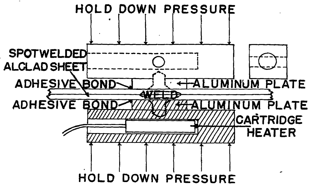
A. BONDING LOADING DISC TO SHEET
