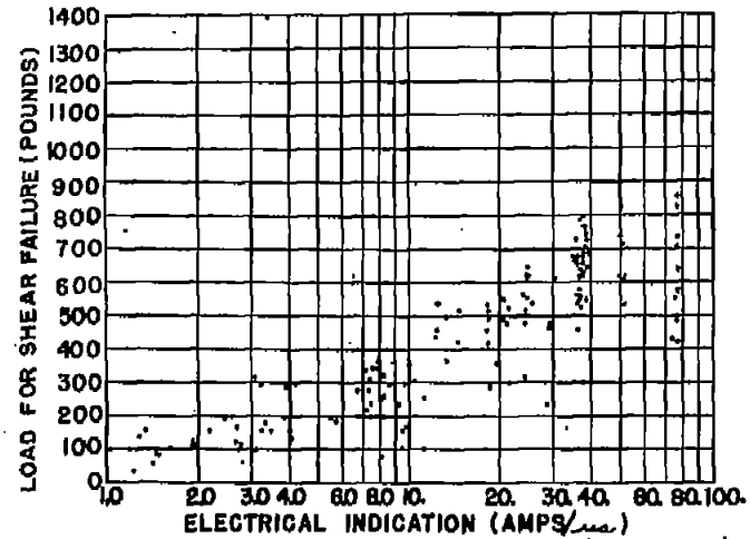
A. 181 WELDS IN .040" 24ST ALCLAD MADE ON FEDERAL WELDER AT RYAN AERONAUTICAL CORPORATION, SAN DIEGO, CALIFORNIA.
