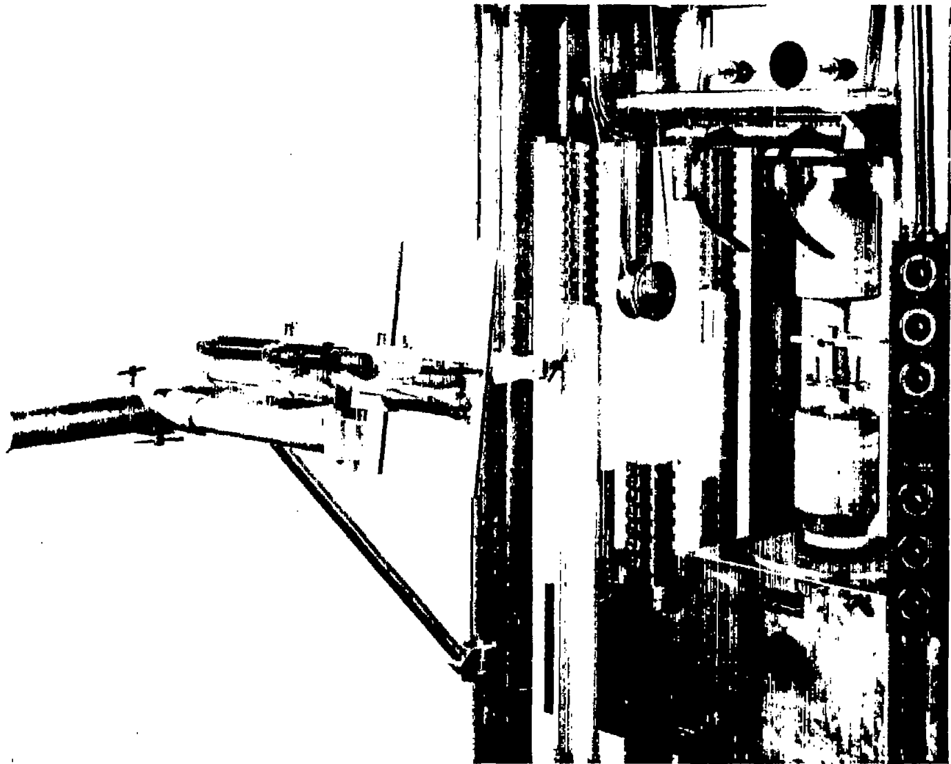
Figure 2.- Martens mirror apparatus and special tension grips as used in determining modulus of elasticity of aluminum alloys.
