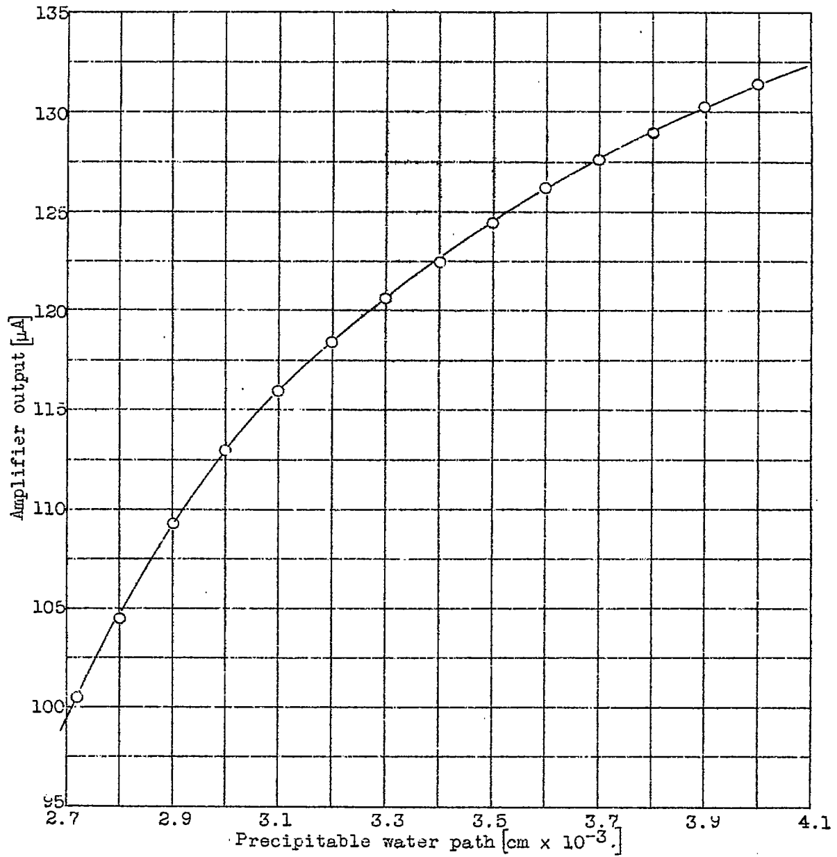
Figure 5.- Calibration curve.
