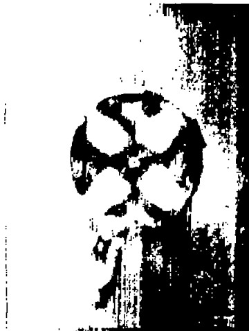
Figure 2.—Etch pattern on copper crystal heated in stearic acid at 200° in air for 24 hours. Normal at (100) pole.
