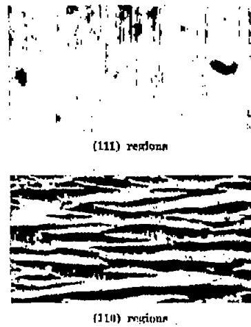
Figure 3.—Photomicrograph of copper crystal etched by stearic acid in air at 200° for 24 hours. Magnification 600.
