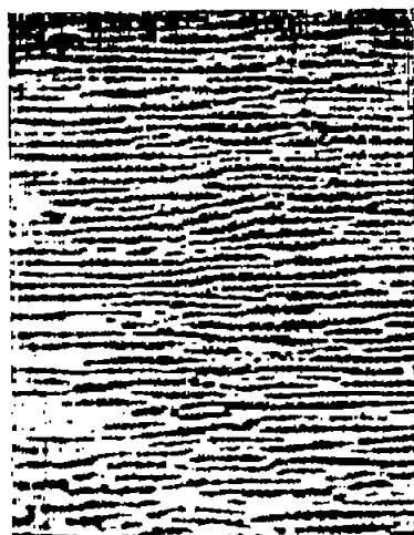
Figure 13.—At (110). Magnification 600. Ridges run perpendicular to line between (100)s.
