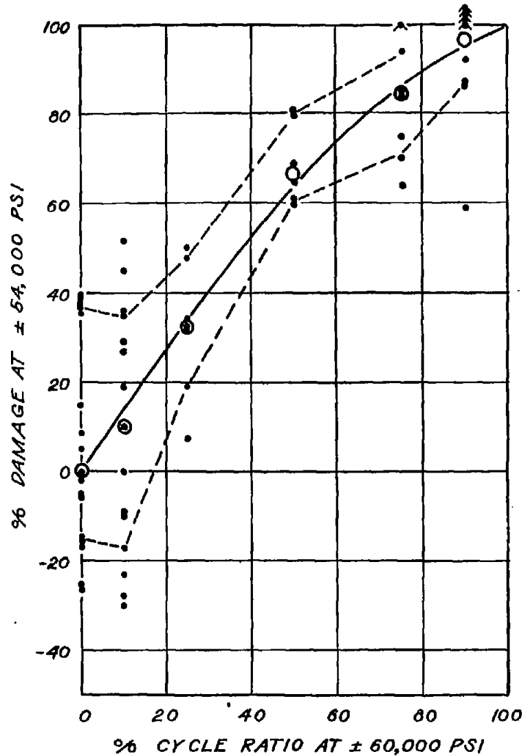
Figure 14.- Change in endurance at ± 54,000 psi after prestressing at ± 60,000 psi. Notched R. R. Moore specimens.
