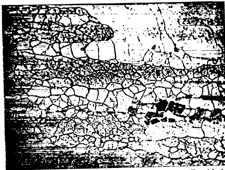
FIGURE 5.—Veining in a section of 25ST aluminum alloy propeller blade. Etchant: 2\frac{1}{2}\% HNO 3 , 1\frac{1}{2}\% HCl, 1% HF. \times 500 .
