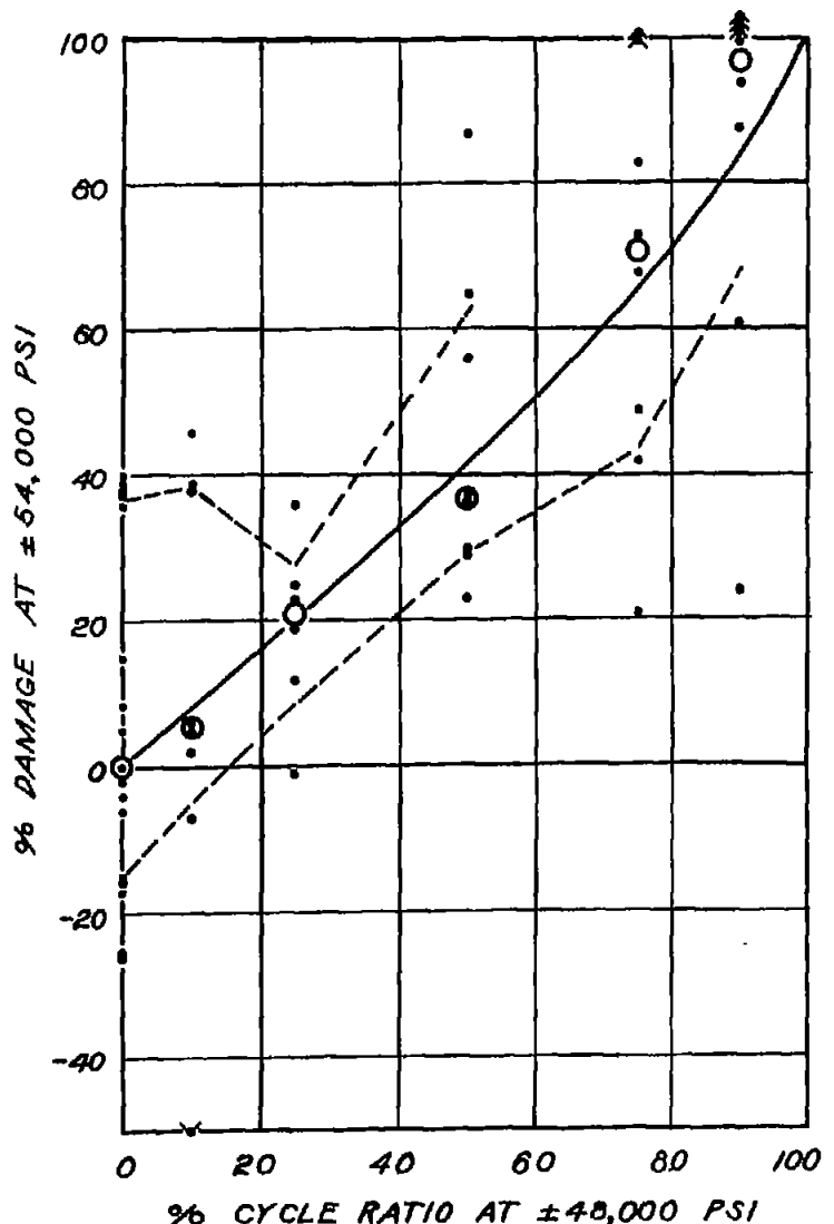
Figure 13.- Change in endurance at ± 54,000 psi after prestressing at ± 48,000 psi. Notched R. R. Moore specimens.
