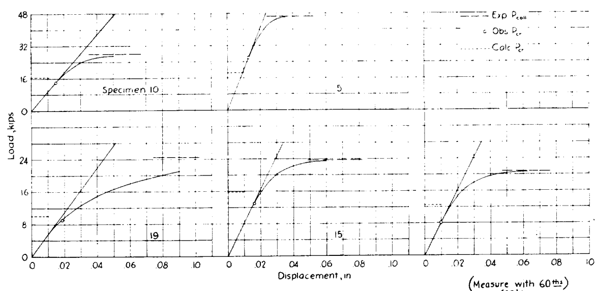
Figure 5.- Load-displacement curves for perforated webs.
