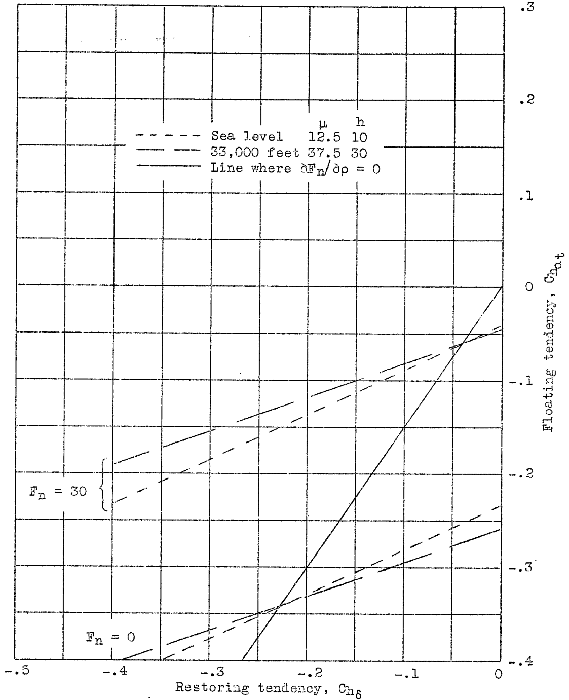
Figure 5.- Effect of altitude on values of stick-force gradient. x_{a.c.} = 0.05c ; W/S_w = 40 pounds per square foot; c = 7 feet.
