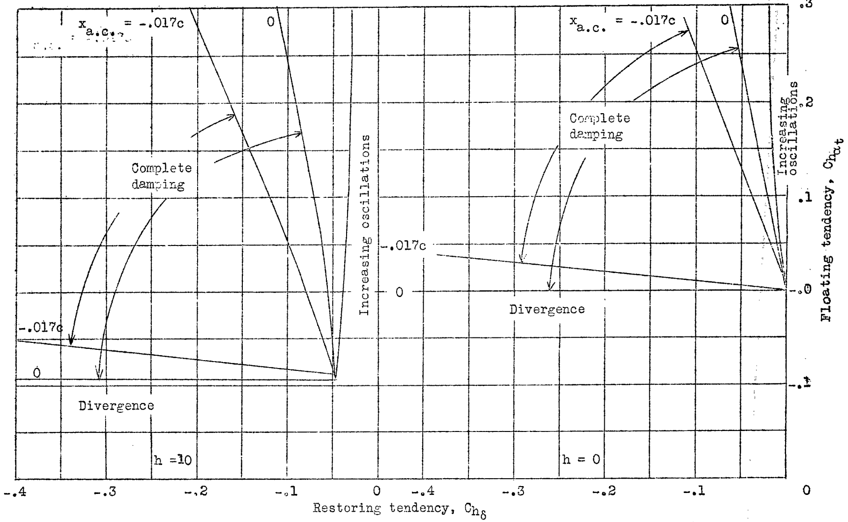
Figure 18.- Boundaries for complete damping, increasing oscillations, and divergence. \mu = 37.5 .
