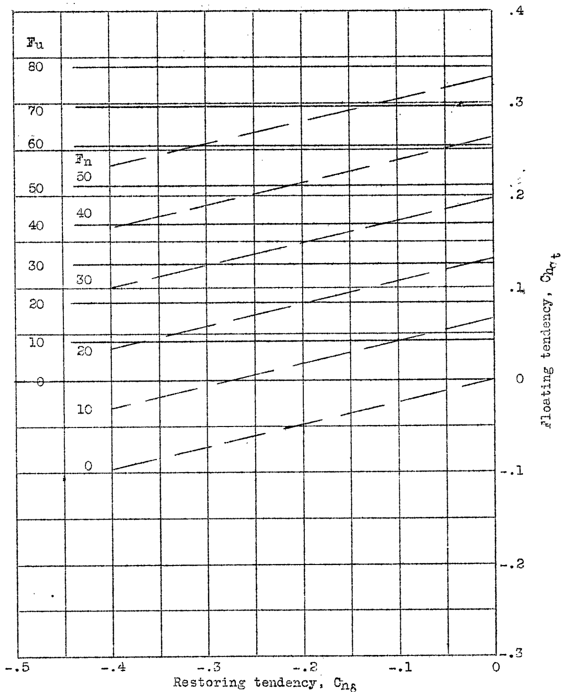
Figure 2.- Trim force F_u and pull-up force F_n as a function of hinge-moment parameters. x_{a.c.} = 0 ; W/S_w = 40 pounds per square foot; c = 7 feet; sea level. F_u = stick force in pounds for \Delta V/V = 1.0 ; F_n = stick force in pounds per g normal acceleration.
