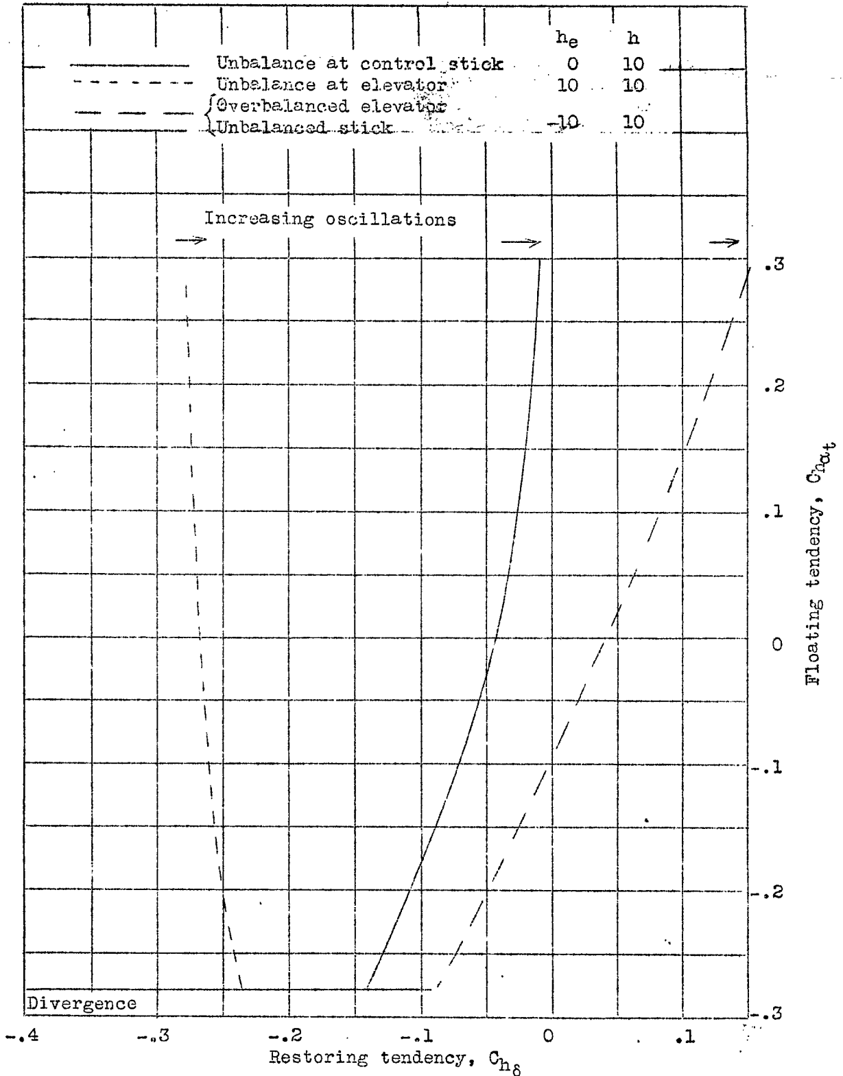
Figure 12.- Effect of location of mass unbalance of the elevator control system on the stability boundaries. \mu = 12.5 ; i_e = 0 ; i_s = 0 .
