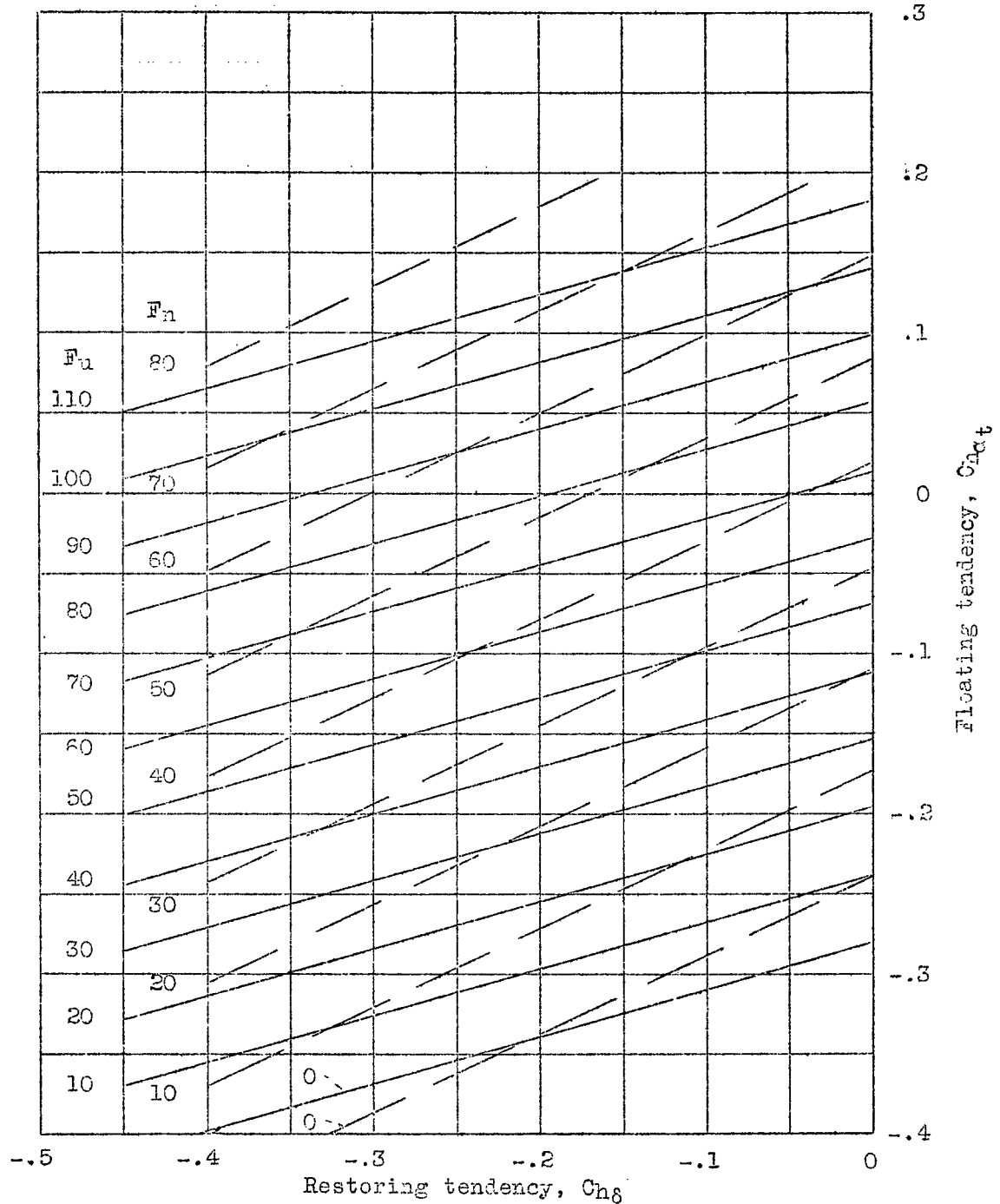
Figure 4.- Trim force F_u and pull-up force F_n as a function of hinge-moment parameters. Mass-unbalanced elevator ( h = 10 ); \alpha_{a.c.} = 0.05c ; W/S_w = 40 pounds per square foot; c = 7 feet; sea level. F_u = stick force in pounds for \Delta V/V = 1.0 ; F_n = stick force in pounds per g normal acceleration.
