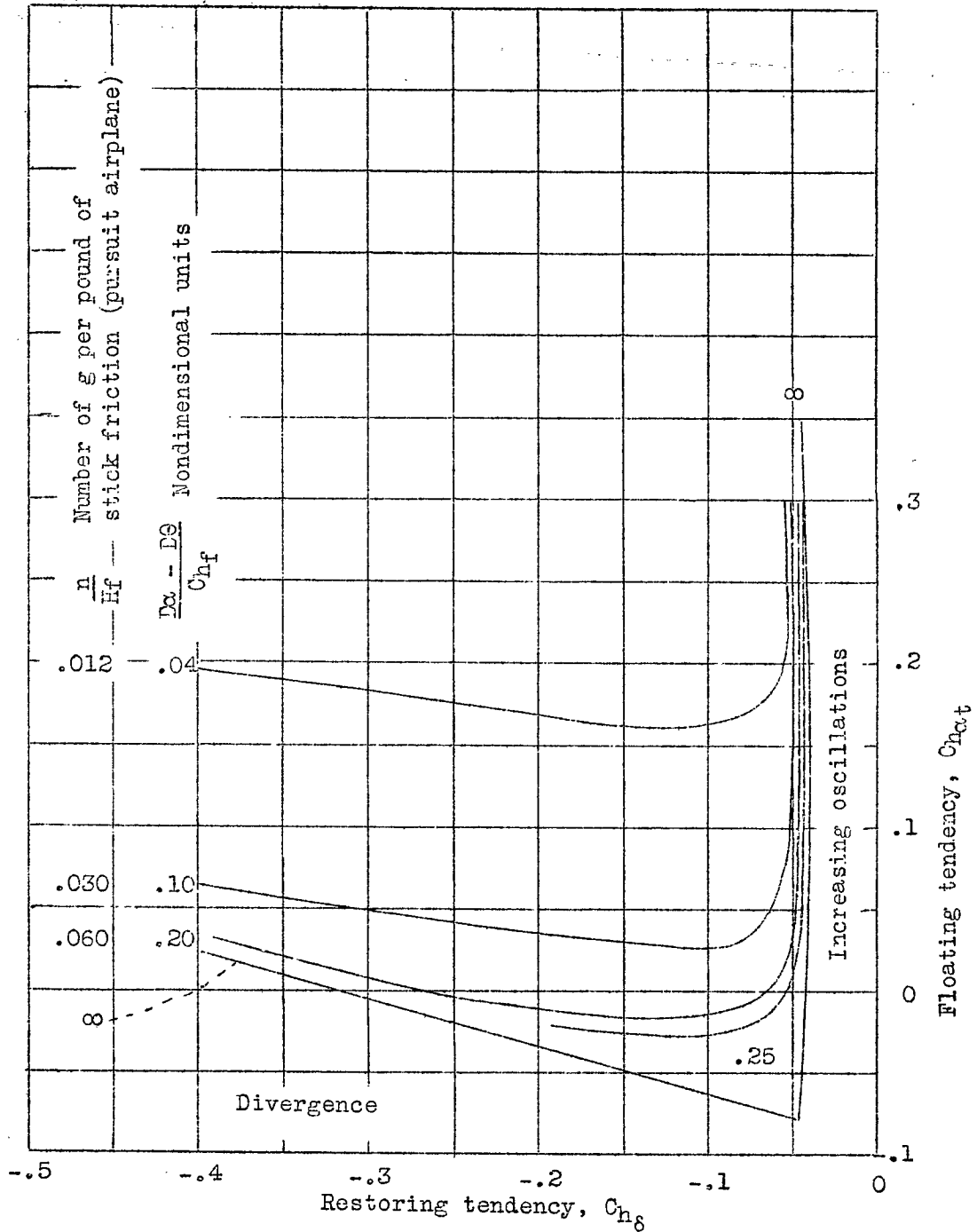
Figure 20.- Variation of maximum normal acceleration in the steady oscillation with elevator hinge-moment parameters. x_{a.c.} = -0.05c ; \mu = 37.5 ; h = 10 ; i_e = 2 ; i_s = 0 .
