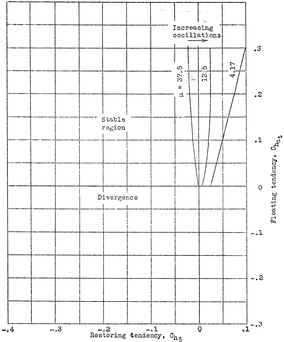
Figure 10.- Variation of stability boundaries with density parameter.
