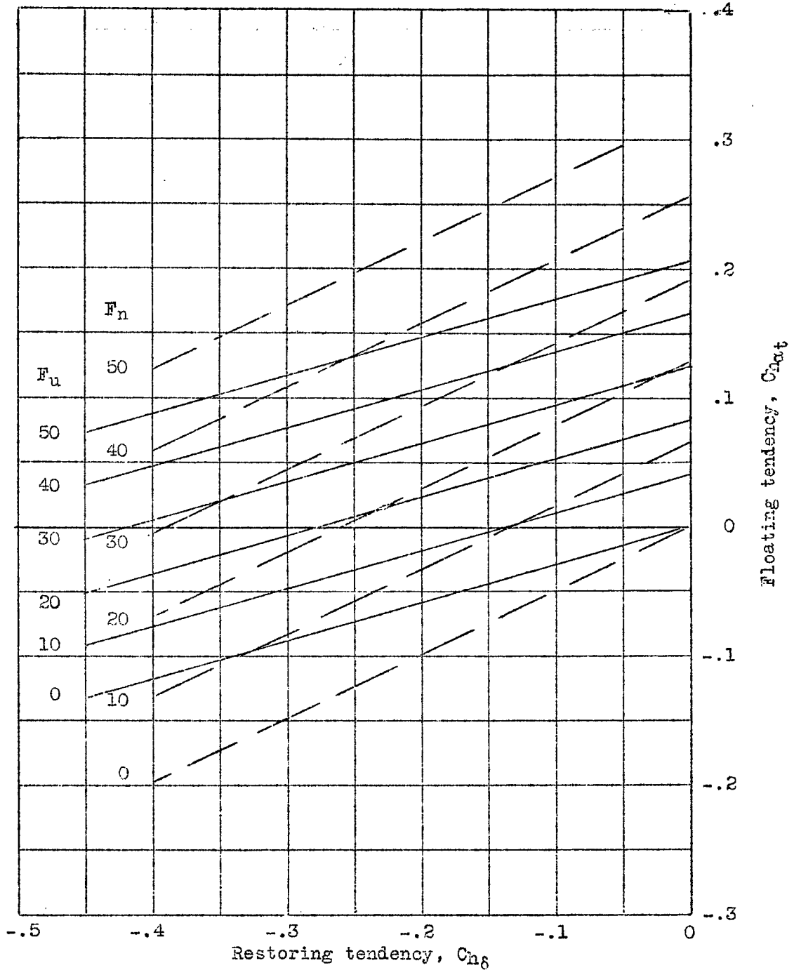
Figure 1.- Trim force F_u and pull-up force F_n as a function of hinge-moment parameters. x_{a.c.} = 0.05c ; W/S_w = 40 pounds per square foot; c = 7 feet; sea level. F_u = stick force in pounds for \Delta V/V = 1.0 ; F_n = stick force in pounds per g normal acceleration.
