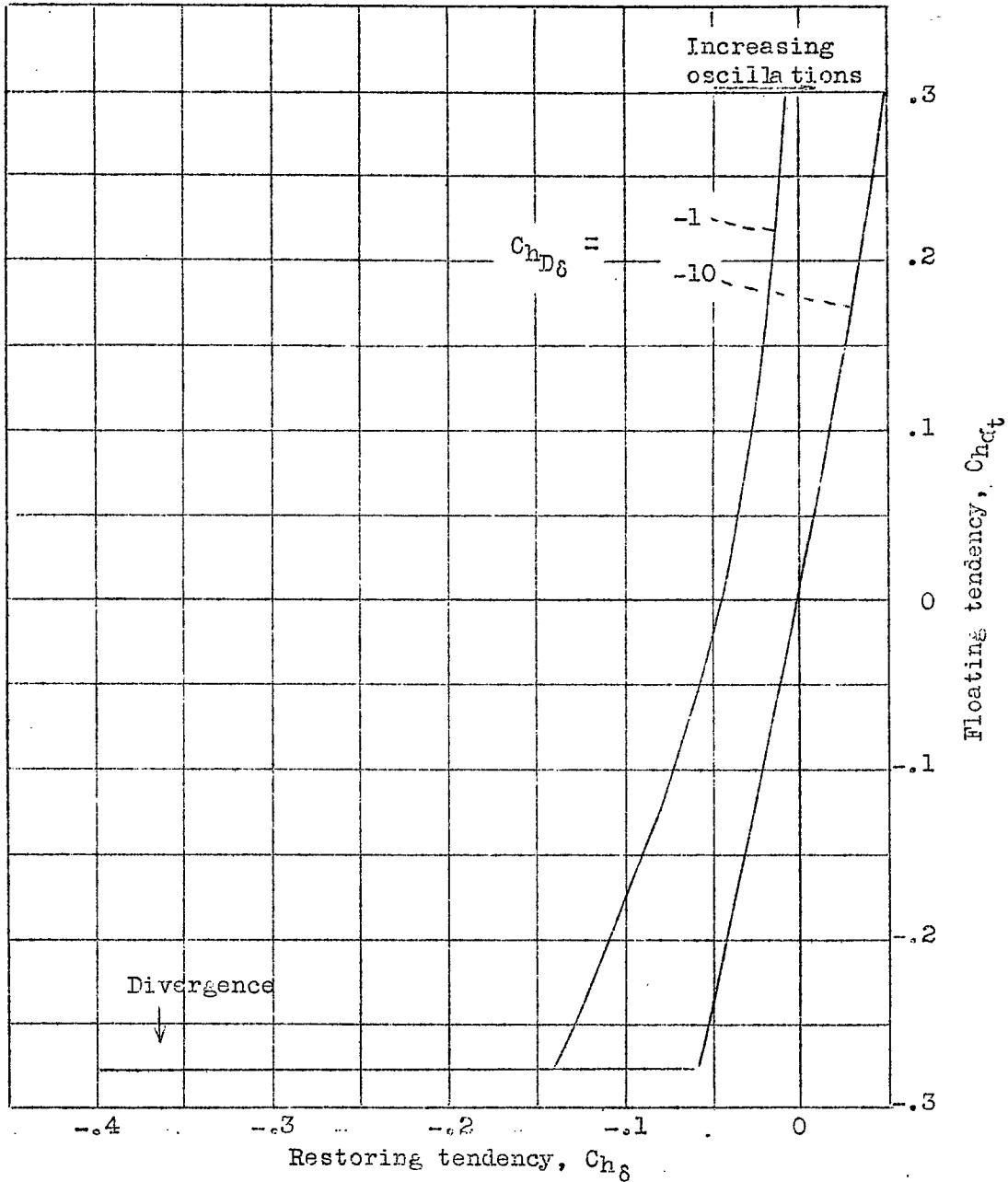
Figure 15.- Illustration of stabilizing effect of elevator damping (viscous friction). x_{a.c.} = 0 ; \mu = 12.5 ; h = 10 .
