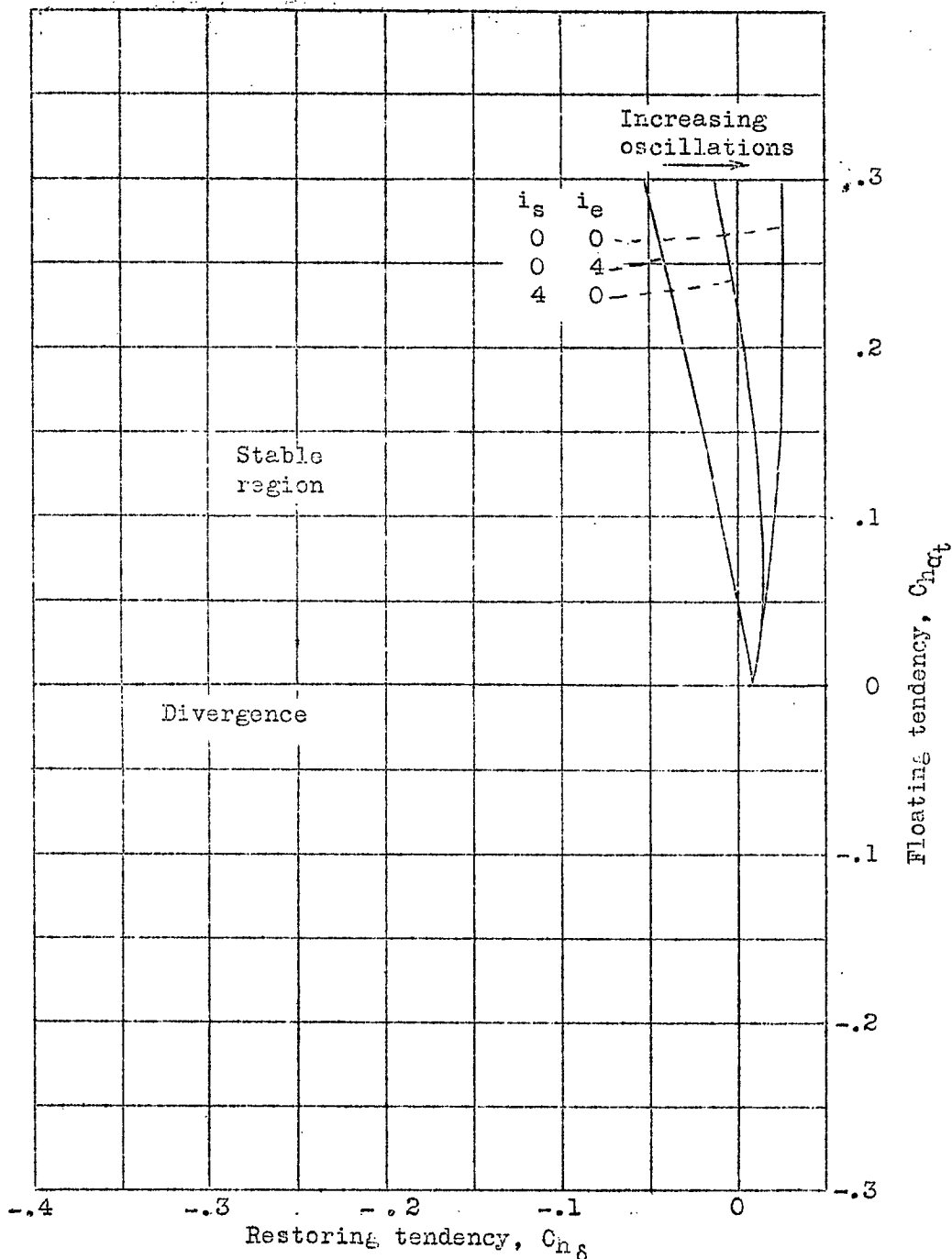
Figure 9.- Effect of elevator-control-system moment of inertia on the boundary for increasing oscillations. \mu = 12.5 .
