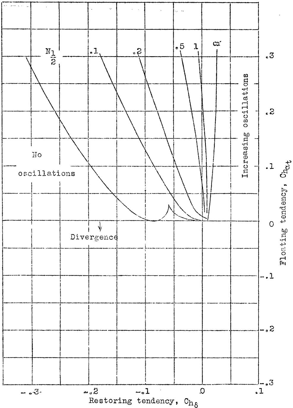
Figure 7.- Number of cycles to damp to half amplitude N_{\frac{1}{2}} against hinge-moment parameters. x_{a.c.} = 0 ; \mu = 12.5 ; h = i = 0 .
