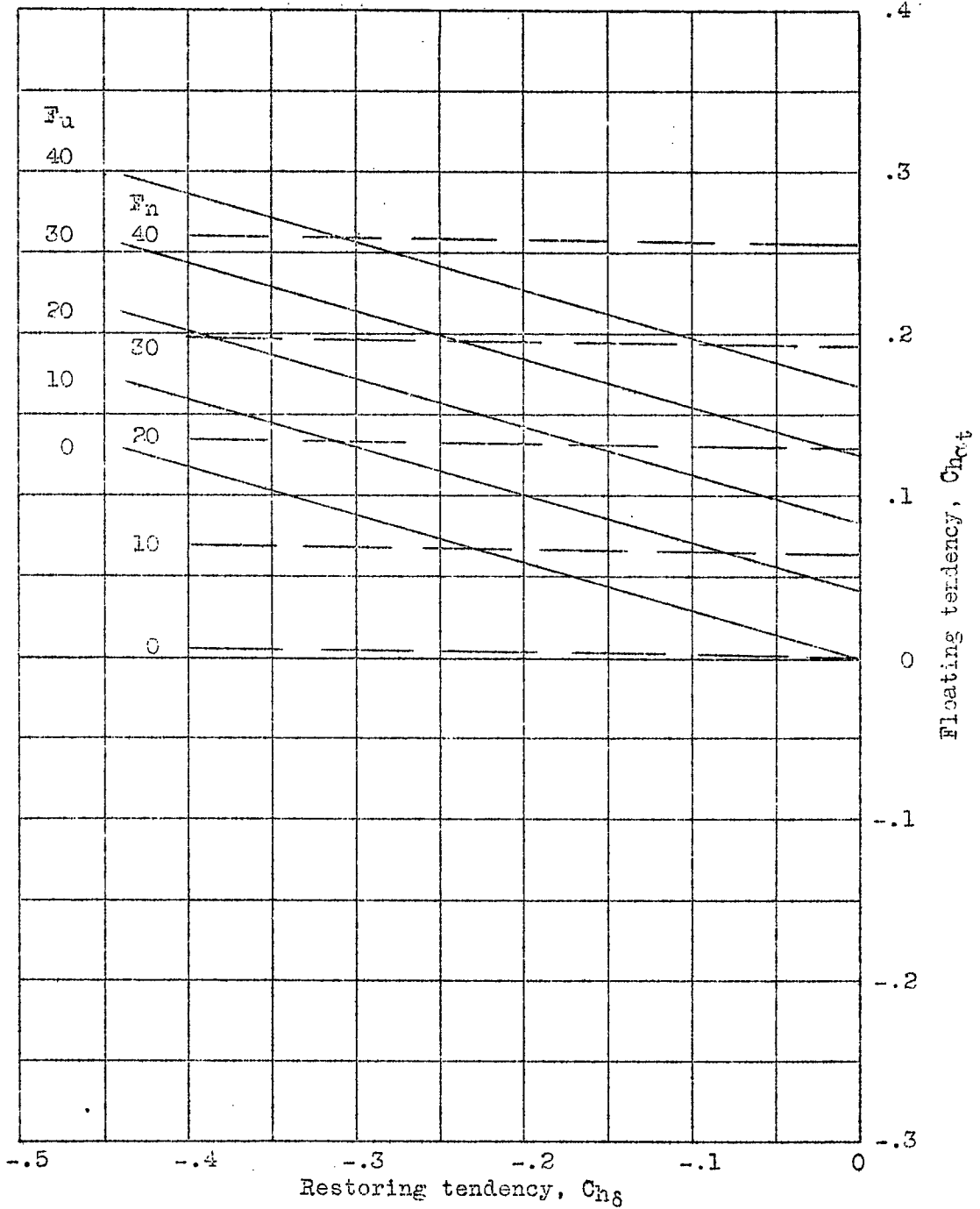
Figure 3.- Trim force F_u and pull-up force F_n as a function of hinge-moment parameters. x_{a.c.} = -0.05c ; W/S_w = 40 pounds per square foot; c = 7 feet; sea level. F_u = stick force in pounds for \Delta V/V = 1.0 ; F_n = stick force in pounds per g normal acceleration.
