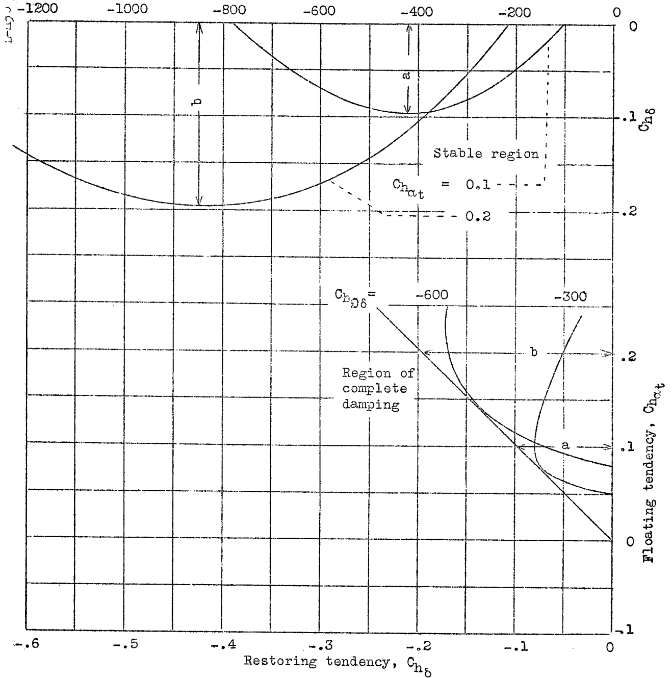
Figure 17.- Method of constructing boundary for complete damping.
