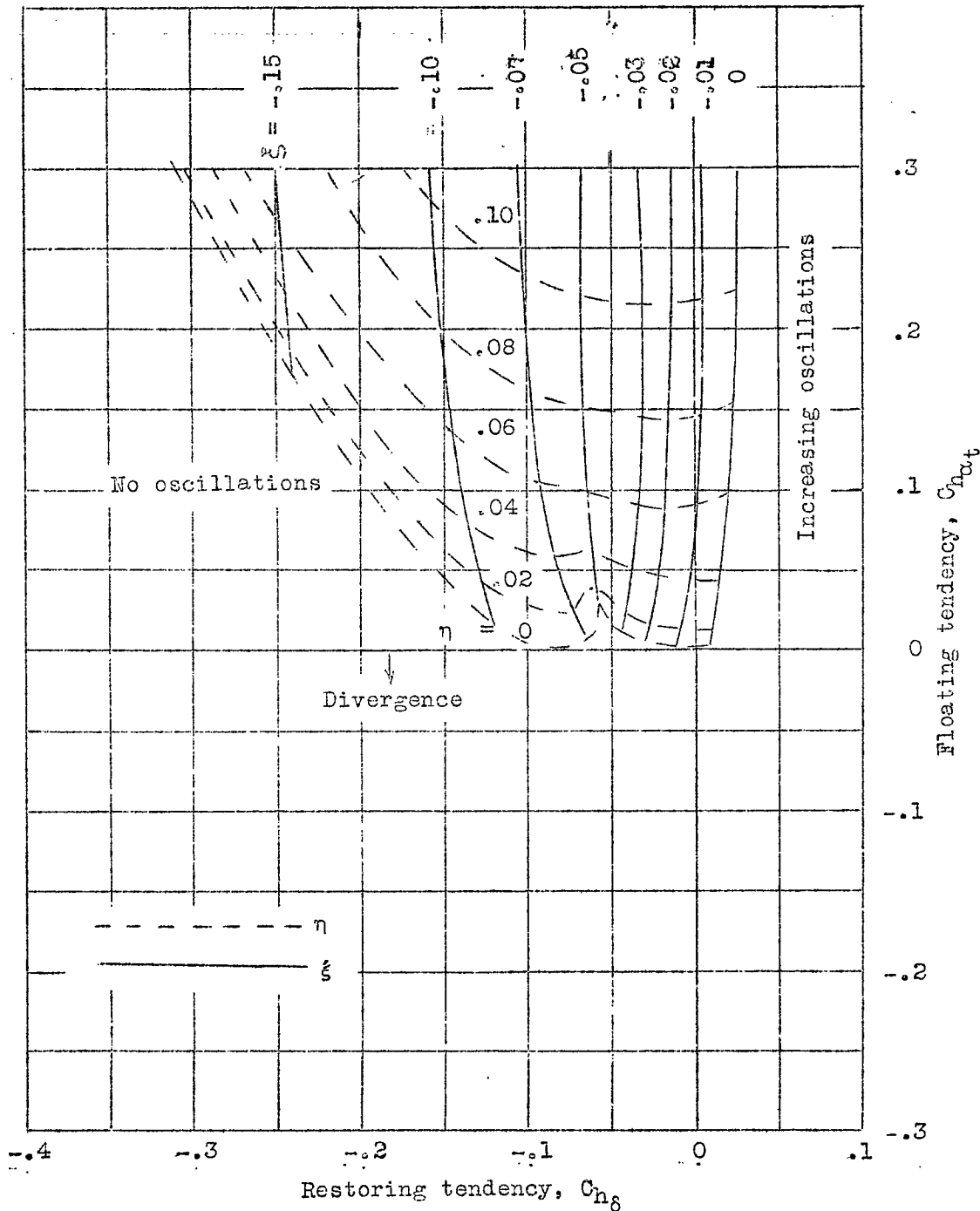
Figure 6.- Variation of damping and frequency of control-free longitudinal oscillation with elevator-balance parameters. x_{a.c.} = 0 ; \mu = 12.5 ; h = \dot{i} = 0 .
