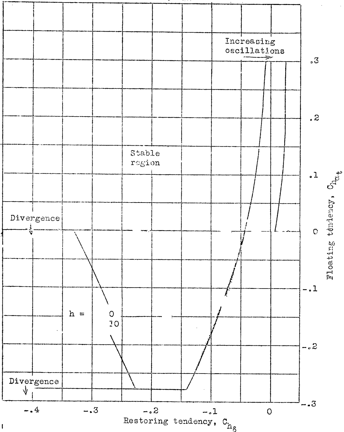
Figure 11.- Effect of mass unbalance of the elevator control system on the stability boundaries. \mu = 12.5 .
