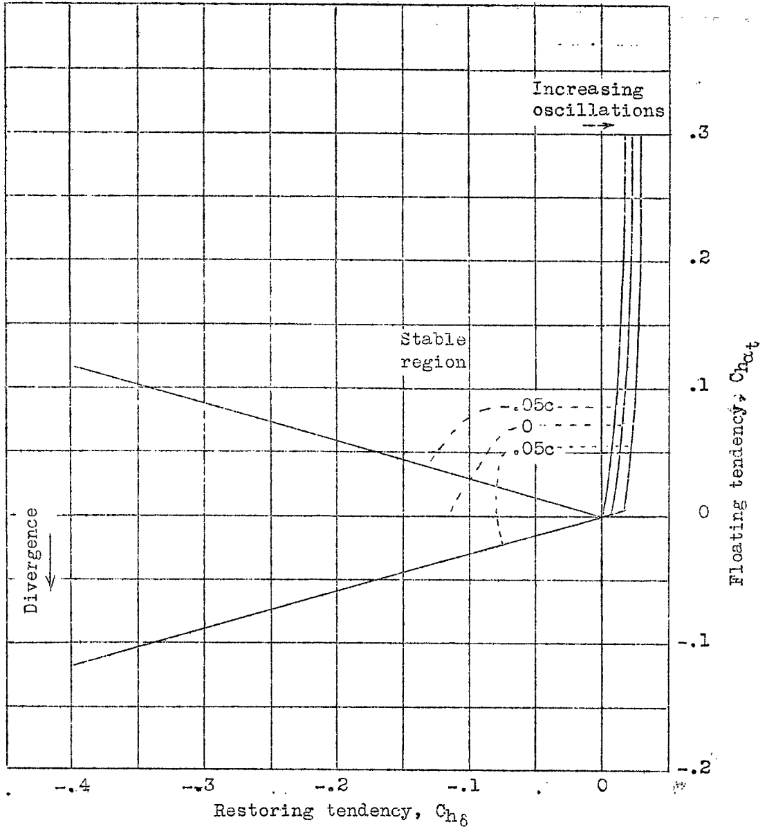
Figure 8.- Effect of center-of-gravity location on stability boundaries. \mu = 12.5 .
