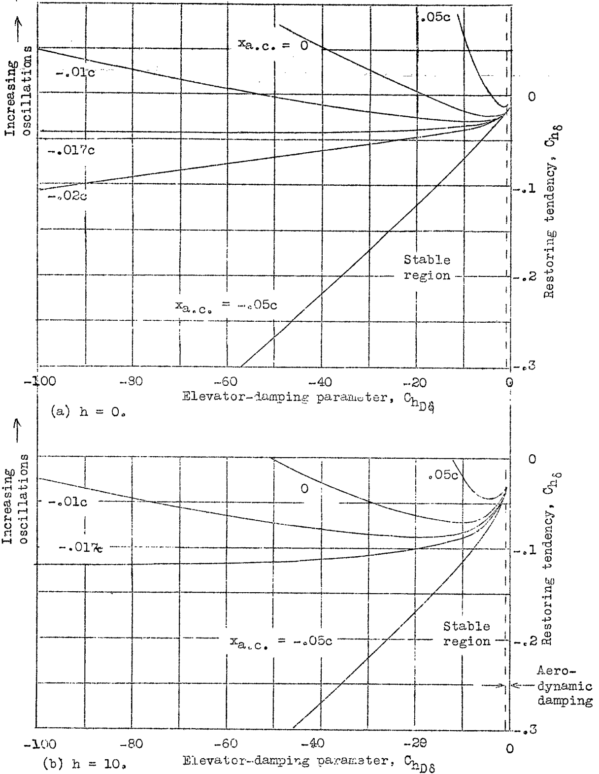
Figure 14.- Effect of elevator damping on the boundary for increasing oscillations for various center-of-gravity locations and elevator-mass-balance conditions. Ch_{\alpha t} = 0.1 ; \mu = 37.5
