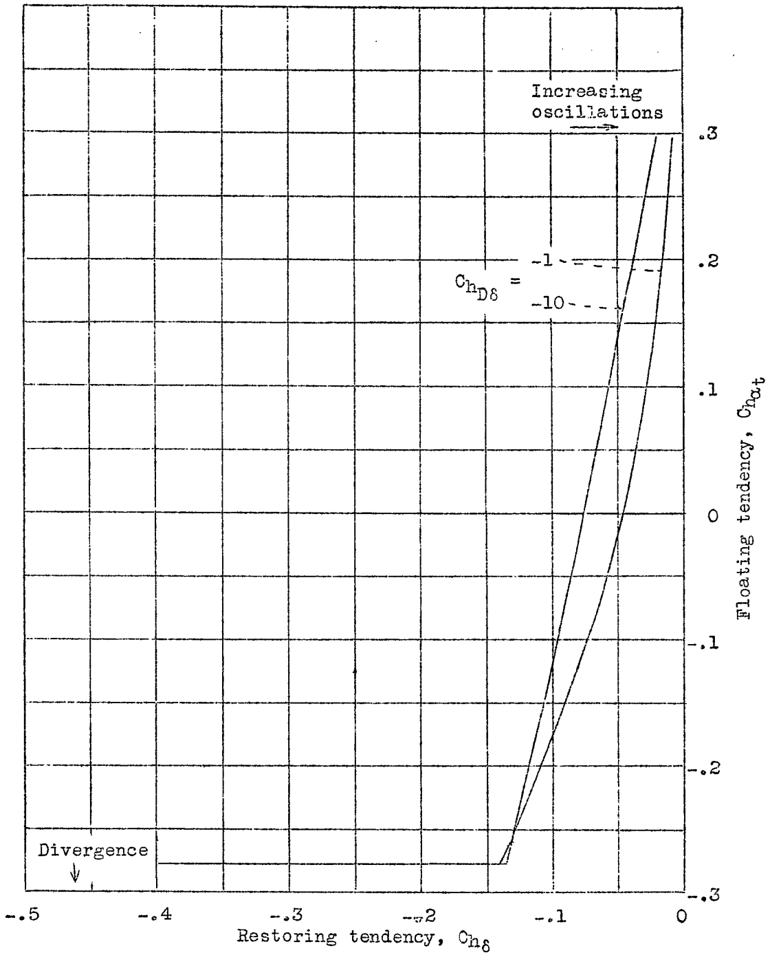
Figure 16.- Illustration of destabilizing effect of elevator damping (viscous friction). x_{a.c.} = -0.05c ; \mu = 12.5 ; h = 10 .
