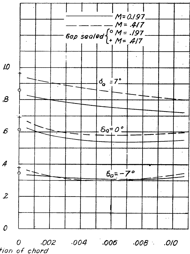
\alpha_o = 0^\circ Figure 16.- Variation of section lift coefficient with gap. Balance nose radii = 0.02c .
