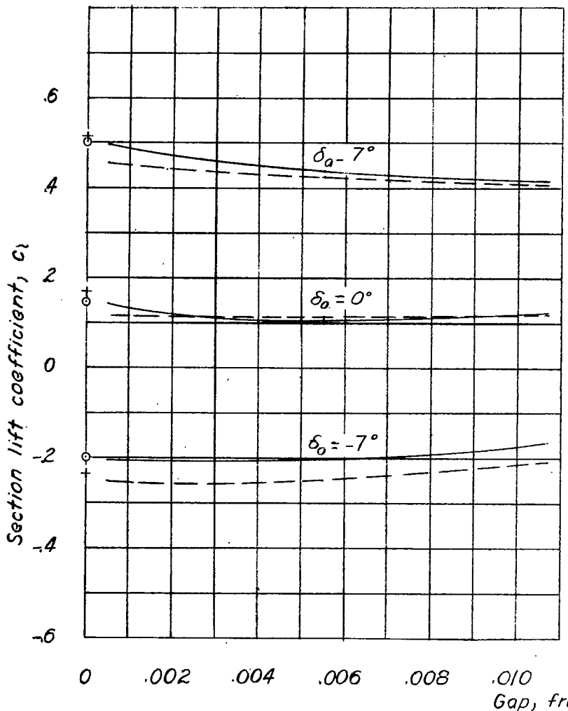
\alpha_o = 0^\circ Figure 16.- Variation of section lift coefficient with gap. Balance nose radii = 0.02c .
