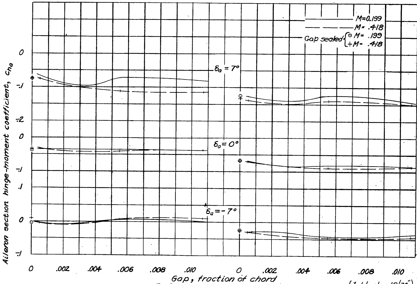
Figure 9.— Variation of aileron section hinge-moment coefficient with gap. \alpha_o = 0^\circ \alpha_o = 5.1^\circ
