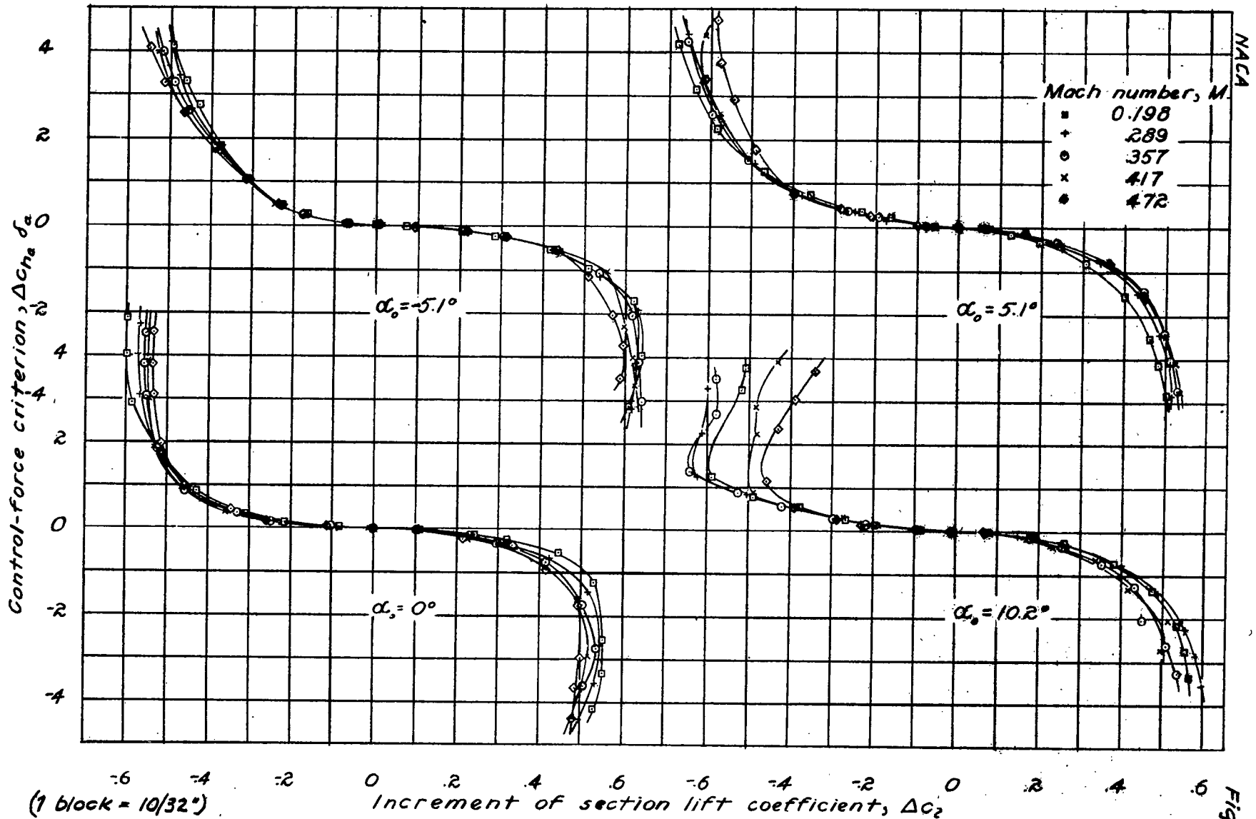
Figure 17: - Variation of control-force criterion with increment of section lift coefficient; showing change with Mach number. Balance nose radii = 0.02c ; gap = 0.0055c .
