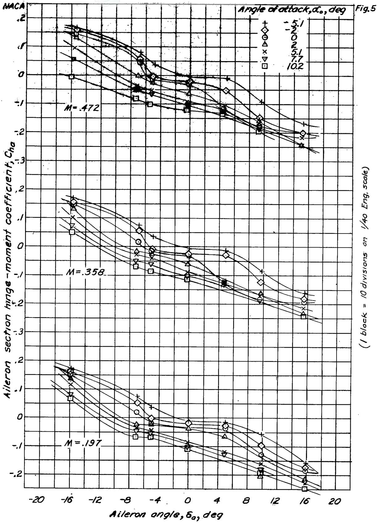
Figure 5.—Variation of aileron section hinge-moment coefficient with aileron angle (by pressure distribution). Balance-nose radii = 0; gap = 0.0055c.
