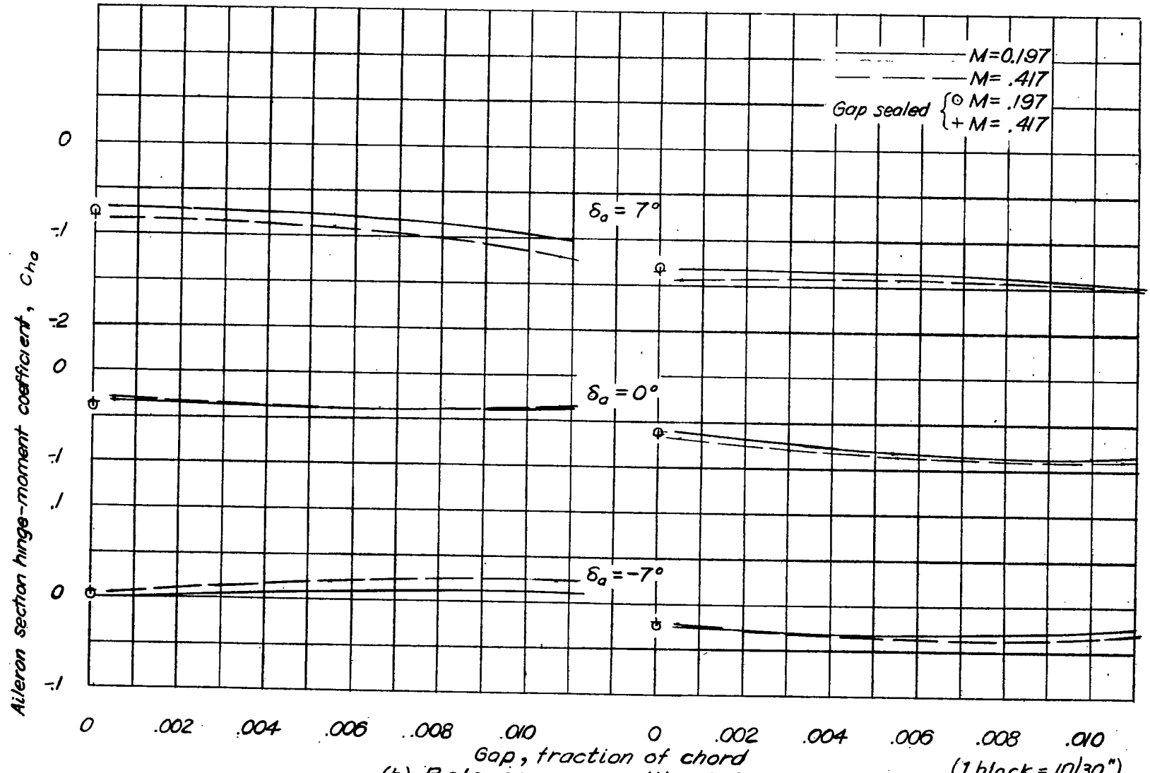
Figure 9.— Variation of aileron section hinge-moment coefficient with gap: (Continued)
