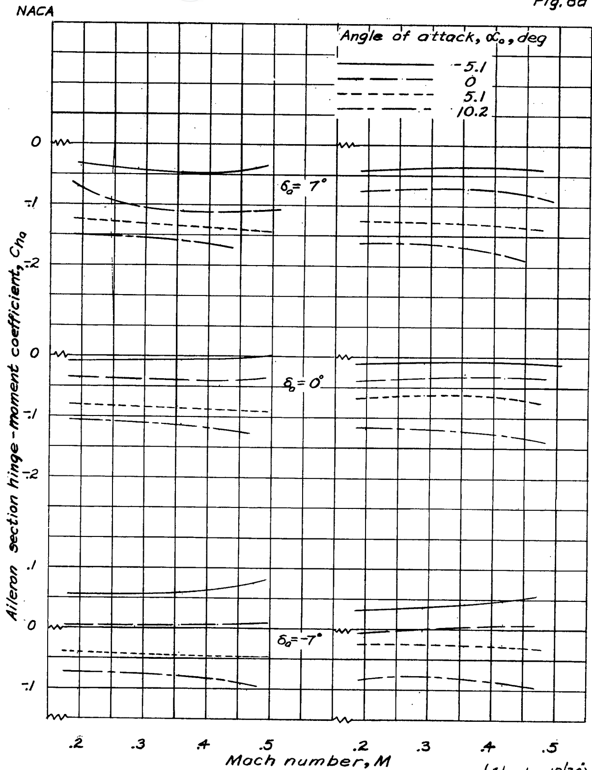
(a) Balance nose radii = 0.01c. Gap = 0.0055c Gap = 0.0055c (sealed)
