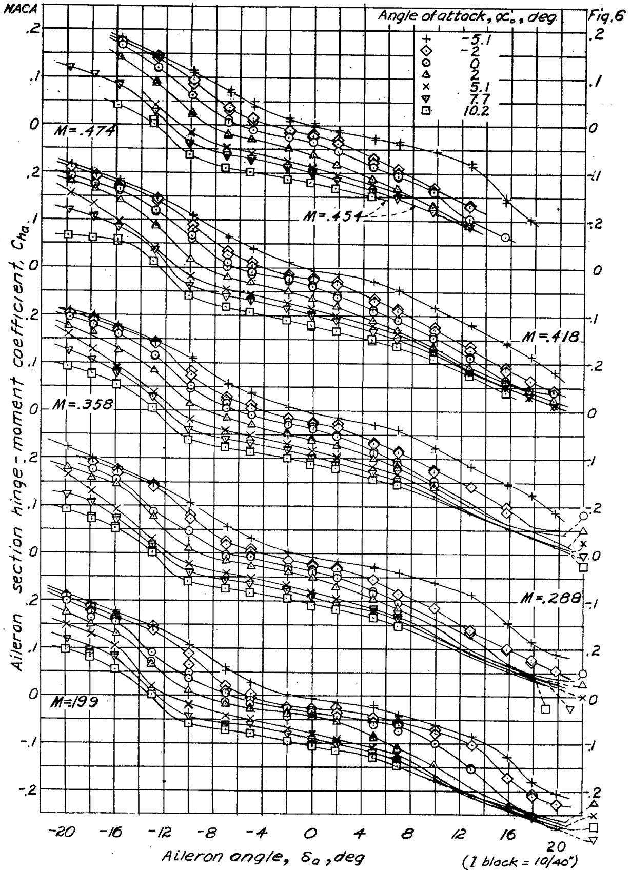
Figure 6.— Variation of aileron section hinge-moment coefficient with aileron angle. Balance-nose radii = 0.01c; gap = 0.0055c.
