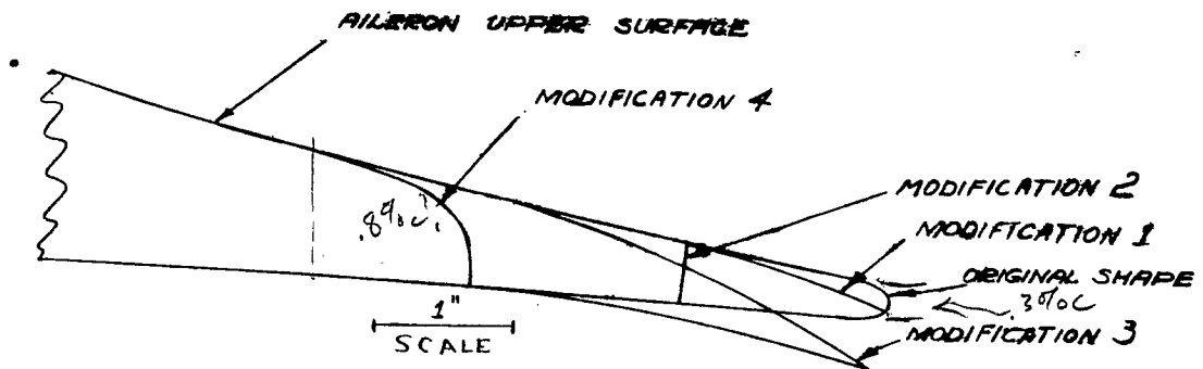
FIGURE 3.—MODIFICATIONS OF TRAILING EDGE OF A 0.20C FRISE-TYPE AILERON ON A 100-INCH CHORD LOW-DRAG MODEL.
