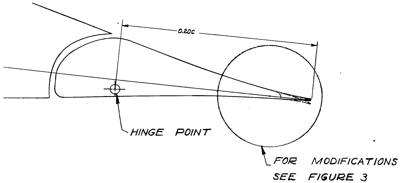
FIGURE 2.—NACA 65,2-417 (APPROX.) TEST MODEL FOR TRAILING-EDGE MODIFICATIONS.
