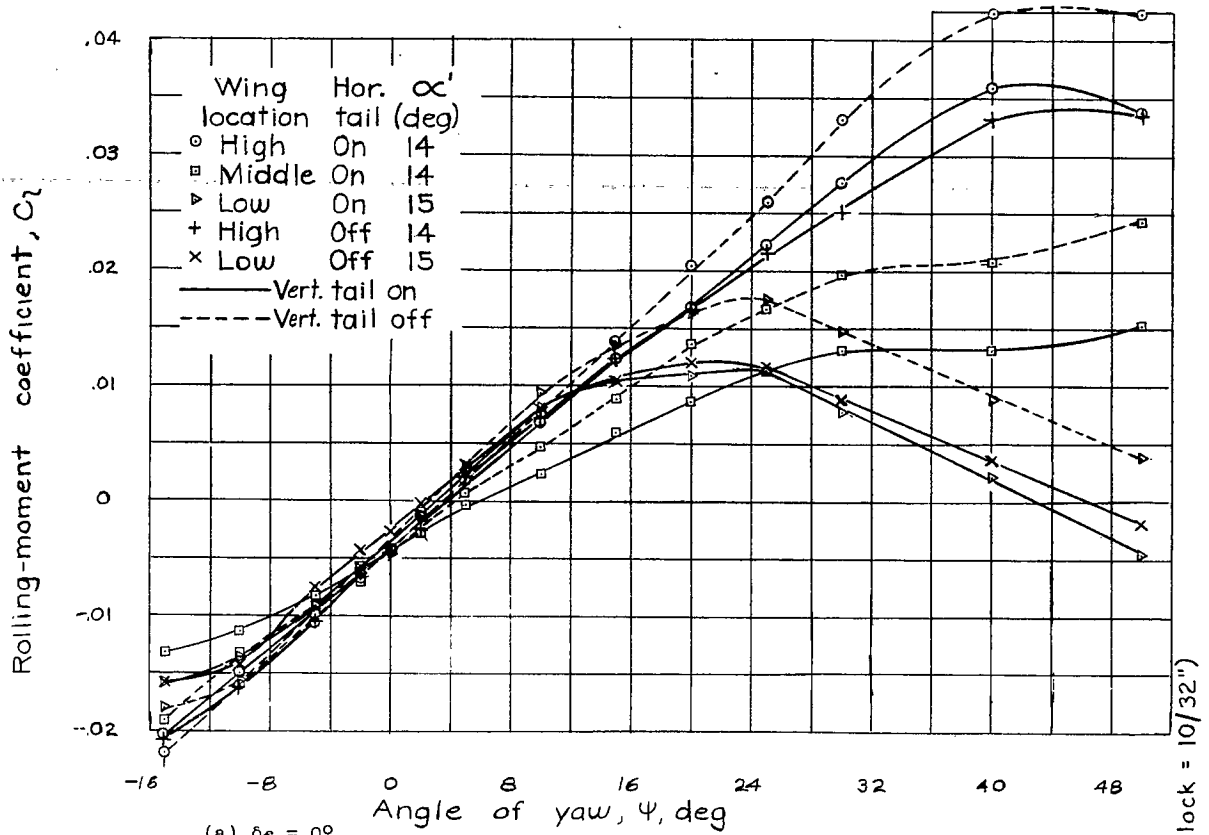
Figure 13.- Variation of rolling-moment coefficient with yaw, NACA 23012 wing with fuselage and horizontal and vertical tails.
