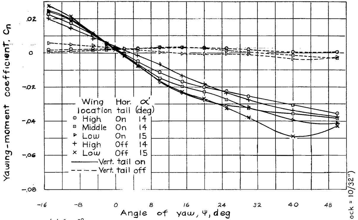
Figure 14.- Variation of yawing-moment coefficient with yaw. NACA 23012 wing with fuselage and horizontal and vertical tails.
