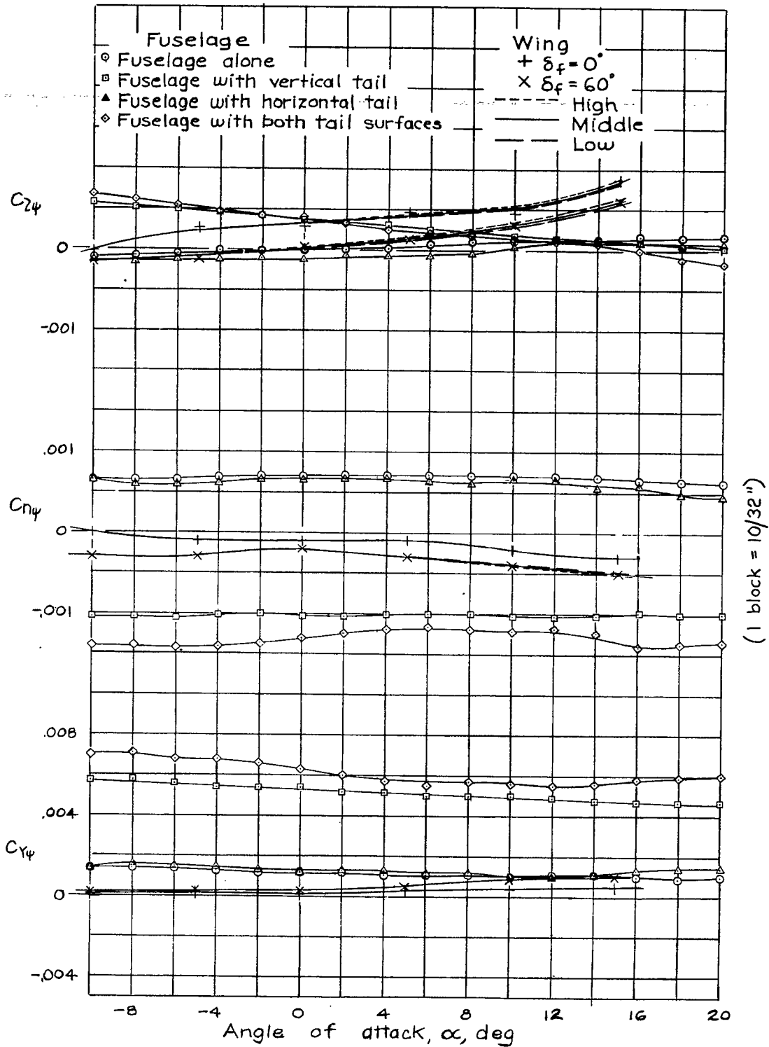
Figure 3.—Variation of C_{2\psi} , C_{n\psi} , and C_{y\psi} with angle of attack.
