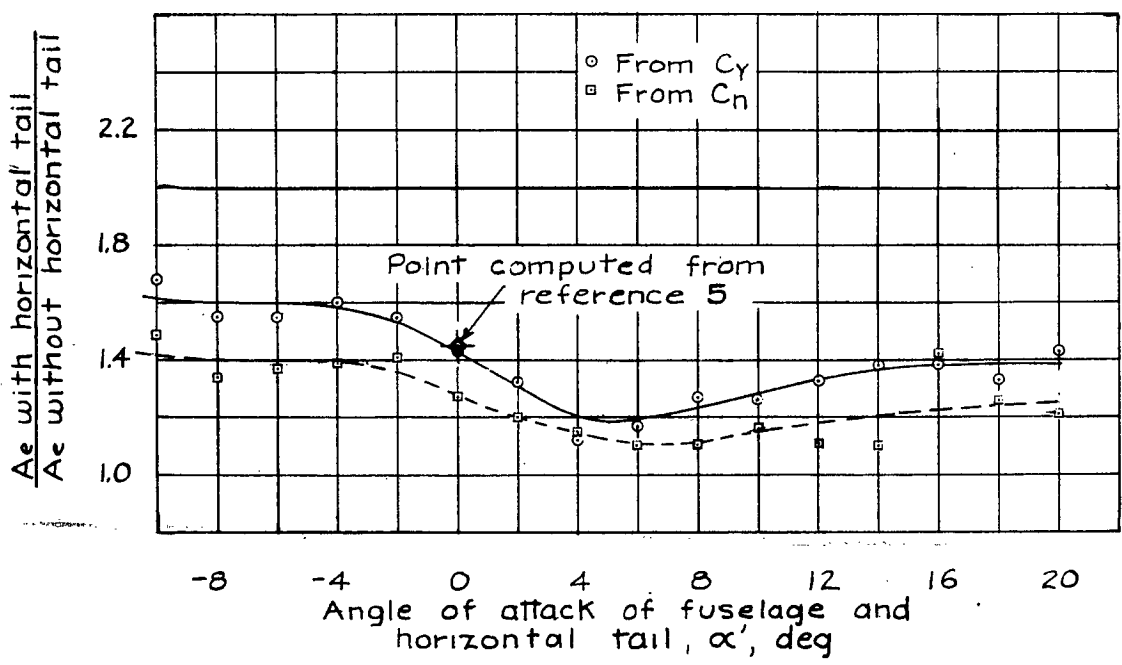
Figure 5.- Ratio of effective aspect ratio of vertical tail on the circular fuselage with horizontal tail to that without horizontal tail.
