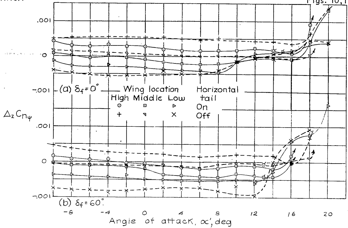
Figure 10.- Effect of wing-fuselage interference on C_{n\psi} due to vertical tail. NACA 23012 wing with fuselage and horizontal and vertical tails. (Data with horizontal tail off from reference 3.)
