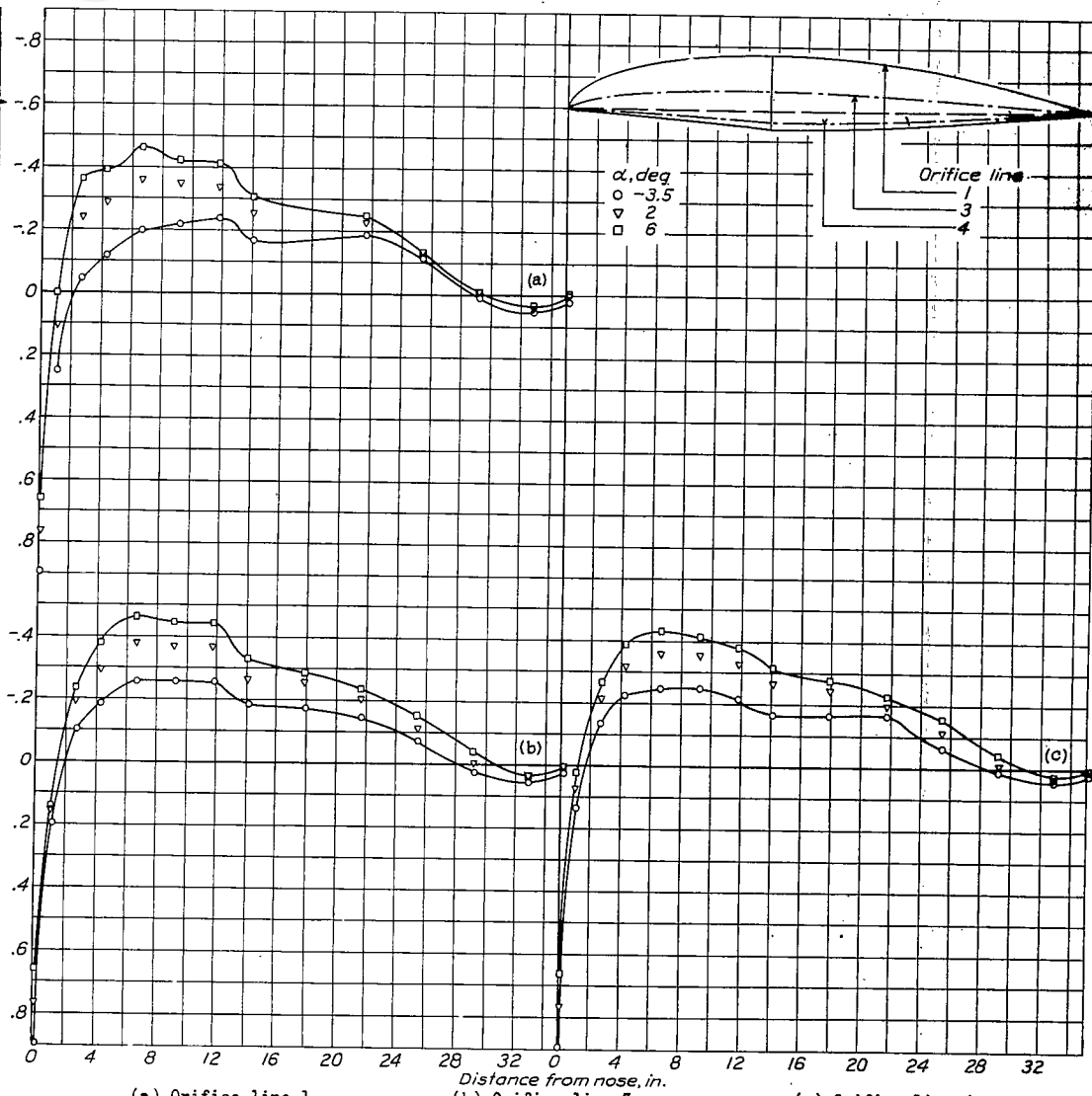
(a) Orifice line 1. (b) Orifice line 3. (c) Orifice line 4 Figure 26.- Pressure distribution about the 4-0-3 windshield for various angles of attack. M, 0.198 .
