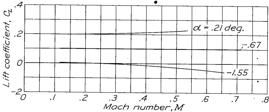
Figure 10.- Variation of model lift coefficient with Mach number.
