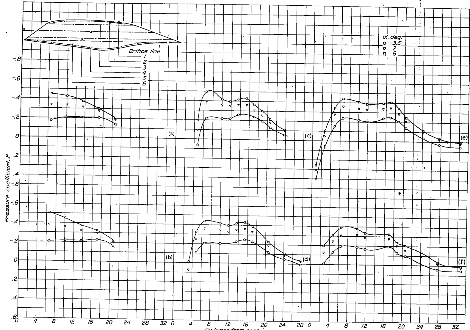
(a) Orifice line 1 (b) Orifice line 2 (c) Orifice line 3 (d) Orifice line 4 (e) Orifice line 5 (f) Orifice line 6 Figure 32.- Pressure distribution about the X-2 windshield for various angles of attack. M, 0.192 .
