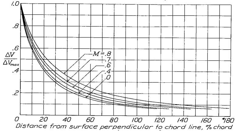
Figure 35.- Theoretical velocity contours for the NACA 2215 wing section. \alpha, -0.67^\circ .
