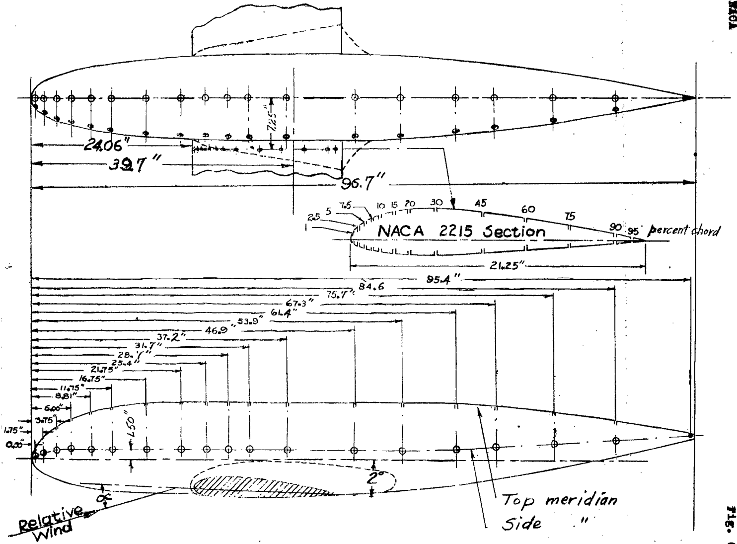
Figure 6. - Pressure-orifice locations on wing and fuselage
