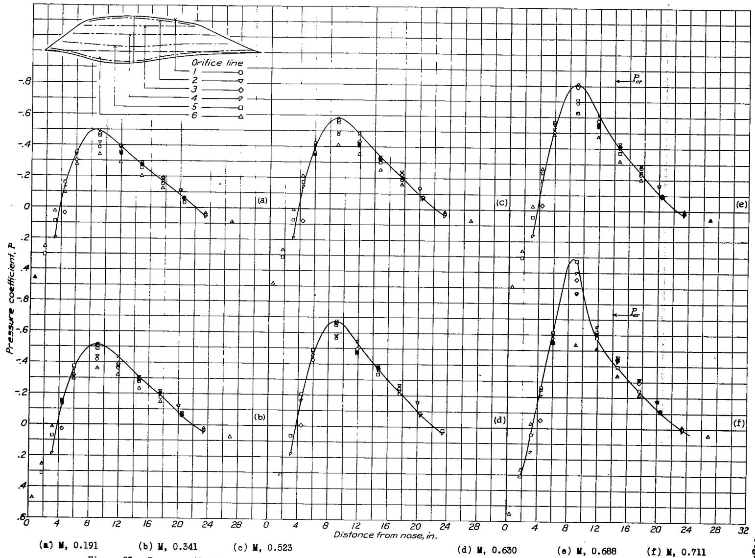
Figure 23.- Pressure distribution about the X-1 windshield for various Mach numbers. \alpha , -0.67^\circ .
