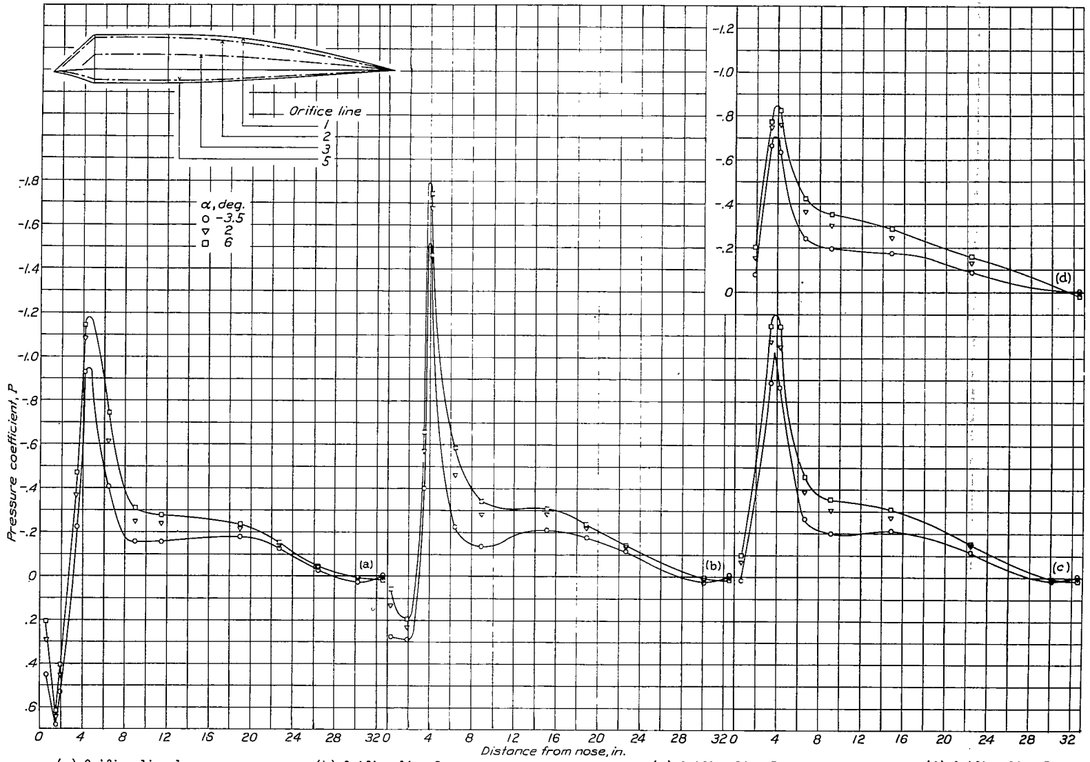
Figure 30.- Pressure distribution about the 8-4-5 windshield for various angles of attack. M, 0.192.
