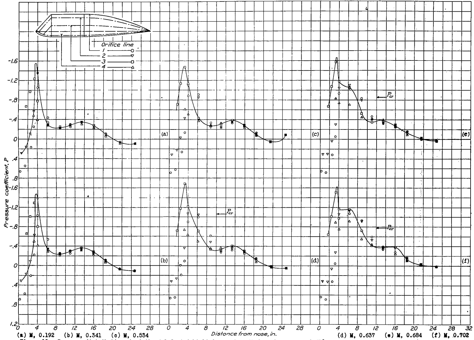
(a) M, 0.192 (b) M, 0.341 (c) M, 0.534 (d) M, 0.637 (e) M, 0.684 (f) M, 0.702 Figure 18.- Pressure distribution about the 6-1-2 windshield for various Mach numbers. \alpha , -0.67^\circ .
