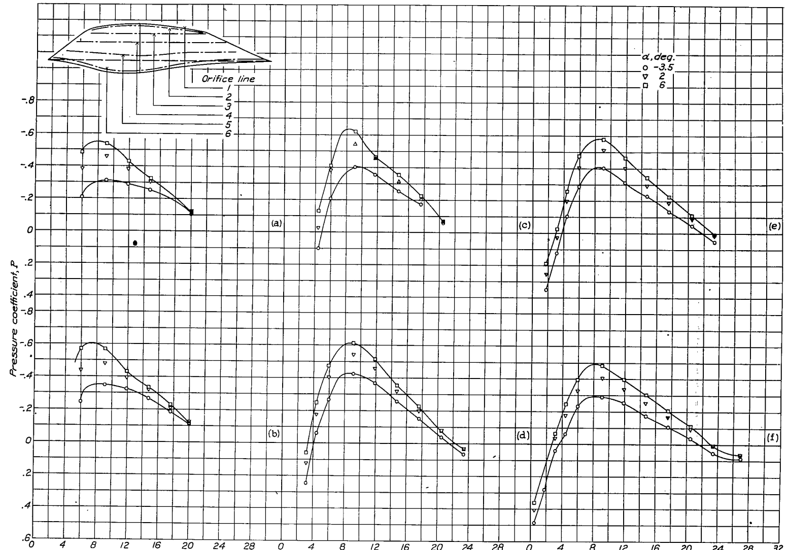
(a) Orifice line 1 (b) Orifice line 2 (c) Orifice line 3 (d) Orifice line 4 (e) Orifice line 5 (f) Orifice line 6 Figure 31.- Pressure distribution about the X-1 windshield for various angles of attack. M , 0.190.
