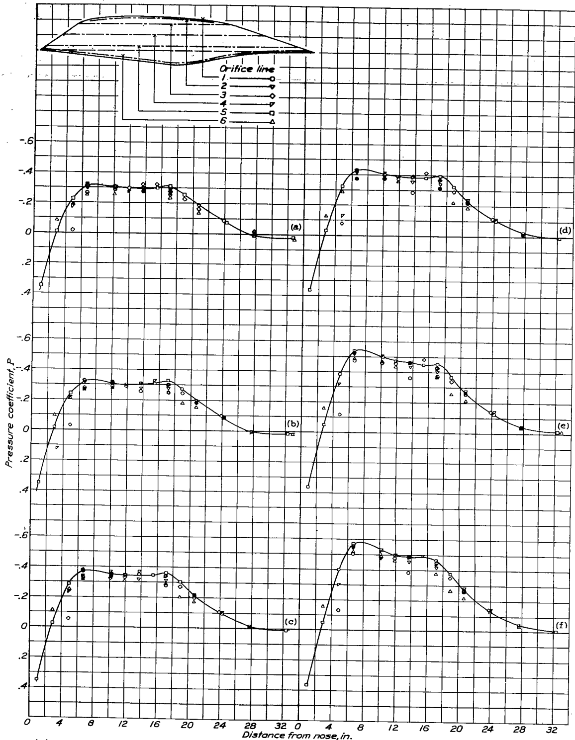
(a) M, 0.194 (b) M, 0.330 (c) M, 0.524 (d) M, 0.623 (e) M, 0.684 (f) M, 0.700 Figure 24.- Pressure distribution about the X-2 windshield for various Mach numbers. \alpha , -0.67^\circ .
