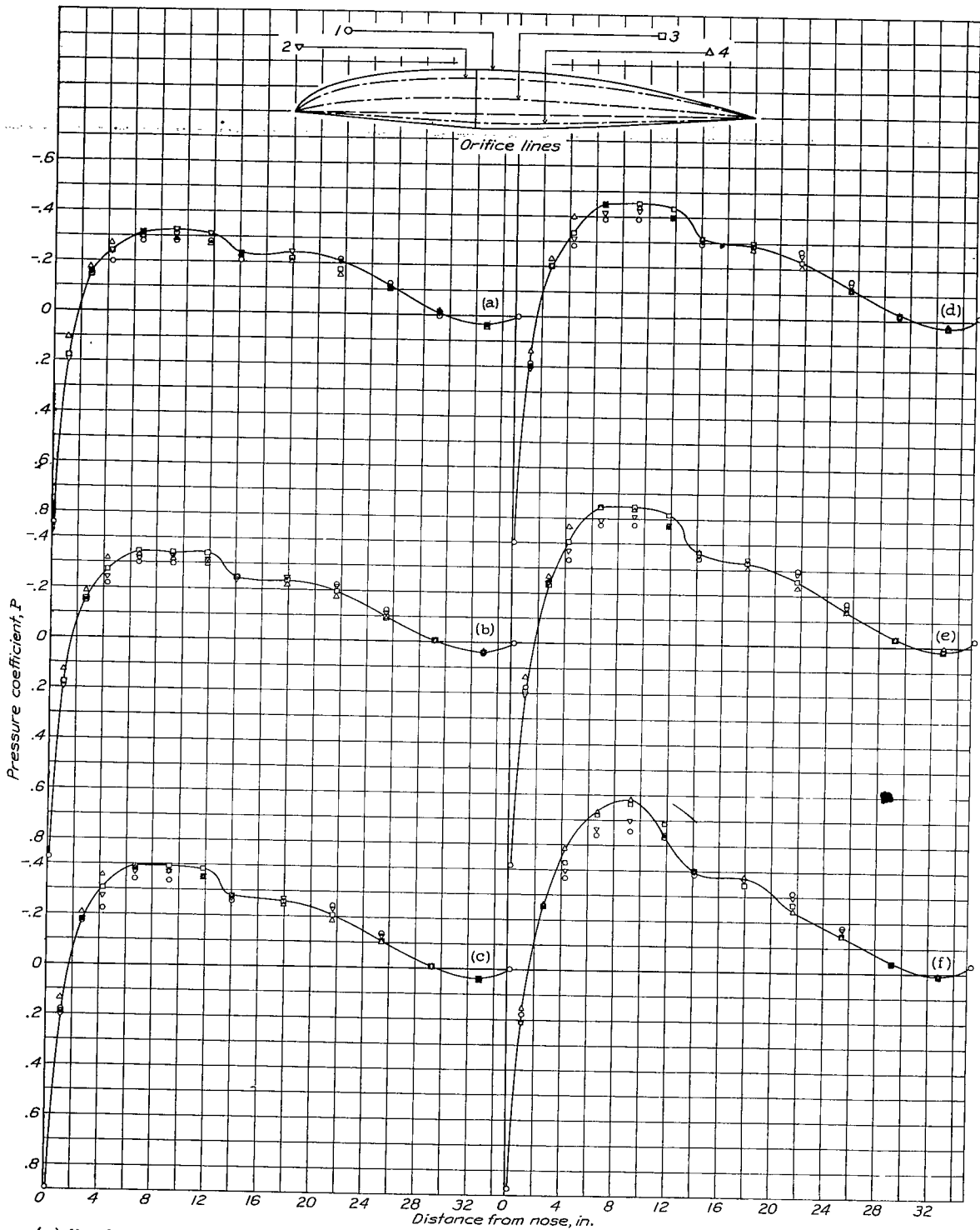
(a) M , 0.197 (b) M , 0.340 (c) M , 0.539 (d) M , 0.620 (e) M , 0.677 (f) M , 0.707 Figure 15.- Pressure distribution about the 4-0-3 windshield for various Mach numbers. \alpha , -0.67^\circ .
