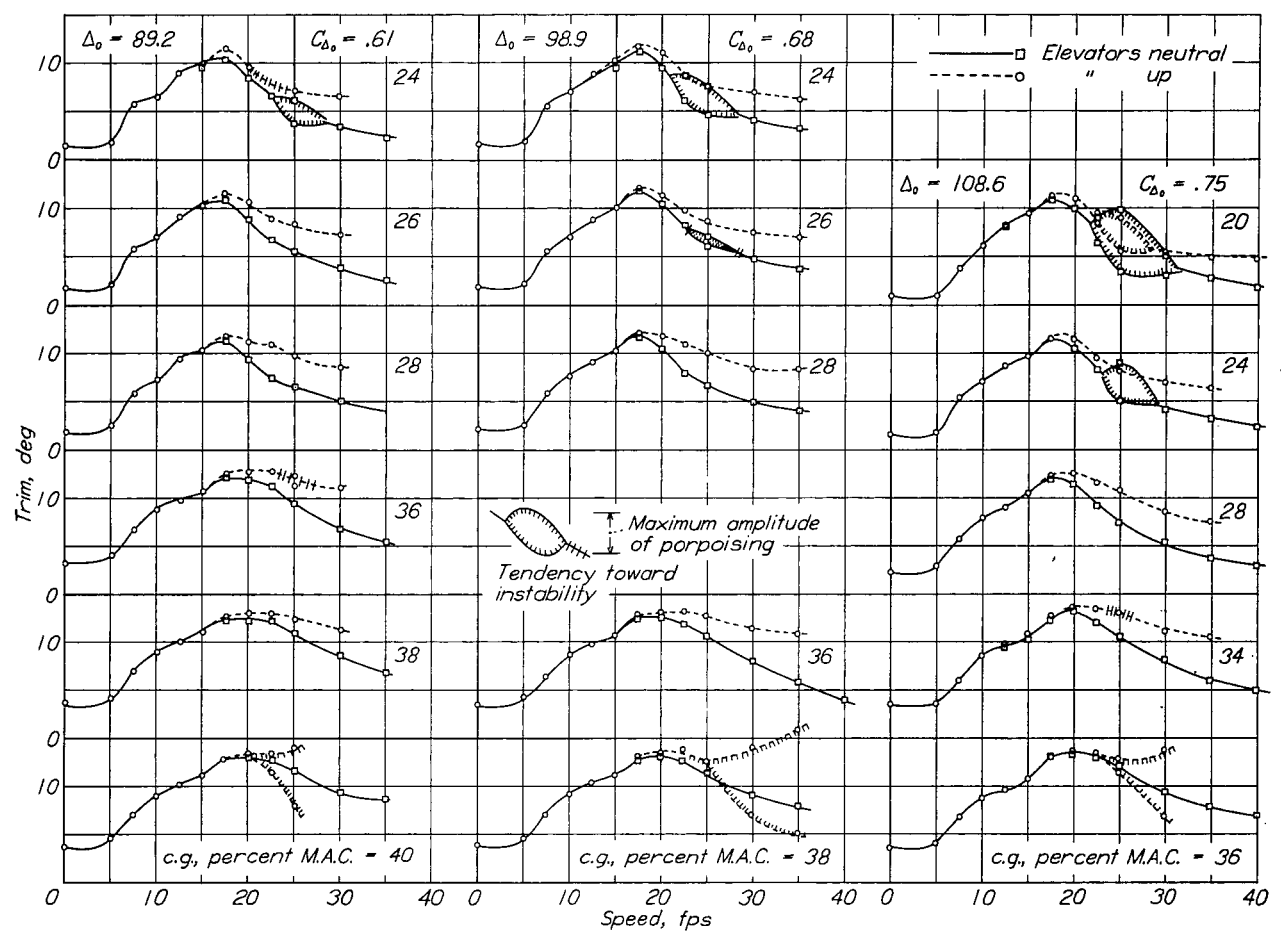
Figure 21.- Effect of position of center of gravity and gross weight on trim. Model 10, 1/8 full-size.
