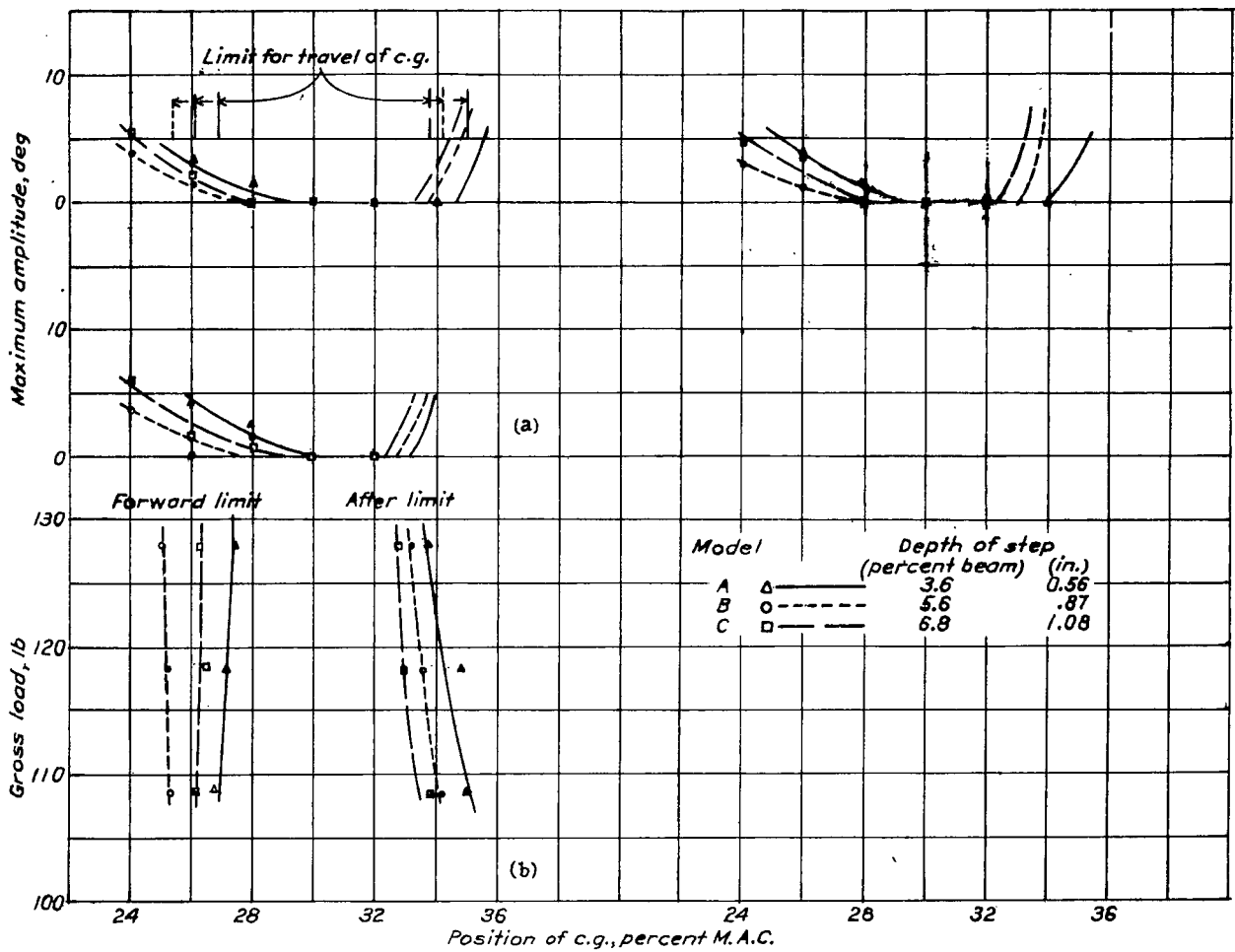
(a) On maximum amplitude of perpoising. Elevators neutral at forward positions of c. g. Elevators full up at after positions of c. g. (b) On limits for travel of the center of gravity. Forward limit of travel of c. g. After limit of travel of c. g. (maximum permissible amplitude, 20°). Length of M. A. C., 24.3 in.
