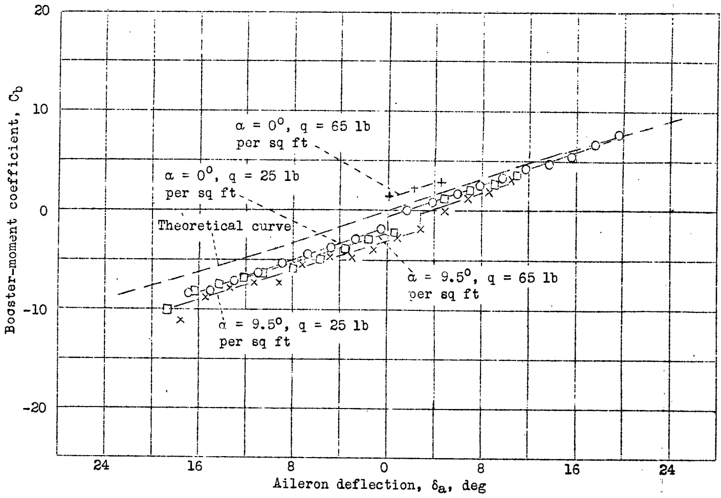
Figure 9.- Booster-moment coefficients at various aileron deflections.
