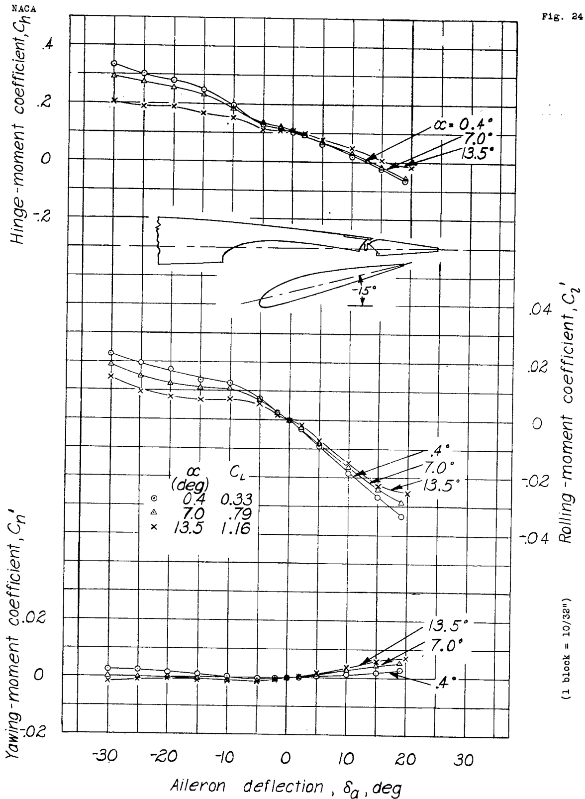
Figure 24.- Rolling-, yawing-, and hinge-moment coefficients of the tapered wing model with a full-span flap and a full-span sealed aileron. Flap position, C-6; balance, 0.30 \bar{c}_n ; \delta_s, -15^\circ .
