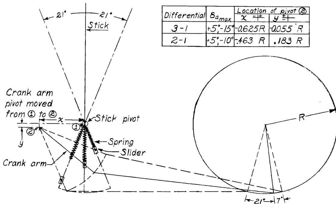
Figure 55.-Detail diagram of the differential linkage.
