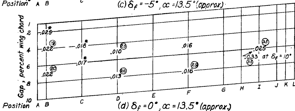
Fig. 17(a to h). - Values of rolling-moment coefficient due to aileron deflections, of \pm 15^\circ at various flap positions and deflections. Tapered wing model with a full-span flap, aileron-gap sealed.
