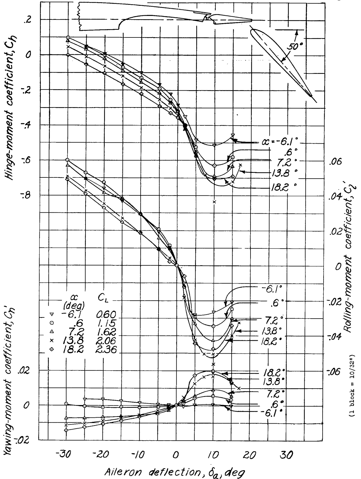
Figure 46.- Rolling-, yawing-, and hinge-moment coefficients of the tapered wing model with a full-span flap and a full-span sealed aileron. Flap position, L-\bar{x} ; balance, 0.30 \bar{c}_a ; \delta_f, 50^\circ .
