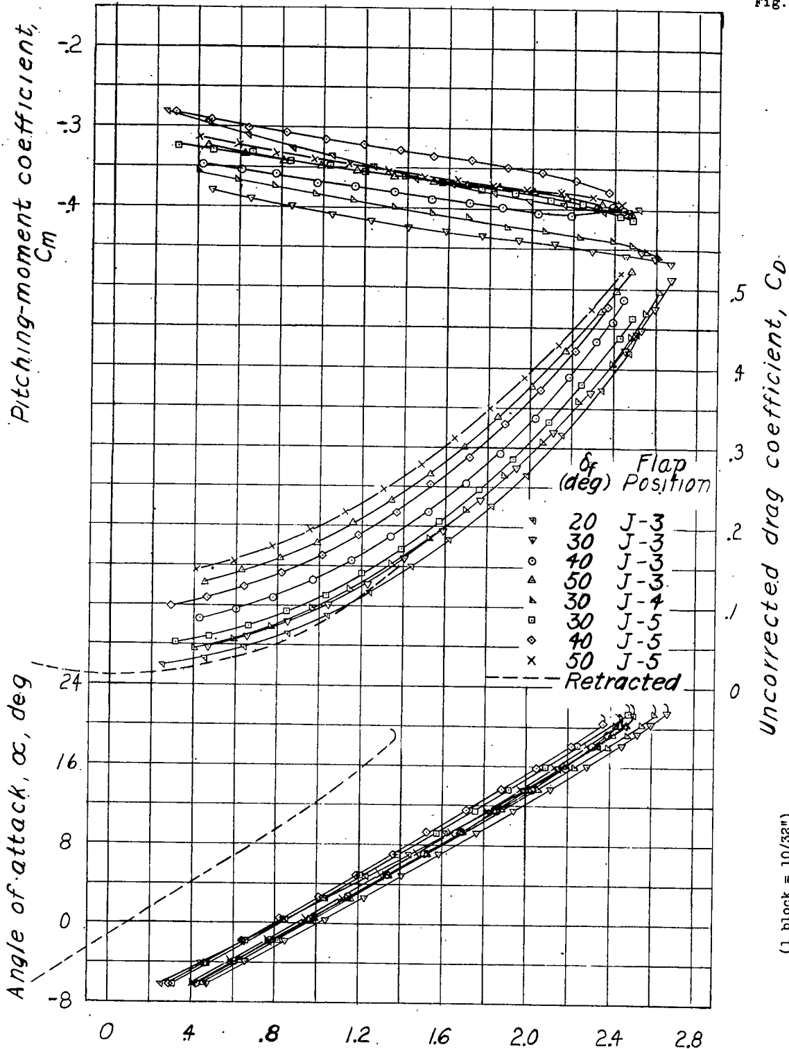
Lift coefficient, C_L Fig. 10(a, b) - Lift, drag, and pitching-moment coefficients of the tapered wing model with a full-span flap and a full-span aileron. Flap at chordwise position J. (a) \delta_a = 0^\circ
