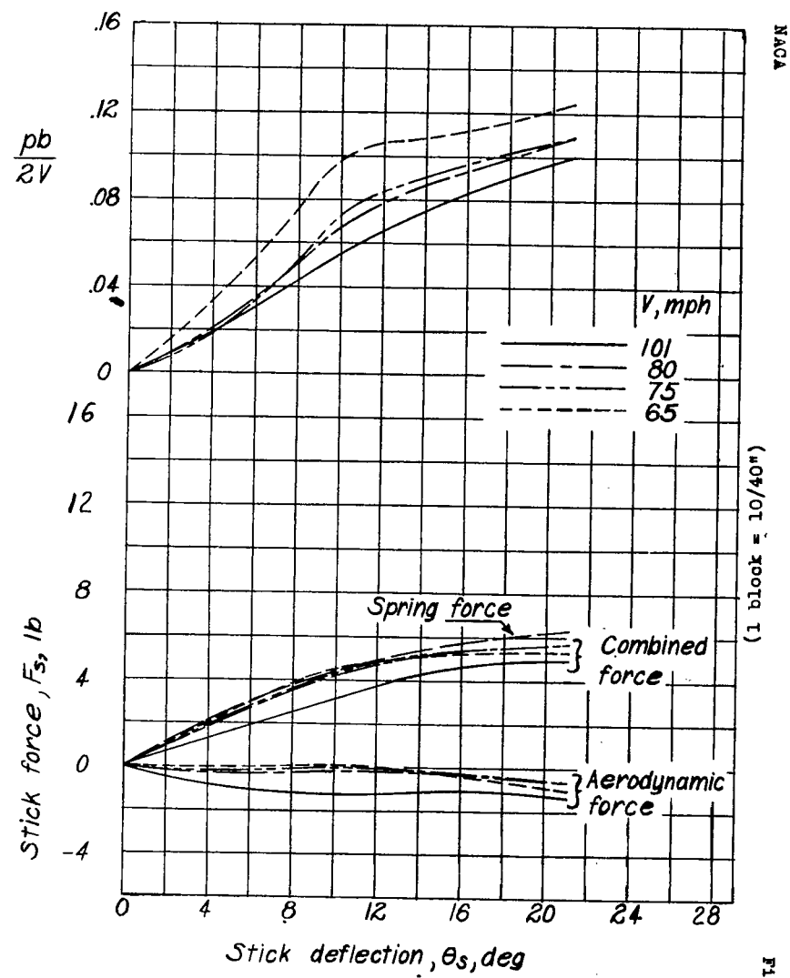
Fig 59.- Variation of stick force and pb/2V with stick deflection. Flap position, L-2, \delta_f = 50^\circ , \delta_a = 5^\circ , 2:1 differential with \delta_{a,max} = +5^\circ, -10^\circ .
