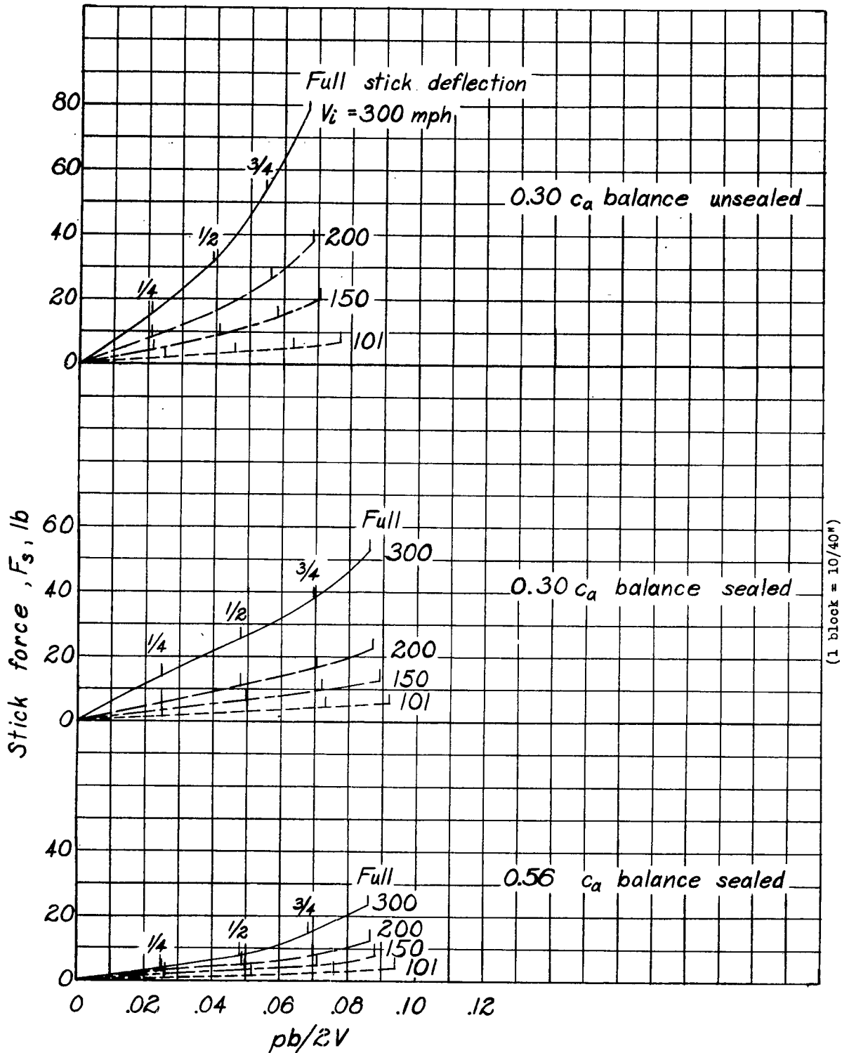
Figure 51. - Estimated aileron-control characteristics of the airplane with tapered wings, full-span flaps retracted, and balanced full-span ailerons linked for a deflection range of \pm 15^\circ .
