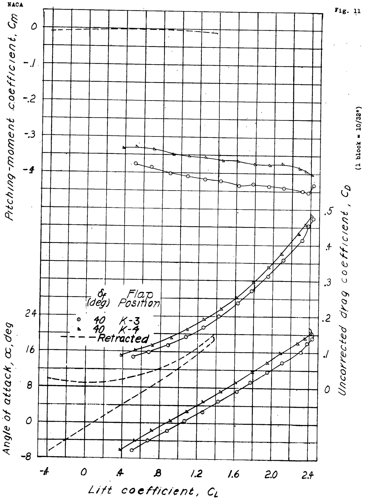
Figure 11.- Lift, drag, and pitching-moment coefficients of the tapered wing model with a full-span flap and a full-span aileron. Flap at chordwise position K; \delta_a, 0^\circ .
