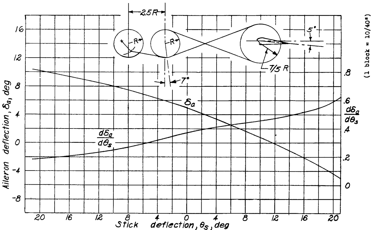
Figure 57. - Variation of aileron angle and mechanical advantage with stick deflection. Aileron drooped 5° with a 2:1 differential; \delta_{a\max} = +5^\circ, -10^\circ .
