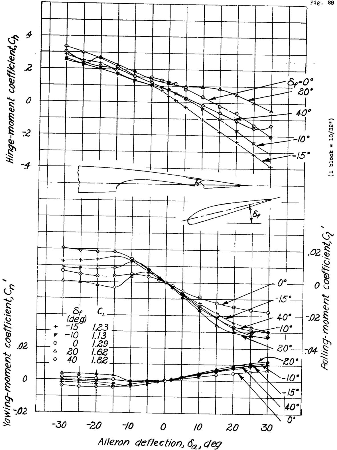
Figure 29.- Rolling-, yawing-, and hinge-moment coefficients of the tapered wing model with a full-span flap and a full-span sealed aileron. Flap position, F-8; balance 0.30 C_a ; \alpha , 13.6° (approx.).
