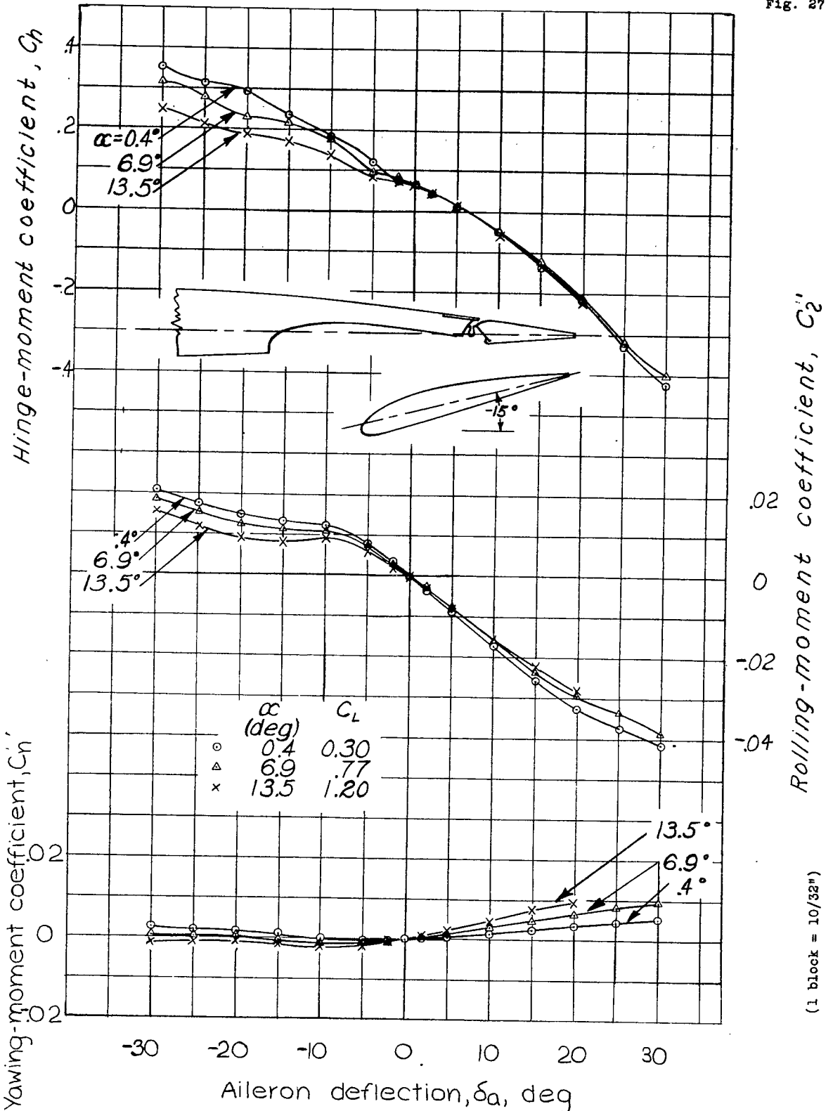
Figure 27. Rolling-, yawing-, and hinge-moment coefficients of the tapered wing model with a full-span flap and a full-span sealed aileron. Flap position, D-8; balance, 0.30\bar{c}_a ; \delta_f, -15^\circ .
