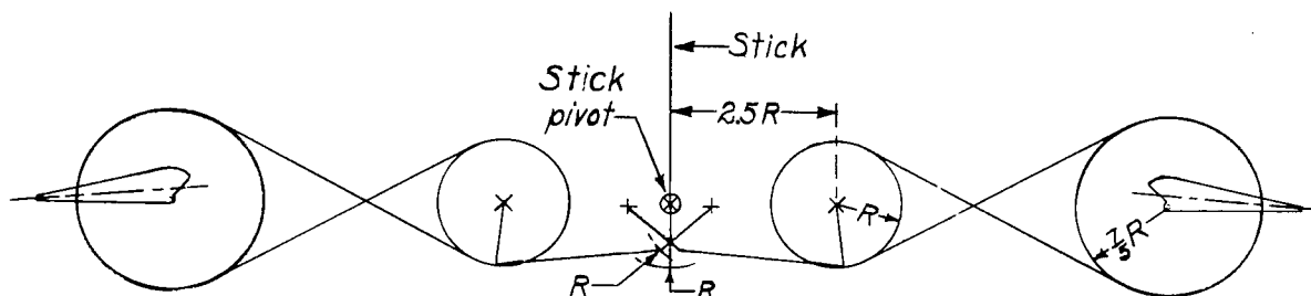
Figure 54.-Schematic diagram of 3:1 differential aileron linkage with a 5^\circ aileron droop. \delta_{a\max}, +5^\circ, -15^\circ
