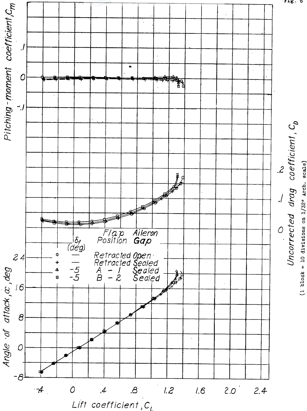
Figure 6.- Lift, drag, and pitching-moment coefficients of the tapered wing model with a full-span flap and full-span aileron. Flap retracted and at chordwise positions A and B; \delta_a, 0^\circ .
