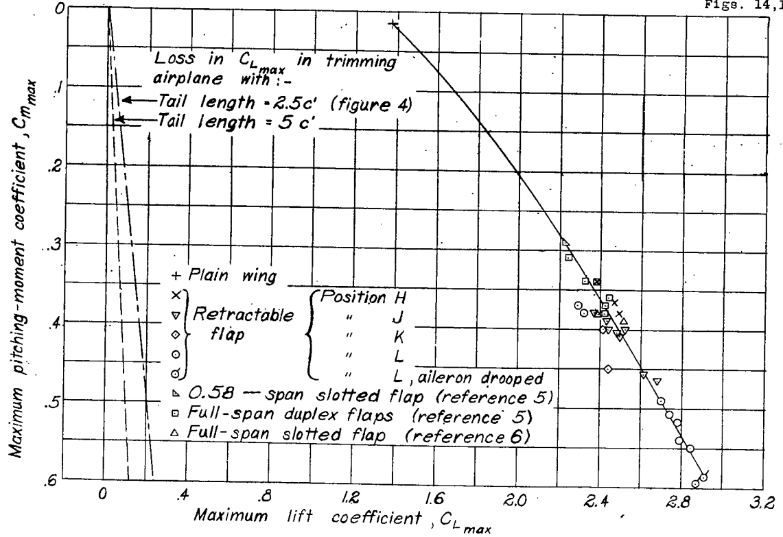
Figure 14.-Variation of the maximum pitching-moment coefficient with maximum lift coefficient for various arrangements of high-lift and lateral-control devices on a tapered wing model.
