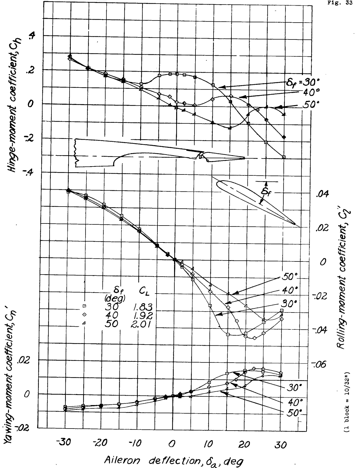
Figure 33 - Rolling-, yawing-, and hinge-moment coefficients of the tapered wing model with a full-span flap and a full-span sealed aileron. Flap position, H-5; balance, 0.30 \bar{c}_a ; \alpha , 13.8°.
