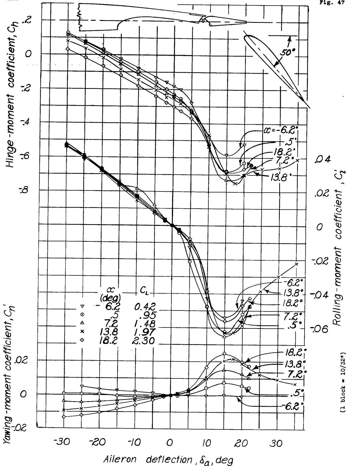
Figure 47. - Rolling-yawing- and hinge-moment coefficients of the tapered wing model with a full-span flap and a full-span sealed aileron. Flap position, L-3; balance, 0.30 \bar{c}_a ; \delta_f , 50°.
