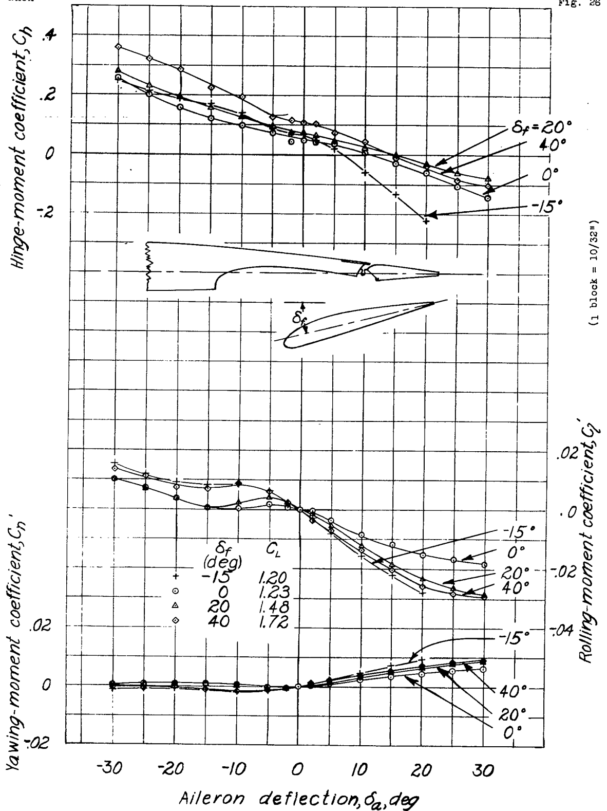
Figure 26.-Rolling-, yawing-, and hinge-moment coefficients of the tapered wing model with a full-span flap and a full-span sealed aileron. Flap position, D-8; balance, 0.30\bar{c}_a ; \alpha , 13.6^\circ (approx.).
