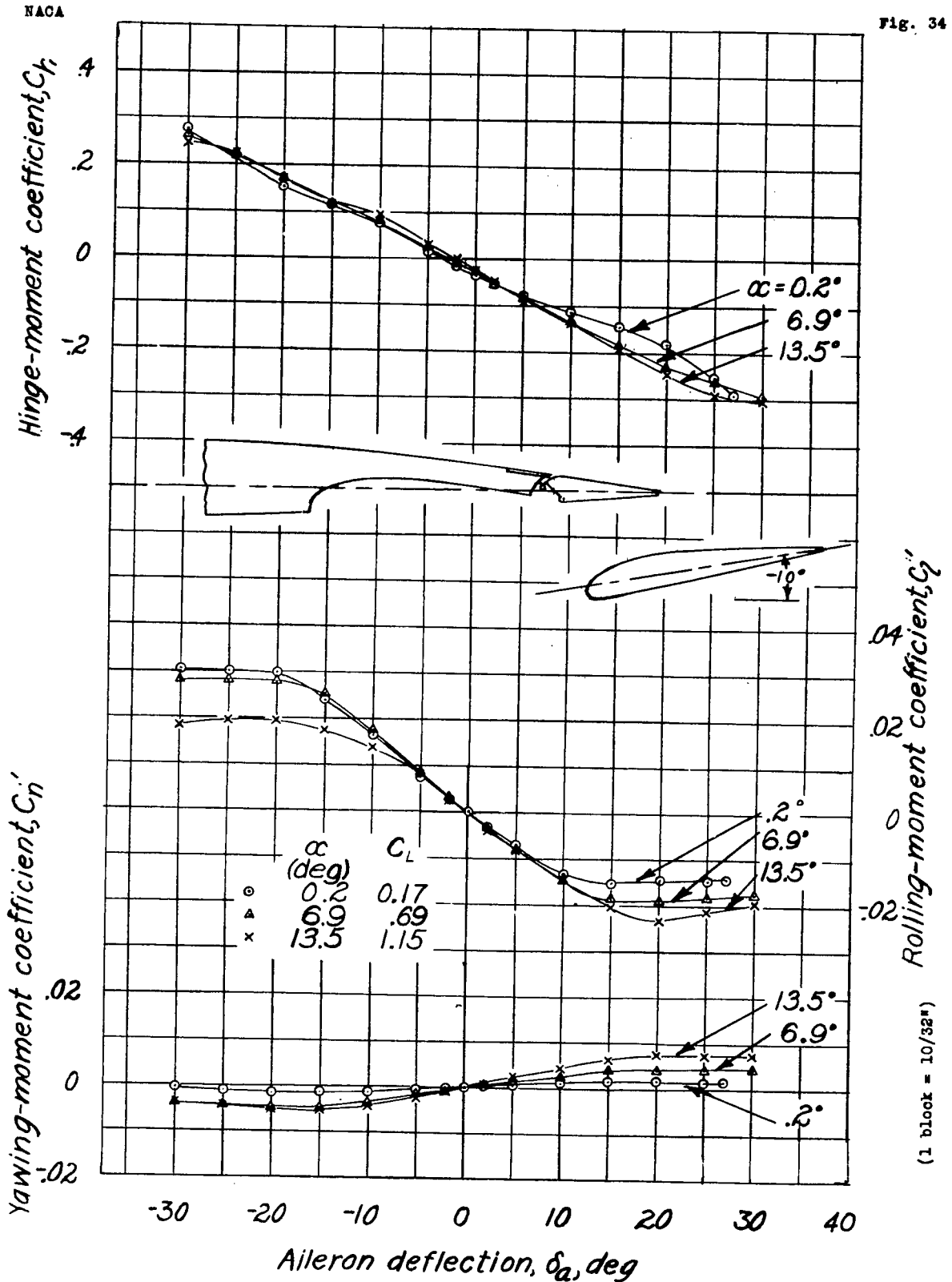
Figure 34.- Rolling-, yawing-, and hinge-moment coefficients of the tapered wing model with a full-span flap and a full-span aileron. Flap position, H-8; balance, 0.30 C_{H_0} ; \delta_f , -10°.
