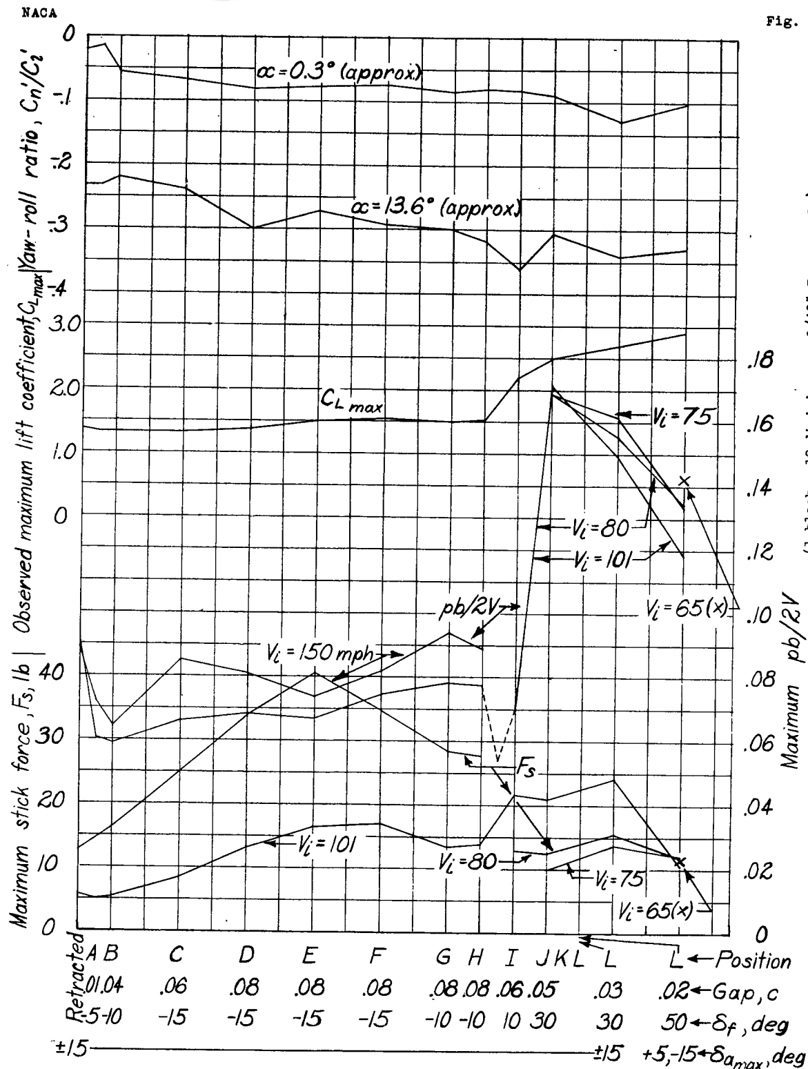
Figure 50.- Estimated aileron-control characteristics of the airplane with tapered wings, full-span flaps, and full-span ailerons. Balance, 0.30 \bar{c}_a ; gap sealed.
