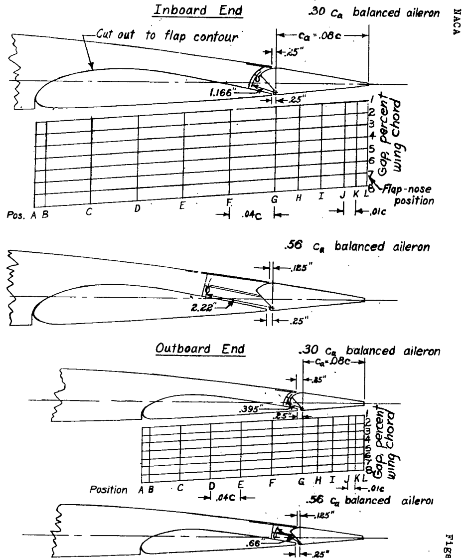
Figure 5. - Aileron details of model.
