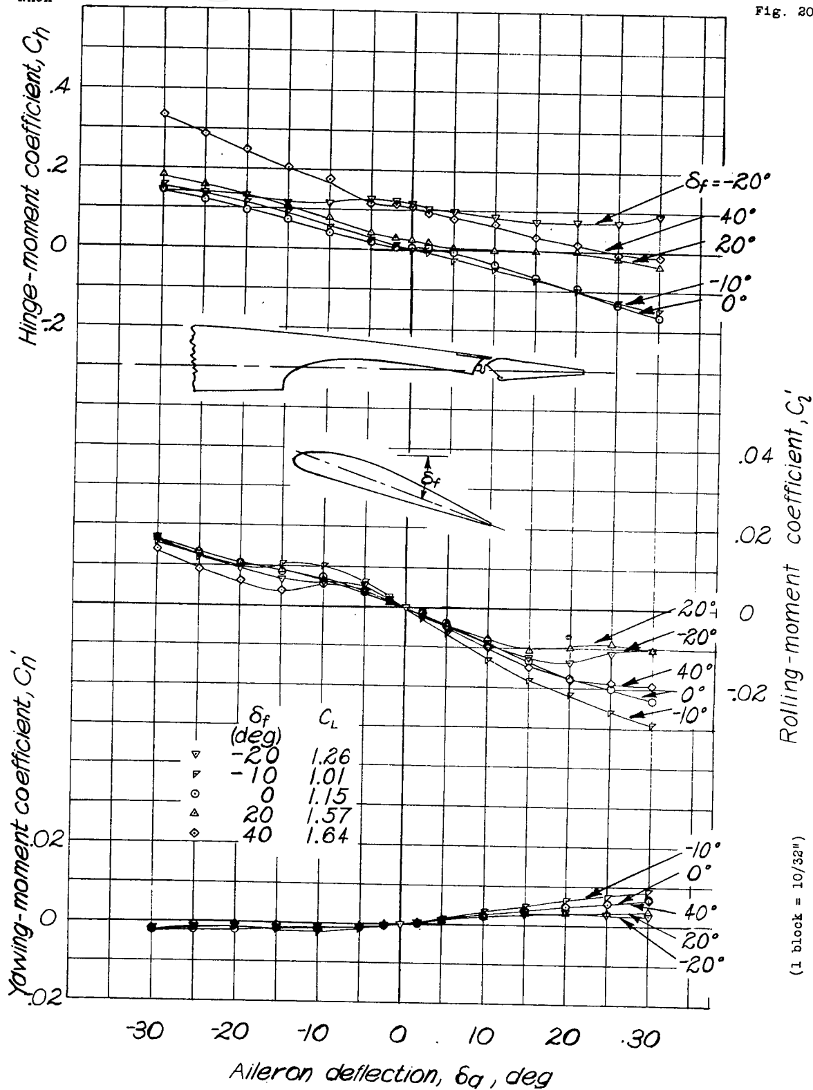
Figure 20.—Rolling-, yawing-, and hinge-moment coefficients of the tapered wing model with a full-span flap and a full-span sealed aileron. Flap position, B-7; balance, 0.30 C_a ; \alpha , 13.6° (approx)
