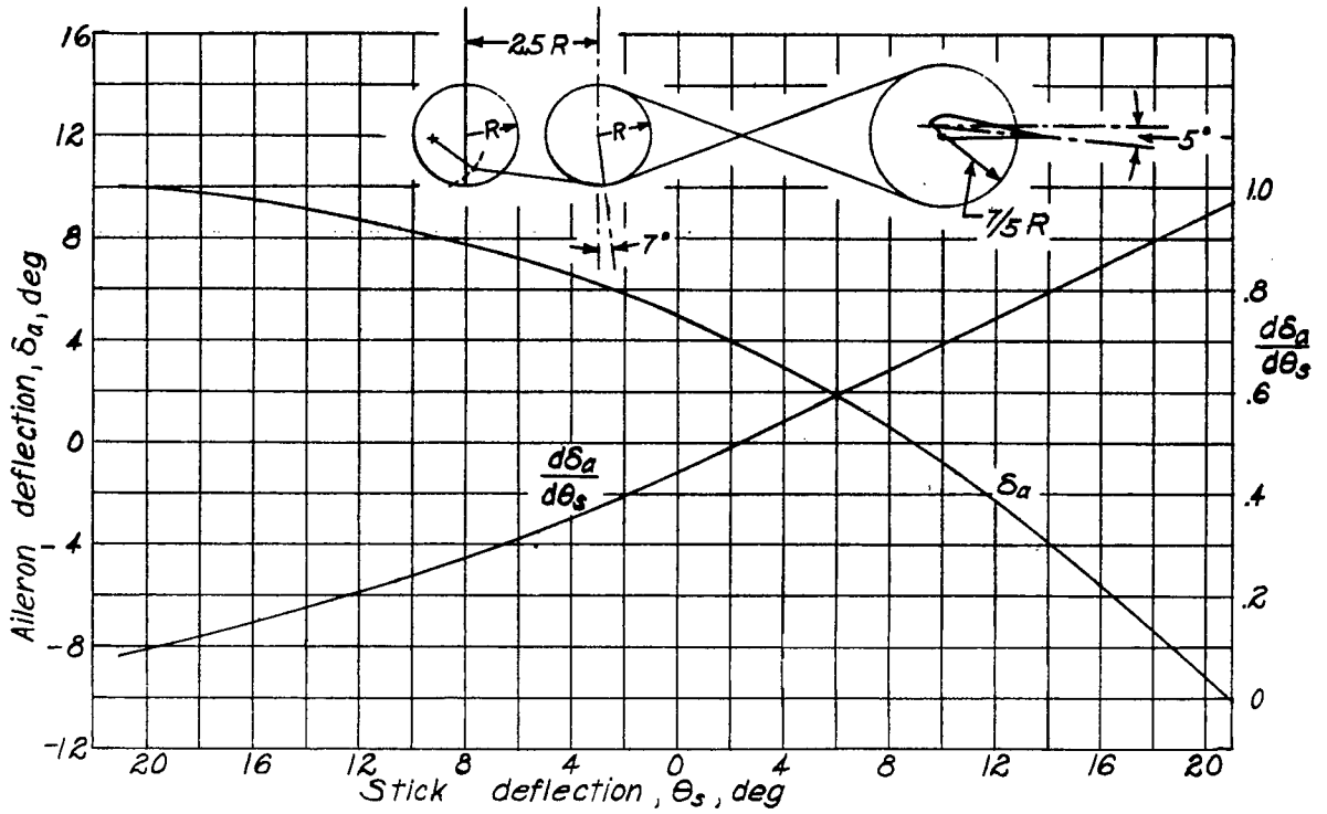
Figure 56.- Variation of aileron angle and mechanical advantage with stick deflection. Aileron drooped 5° with a 3:1 differential; \delta_{a\max} = +5^\circ, -15^\circ .
