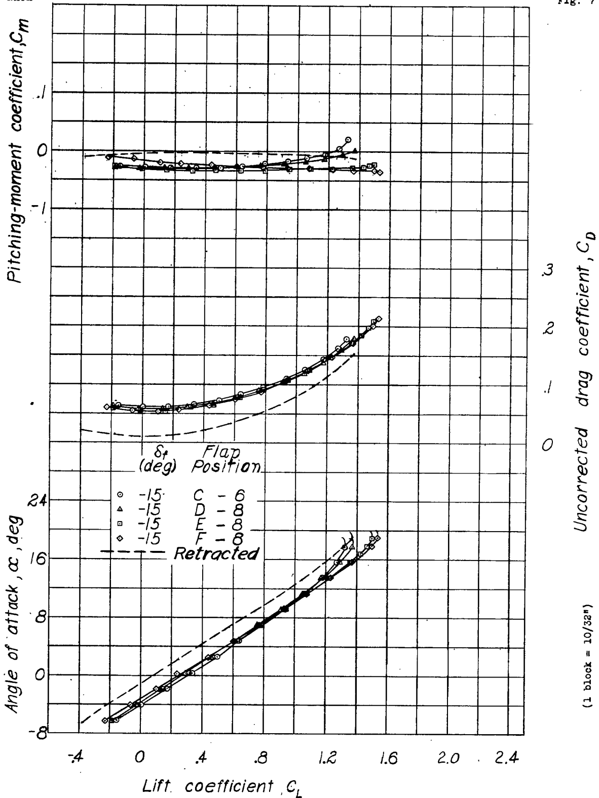
Figure 7.- Lift, drag, and pitching-moment coefficients of the tapered wing model with a full-span flap and a full-span aileron. Flap at chordwise positions C, D, E, and F; \delta_a, 0^\circ .
