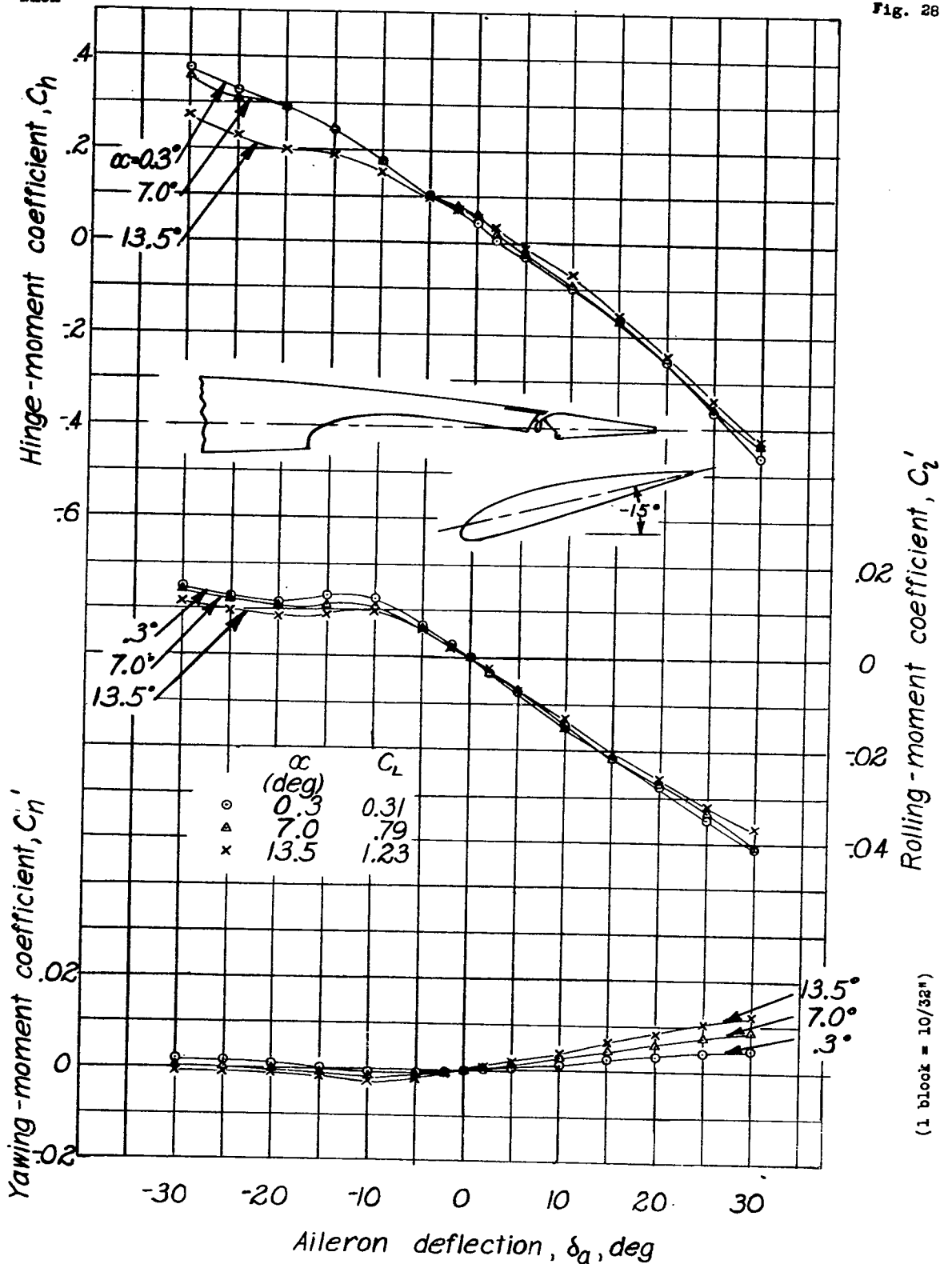
Figure 28.- Rolling-, yawing-, and hinge-moment coefficients of the tapered wing model with a full-span flap and a full-span sealed aileron. Flap position, E-8; balance, 0.30c_a ; \alpha_f, -15^\circ .
