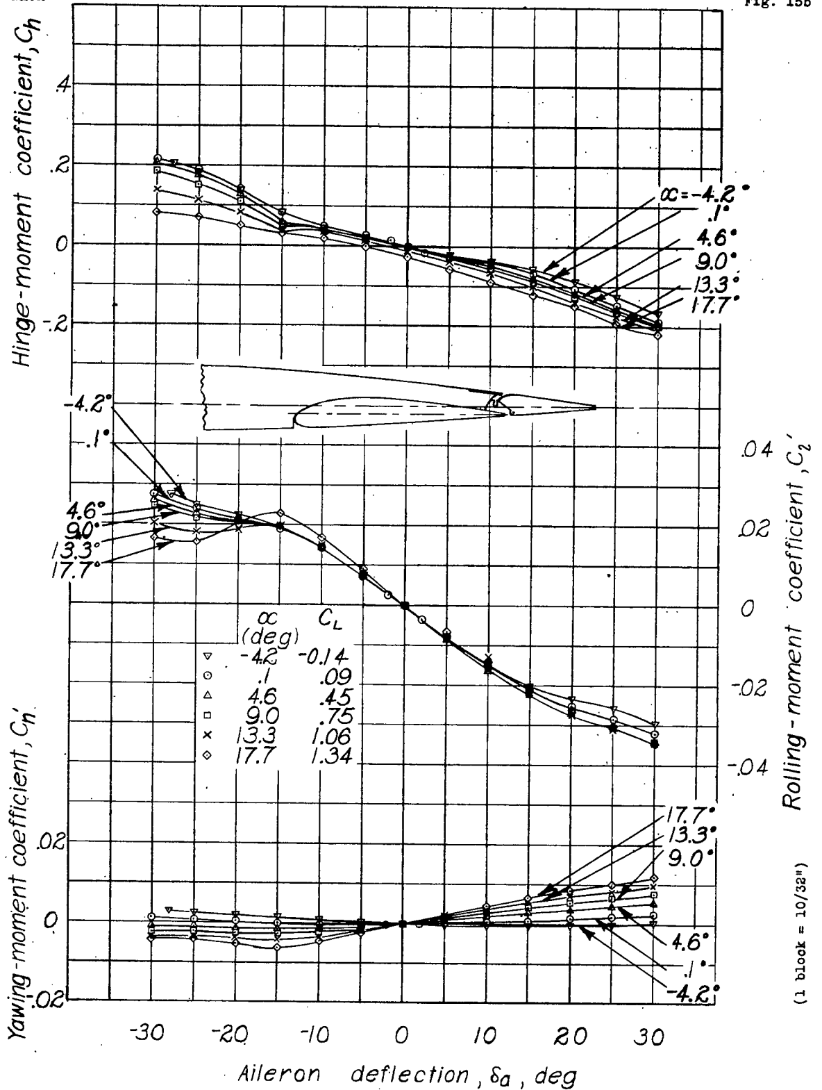
(b) Balance, 0.30 \bar{c}_a ; gap sealed.
