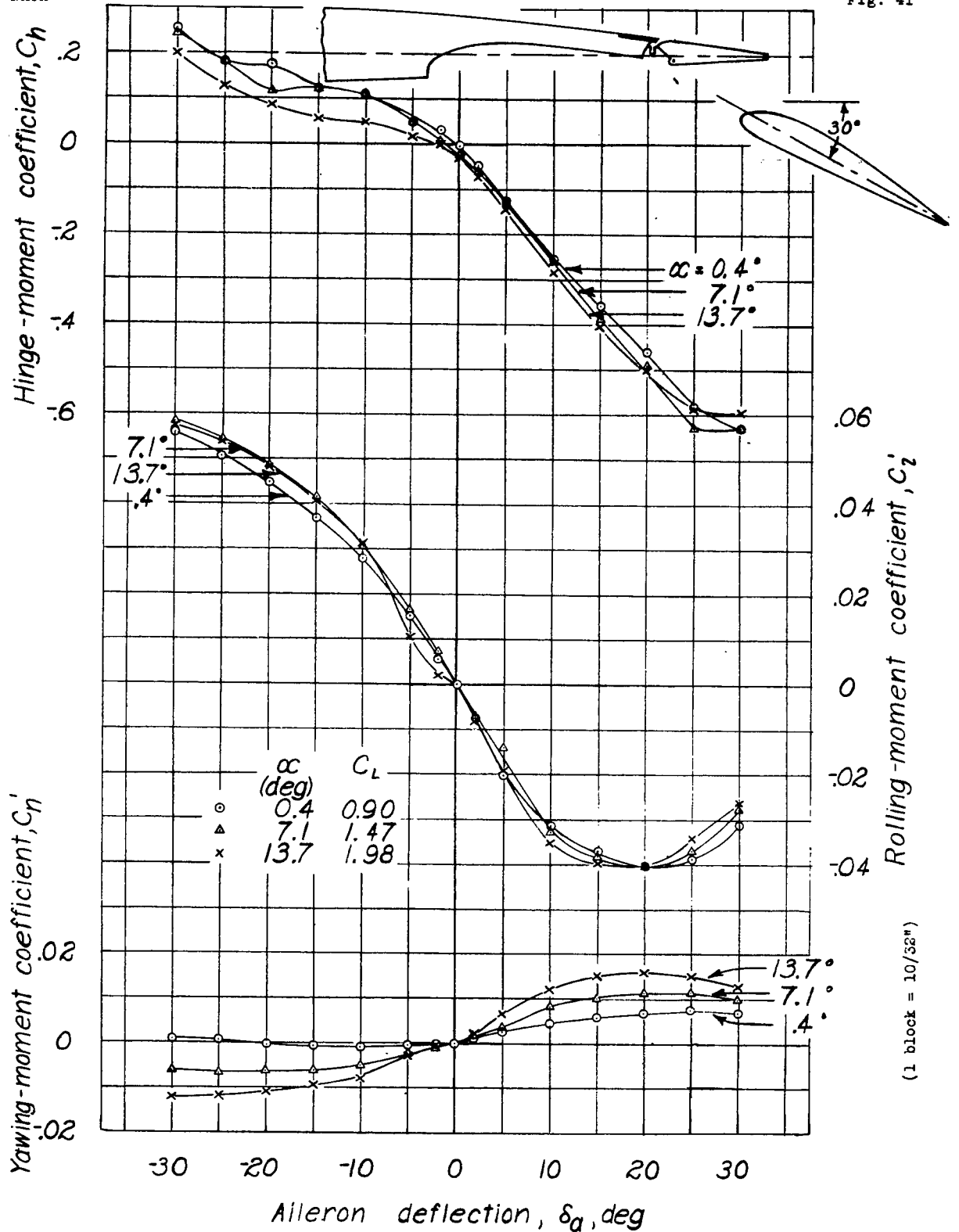
Figure 41.- Rolling-, yawing-, and hinge-moment coefficients of the tapered wing model with a full-span flap and a full-span sealed aileron. Flap position, J-5; balance, 0.30 c_a ; \delta_f, 30^\circ .
