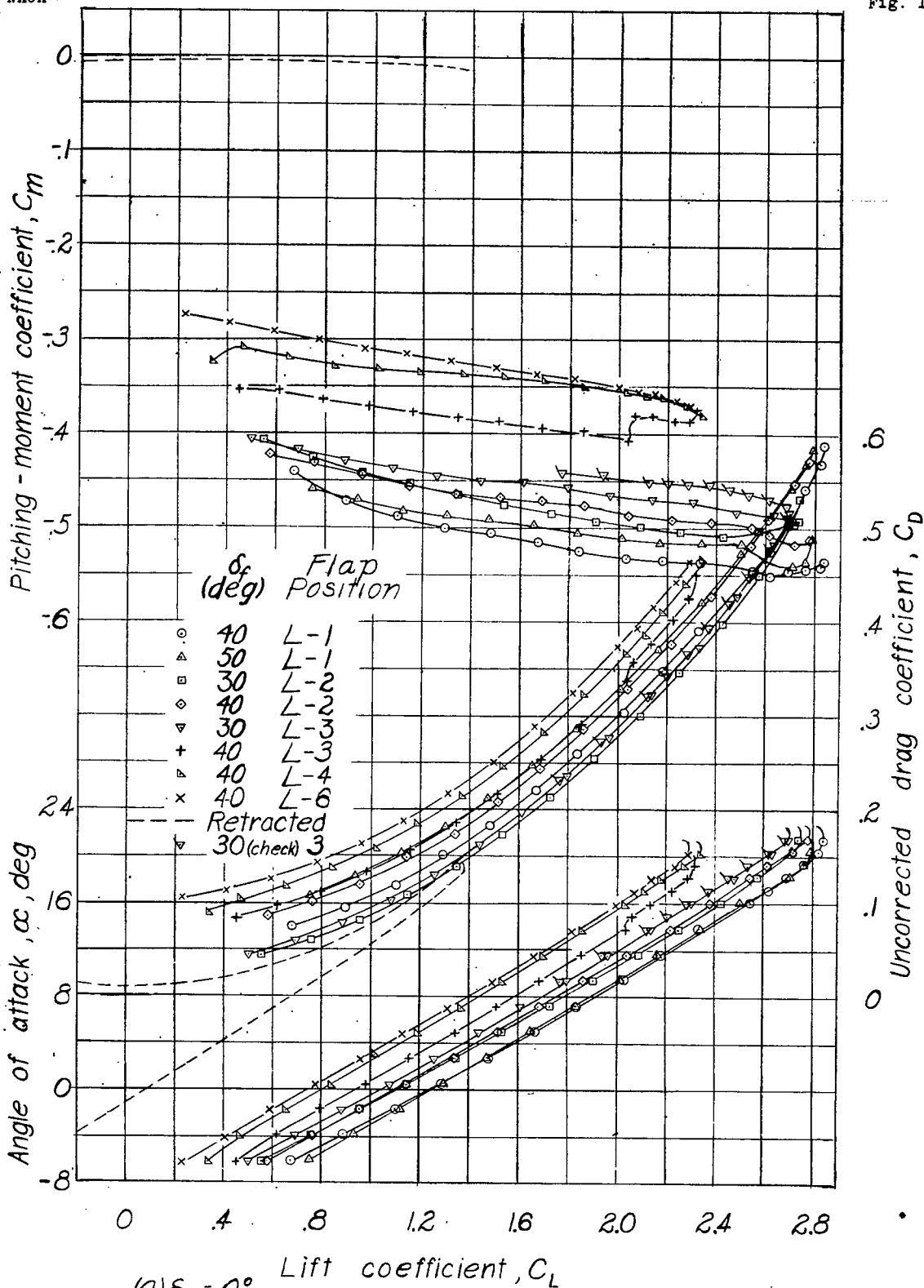
Fig. 12(a,b).-Lift, drag, and pitching-moment coefficients of the tapered wing model with a full-span flap and a full-span aileron. Flap at chordwise position L
