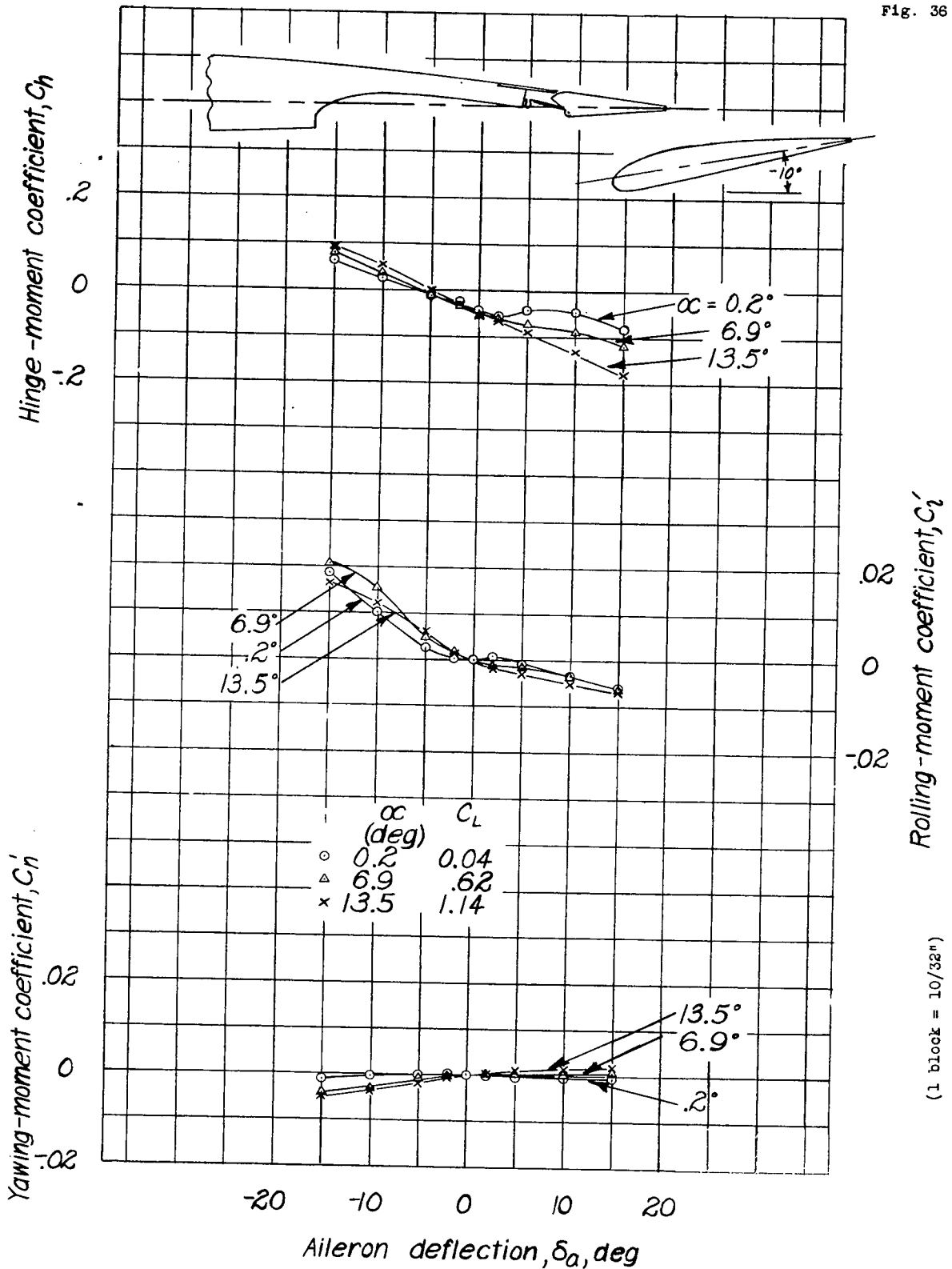
Figure 36.- Rolling-, yawing-, and hinge-moment coefficients of the tapered wing model with a full-span flap and a full-span sealed aileron. Flap position, I-6; balance, 0.56 \bar{c}_a ; \delta_f, -10^\circ
