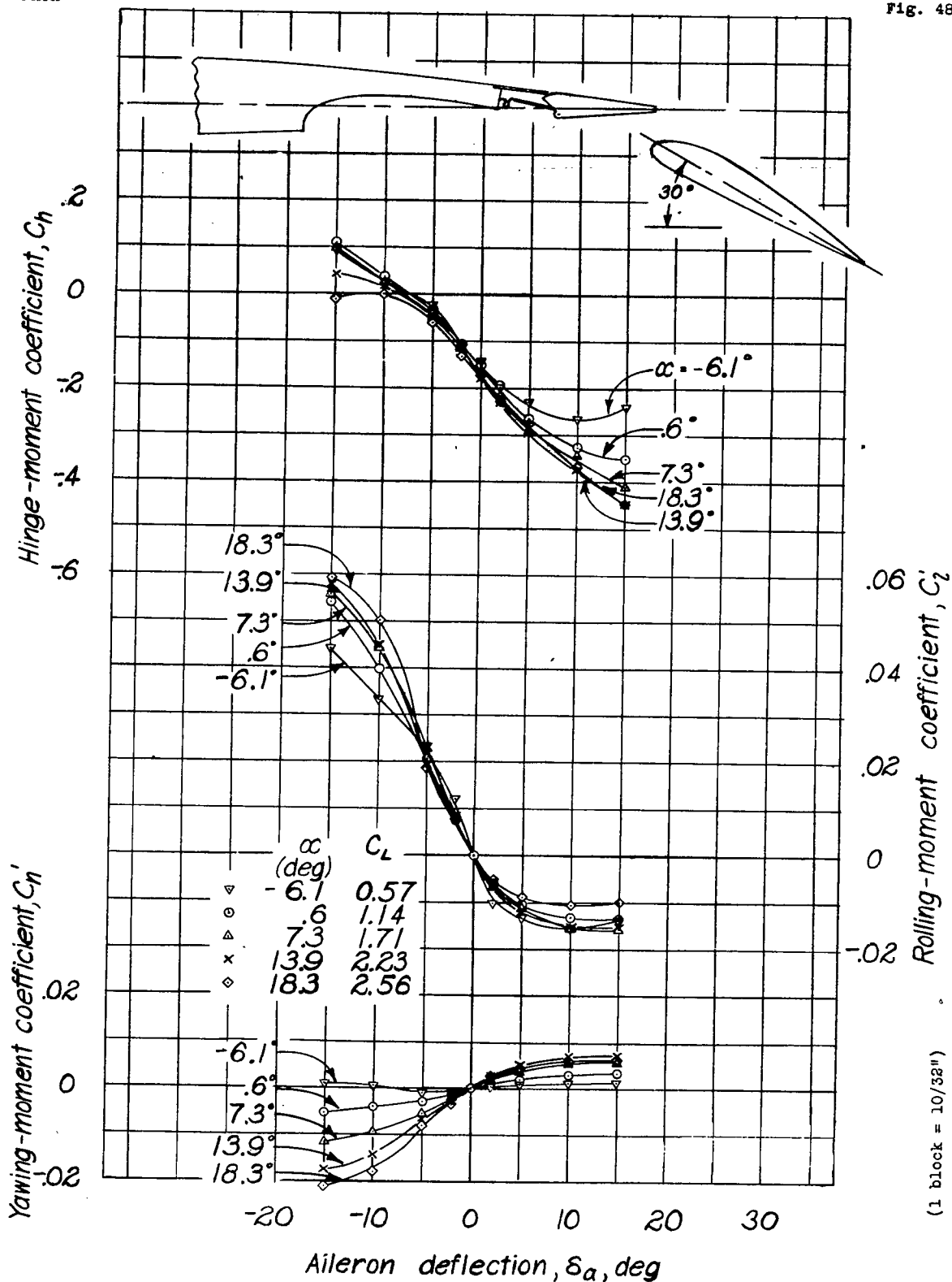
Figure 48.- Rolling-, yawing-, and hinge-moment coefficients of the tapered wing model with a full-span flap and a full-span sealed aileron. Flap position, L-3; balance, 0.56 \bar{c}_a ; \delta_{fl} , 30^\circ .
