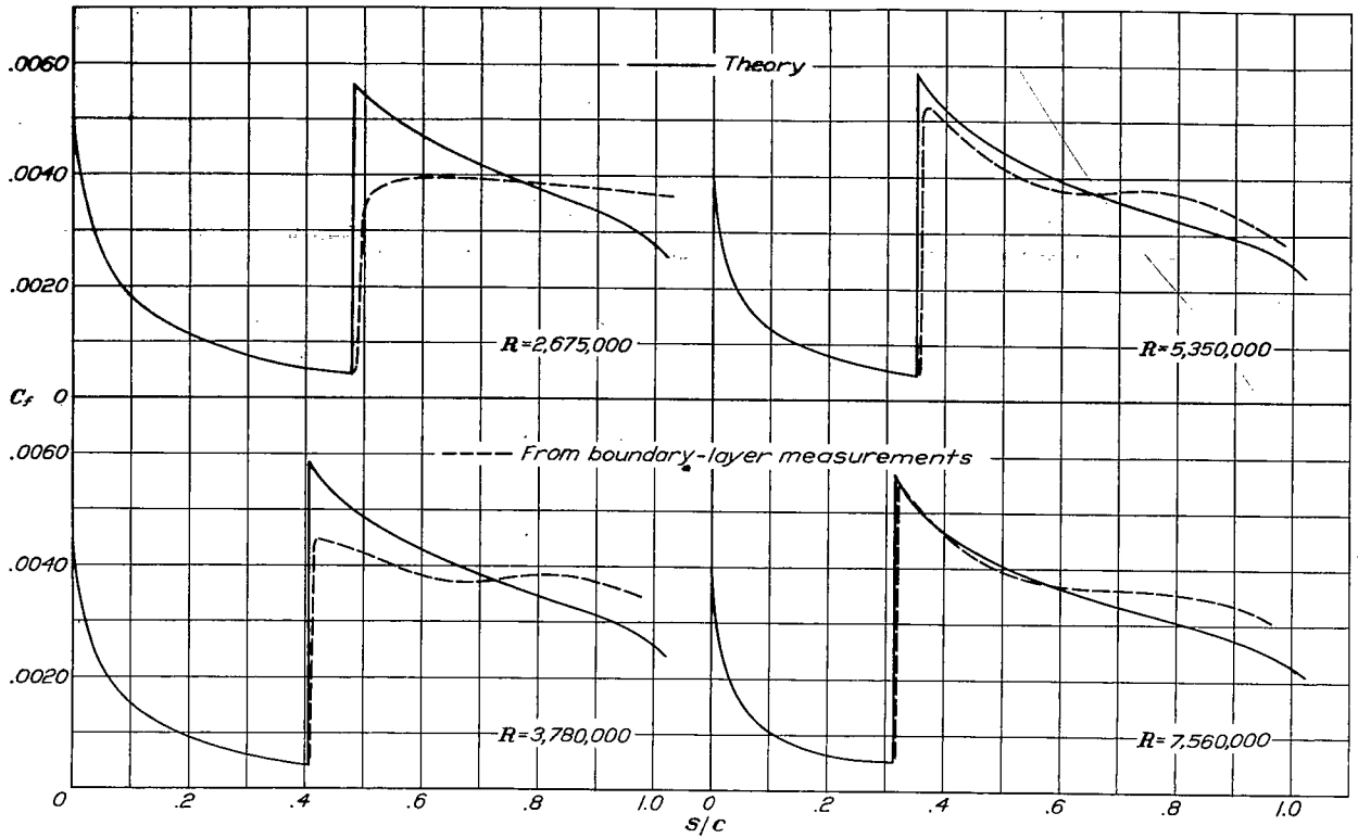
Figure 24.- Distribution of skin friction along the surface of N.A.C.A. 0012 airfoil.
