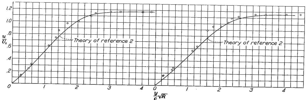
Figure 8.- Boundary-layer survey 0.37c along surface from leading edge of N.A.C.A. 0012 airfoil.
