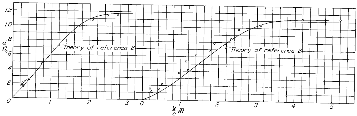
Figure 10.- Boundary-layer survey 0.52c along surface from leading edge of N.A.C.A. 0012 airfoil.
