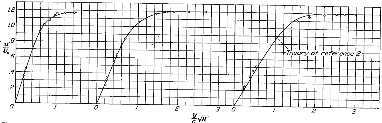
Figure 6.- Boundary-layer survey 0.22c along surface from leading edge of N.A.C.A. 0012 airfoil.
