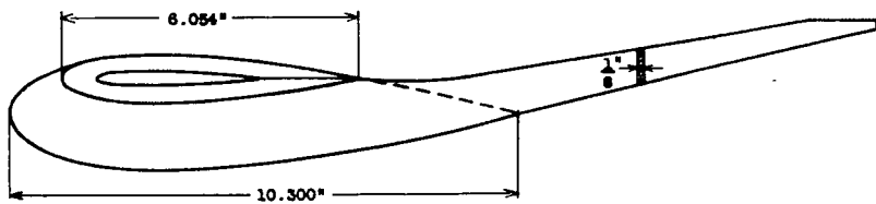
Figure 1.- Wing-fuselage combination with airfoil-type fuselage.
