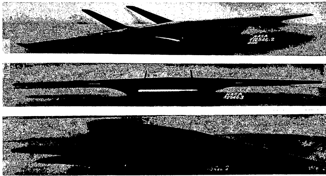
Figure 7.- Combination with large fillets.
