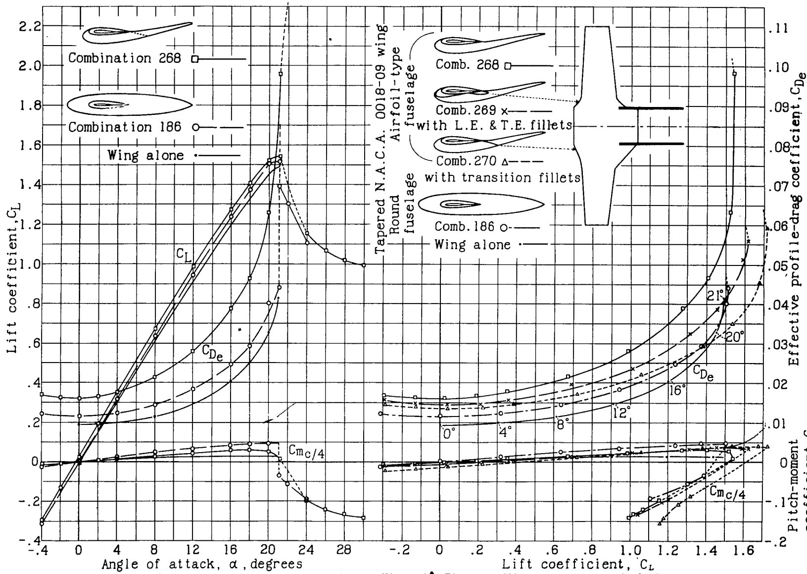
Figure 2.- Comparison of airfoil-type fuselage and conventional wing-fuselage combinations.
