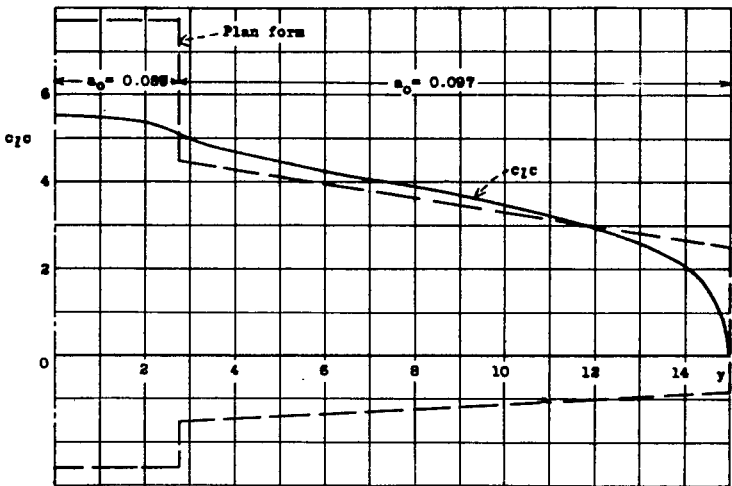
Figure 4.- Span load distribution for airfoil-type-fuselage combination.
