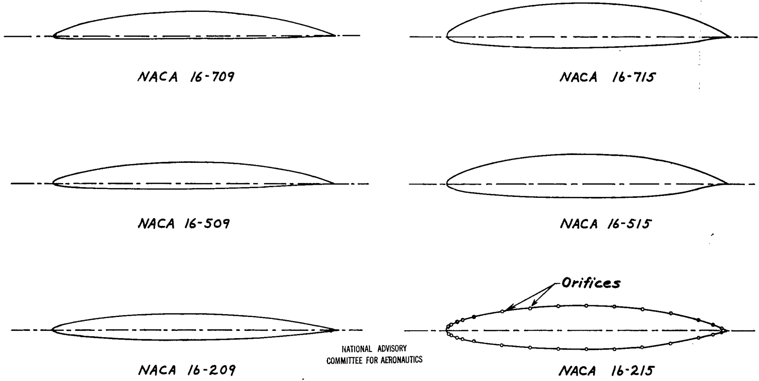
Figure 1.- Airfoil profiles tested and distribution of pressure orifices.
