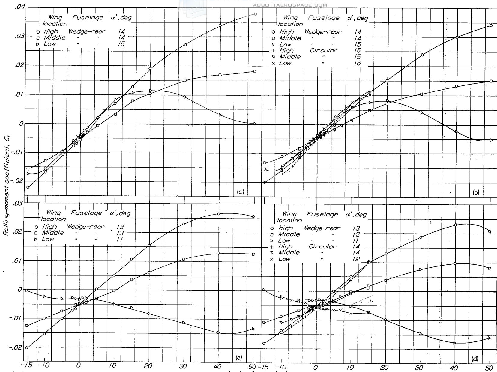
(a) Tail off, \delta_f = 0^\circ (b) Tail on, \delta_f = 0^\circ (c) Tail off, \delta_f = 60^\circ (d) Tail on, \delta_f = 60^\circ Figure 11.- Variation of rolling-moment coefficient with yaw. NACA 23012 wing with fuselage, \Lambda = 4.75^\circ . (Data for circular fuselage converted from reference 2.)
