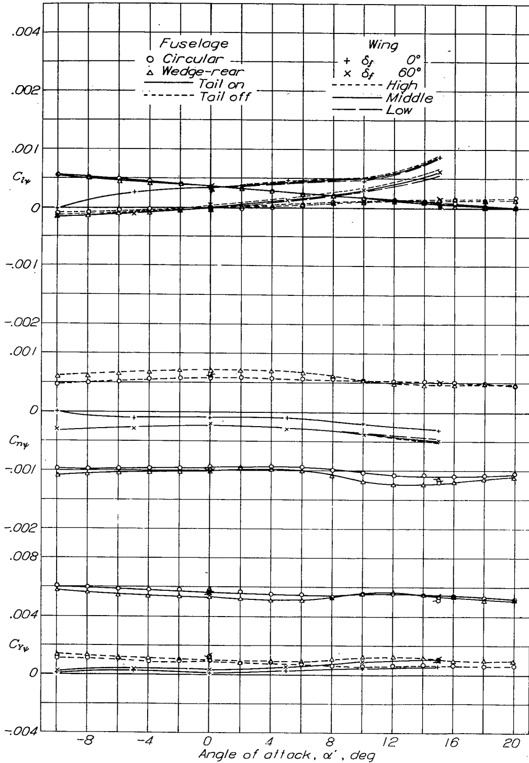
Figure 3.- Variation of C_{l_w} , C_{n_w} , and C_{y_w} with angle of attack. NACA 23012 wing alone, fuselage alone, and fuselage with tail. (Data for wing and circular fuselage converted from references 7 and 1, respectively.)
