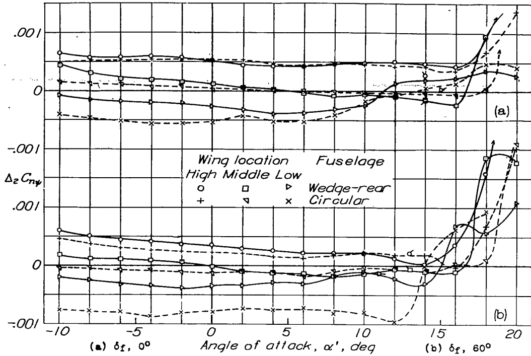
Figure 8.- Effect of wing-fuselage interference on C_{np} due to tail. NACA 23012 wing with fuselage and tail. (Data for circular fuselage converted from reference 2.)
