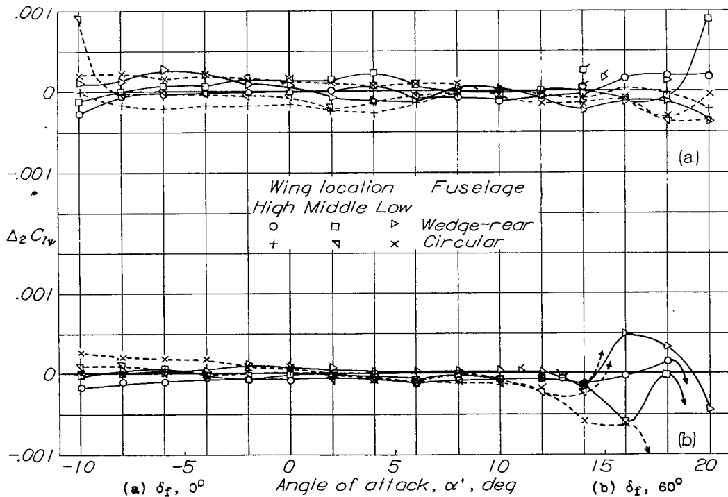
Figure 7.- Effect of wing-fuselage interference on C_{l\psi} due to tail. NACA 23012 wing with fuselage and tail. (Data for circular fuselage converted from reference 2.)
