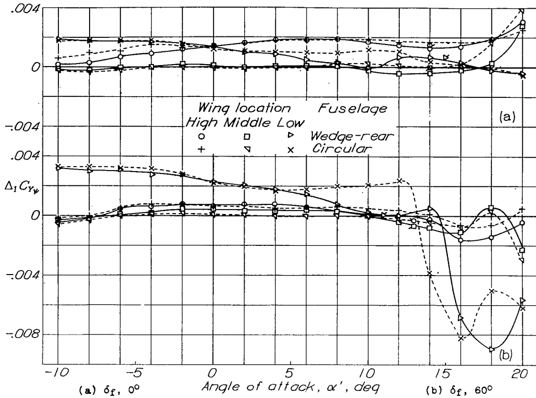
Figure 6.- Increment of C_{Y\psi} due to wing-fuselage interference. NACA 23012 wing with fuselage. (Data for circular fuselage converted from reference 2.)
