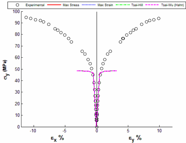
Figure 30. ±45° angle ply laminate E-glass/MY750/HY917/DY063: Stress/strain curve for \sigma_y/\sigma_x = 1/-1 with HFGMC
