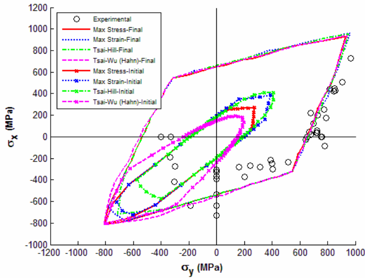
Figure 13. (0°/±45°/90°) laminate AS4/3501-6: \sigma_y vs \sigma_x failure stress envelope with GMC
