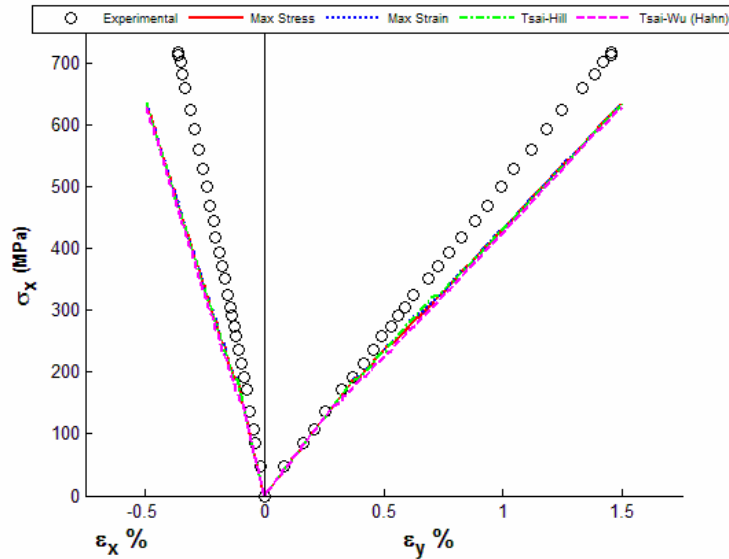
Figure 15. (0^\circ/\pm 45^\circ/90^\circ) laminate AS4/3501-6: Stress/strain curves for \sigma_y/\sigma_x = 0/1 with GMC
