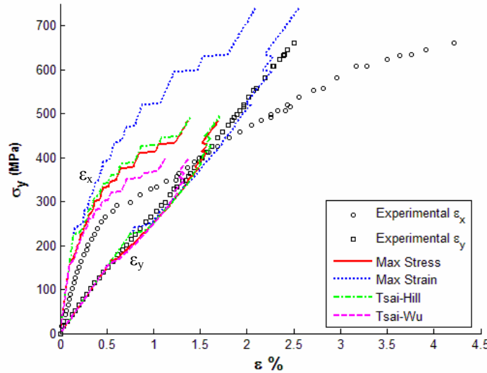
Figure 23. ±55° angle ply laminate E-glass/MY750/HY917/DY063: Stress/strain curve for \sigma_y/\sigma_x = 2/1 with GMC
