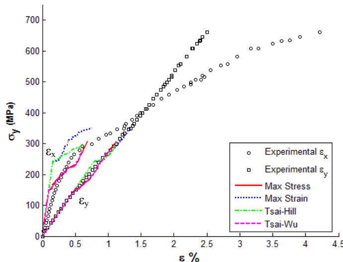
Figure 24. ±55° angle ply laminate E-glass/MY750/HY917/DY063: Stress/strain curve for \sigma_y/\sigma_x = 2/1 with HFGMC
