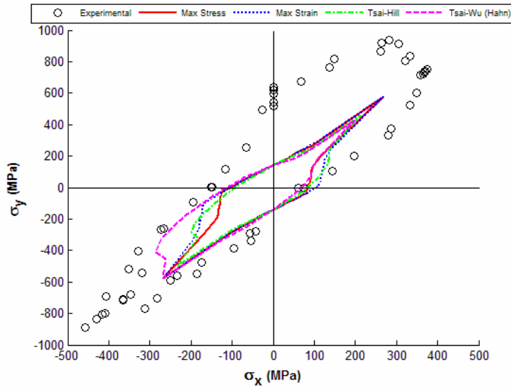
Figure 19. ±55° angle ply laminate E-glass/MY750/HY917/DY063: \sigma_y vs \sigma_x failure stress envelope with GMC
