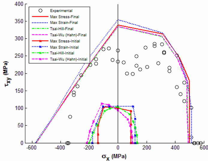
Figure 11. (90^\circ/\pm 30^\circ/90^\circ) laminate E-glass/LY556/HT907/DY063: \sigma_y vs \tau_{xy} failure stress envelope with GMC
