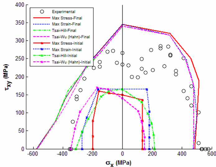
Figure 12. (90^\circ/\pm 30^\circ/90^\circ) laminate E-glass/LY556/HT907/DY063: \sigma_y vs \tau_{xy} failure stress envelope with HFGMC
