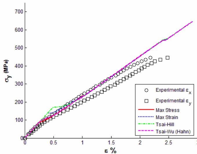
Figure 28. ±45° angle ply laminate E-glass/MY750/HY917/DY063: Stress/strain curve for \sigma_y/\sigma_x = 1/1 with HFGMC
