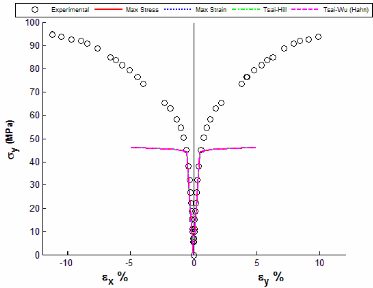
Figure 29. ±45° angle ply laminate E-glass/MY750/HY917/DY063: Stress/strain curve for \sigma_y/\sigma_x = 1/-1 with GMC
