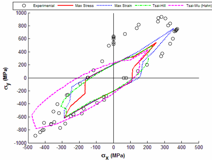
Figure 20. ±55° angle ply laminate E-glass/MY750/HY917/DY063: \sigma_y vs \sigma_x failure stress envelope with HFGMC
