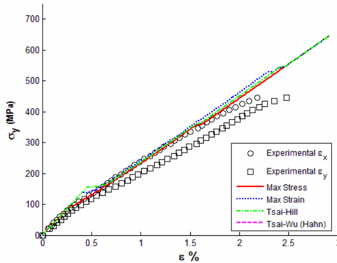
Figure 27. ±45° angle ply laminate E-glass/MY750/HY917/DY063: Stress/strain curve for \sigma_y/\sigma_x = 1/1 with GMC
