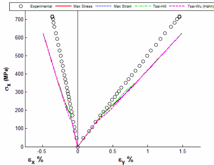
Figure 16. (0^\circ/\pm 45^\circ/90^\circ) laminate AS4/3501-6: Stress/strain curves for \sigma_y/\sigma_x = 0/1 with HFGMC
