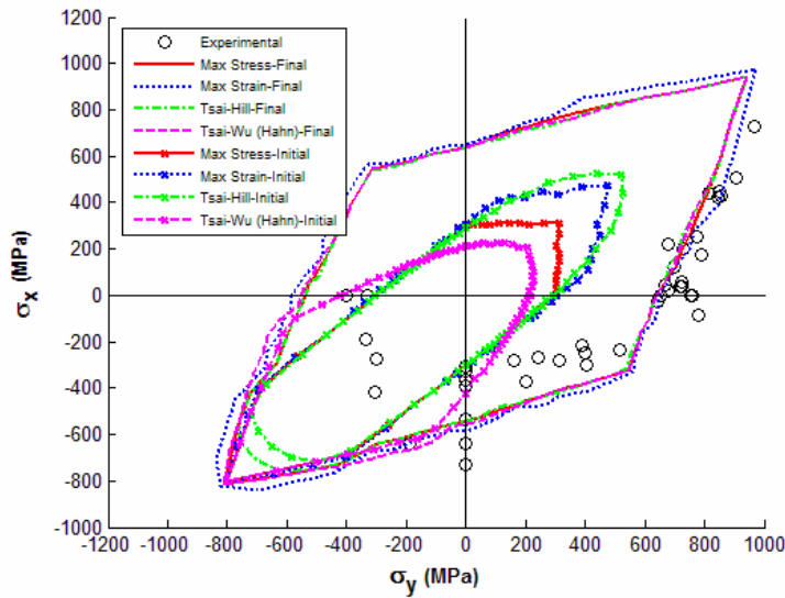
Figure 14. (0°/±45°/90°) laminate AS4/3501-6: \sigma_y vs \sigma_x failure stress envelope with HFGMC
