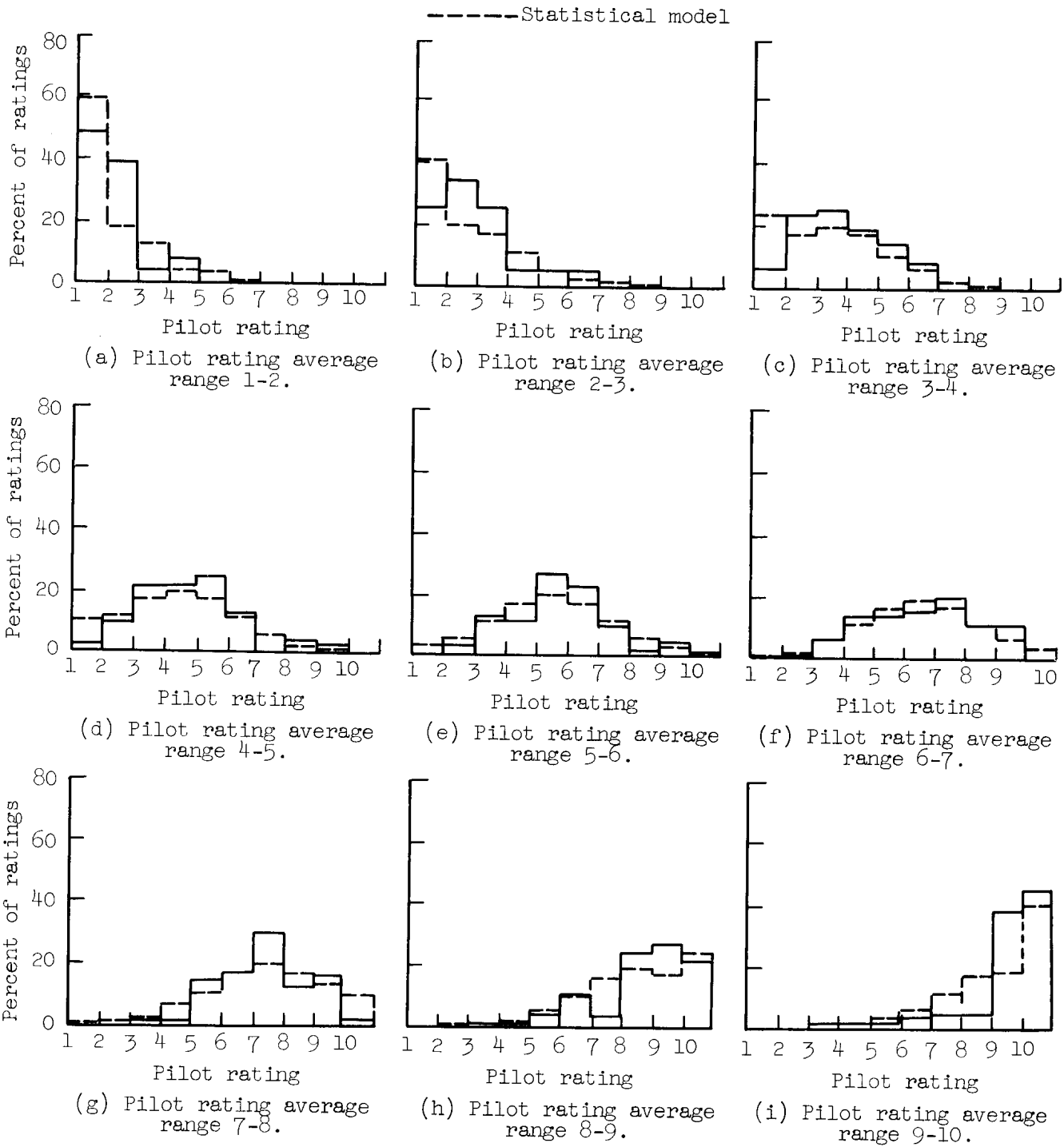
Figure 14. - Histograms for the variation in actual pilot ratings and the statistical model for various ranges of average pilot ratings.
