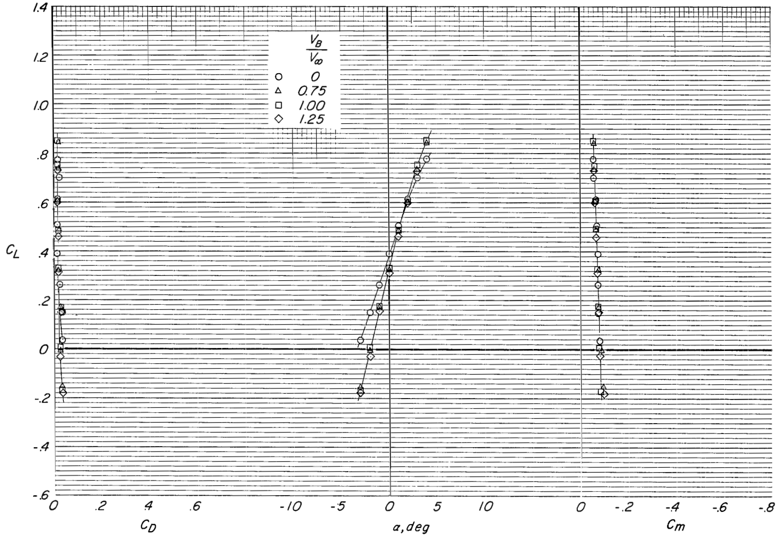
Figure 8.- Effect of variations in the velocity of the moving-belt ground plane on the longitudinal aerodynamic characteristics of the aspect-ratio-10 wing with flaps retracted and at a height-to-span ratio of 0.017.
