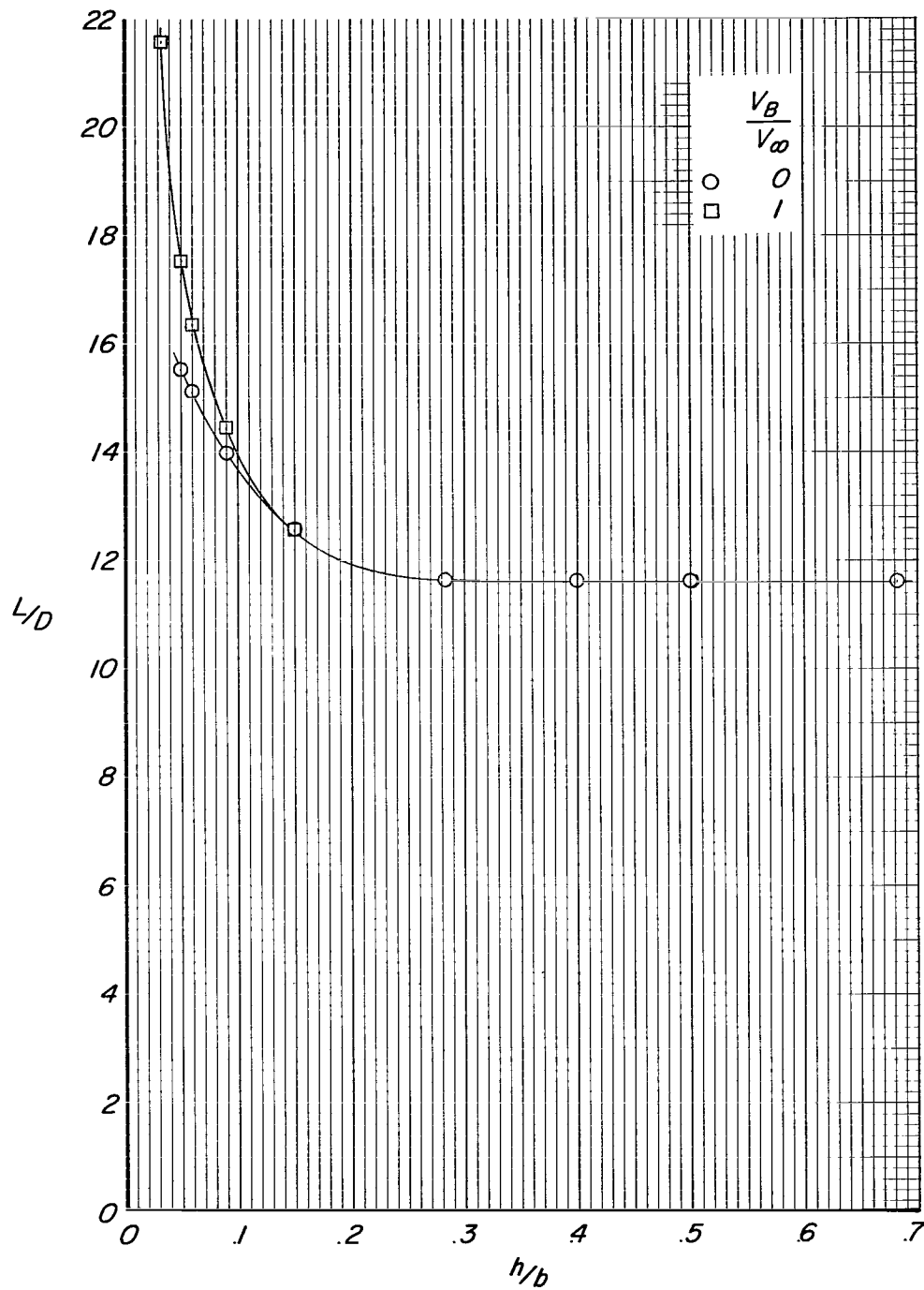
(g) Variation of lift-drag ratio with height-to-span ratio at C_L = 2 .
