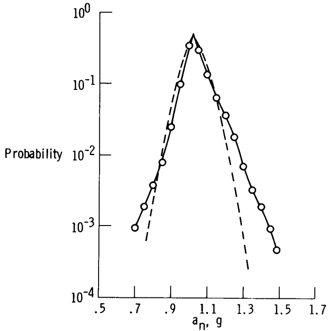
(e) Normal acceleration.
