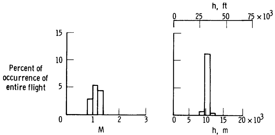
(b) Transonic acceleration.
