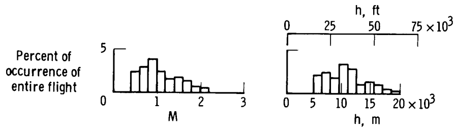
(e) Letdown.
