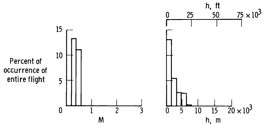
(f) Approach.
