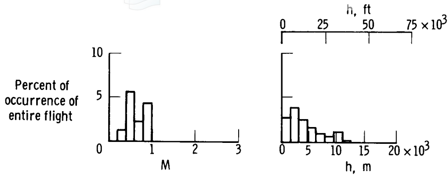
(a) Climbout.
