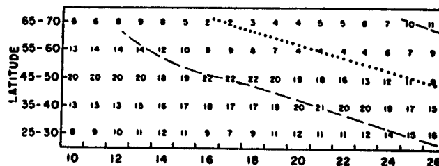
FIG. 5.2: Time section of zonal wind speed (mps) at 500 mb, November 10-26, 1950. Only one quarter of the calculated values is reproduced (every second 5° belt of latitude and every second day). Dashed lines denote relative maxima, and dotted lines relative minima of zonal wind speed [72].
