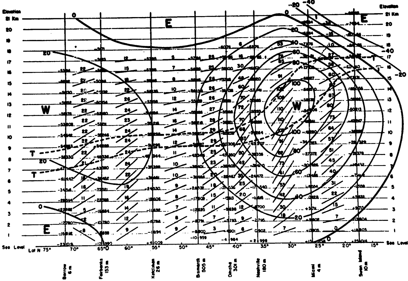
FIG. 1.3: Vertical cross-section of pressure (mb), temperature (°C) and wind (knots) for North America during winter [108].
