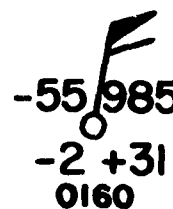
FIG. 6.1: Model for plotting upper-air data on constant pressure charts: -55° is temperature in °C; 985 is height in feet of 300-mb surface, first and last numbers omitted; +31 is height change in tens of feet; -2 is temperature change in °C; and 0160 is wind direction in tens of degrees and speed in knots, i.e., direction 10° and speed 60 knots. The direction is graphically represented by shaft. One barb is 10 knots, one triangle 50 knots.
