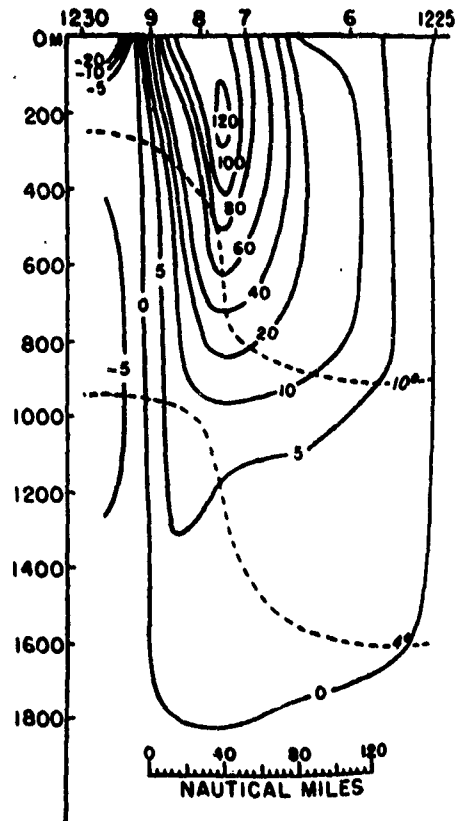
FIG. 7.2: Relationship between the distribution of temperature and current in Gulf Stream off Chesapeake Bay. Isotherms are given by broken cu. ves, current speed (cm/sec) by full lines [102].
