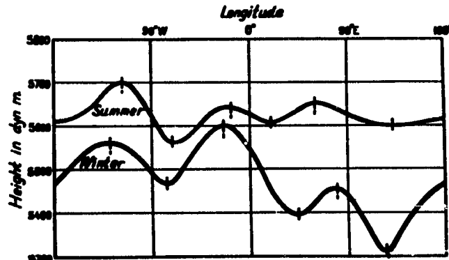
FIG. 3.18: The mean height of the 500-mb surface as a function of longitude. In summer the figure represents conditions in the latitude belt 45°N-50°N, in winter 35°N-40°N [14].
