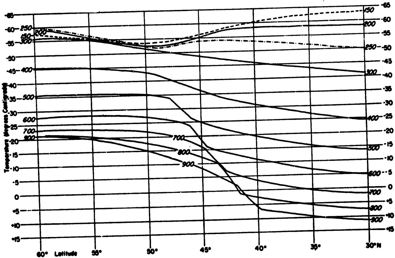
Fig. 2.20: Profiles of temperatures of isobaric surfaces (labeled in slanting numbers) taken from fig. 2.10. The latitudinal temperature gradient at any isobaric level may be judged by the slope of the profile [60].
