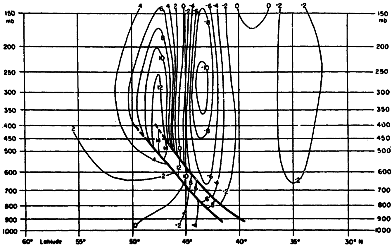
FIG. 2.12: Mean horizontal wind shear from fig. 2.10. Units are m/sec/(100 km), or 10^{-5} \text{ sec}^{-1} . Positive numbers indicate cyclonic shear; negative numbers, anticyclonic shear [60].
