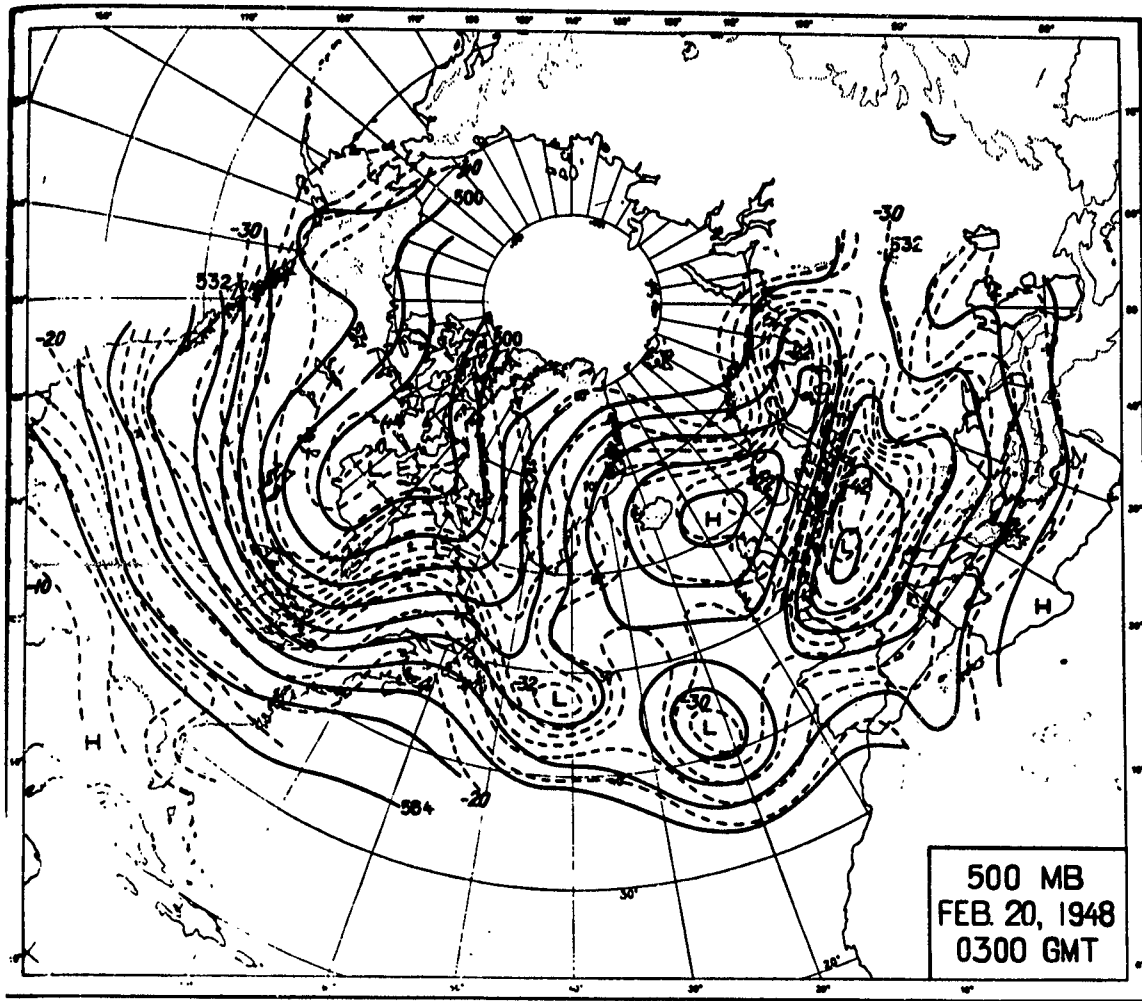
FIG. 2.17: Contours and isotherms on the 500-mb surface, 0300Z, February 20, 1948, showing a well-developed block [9].
