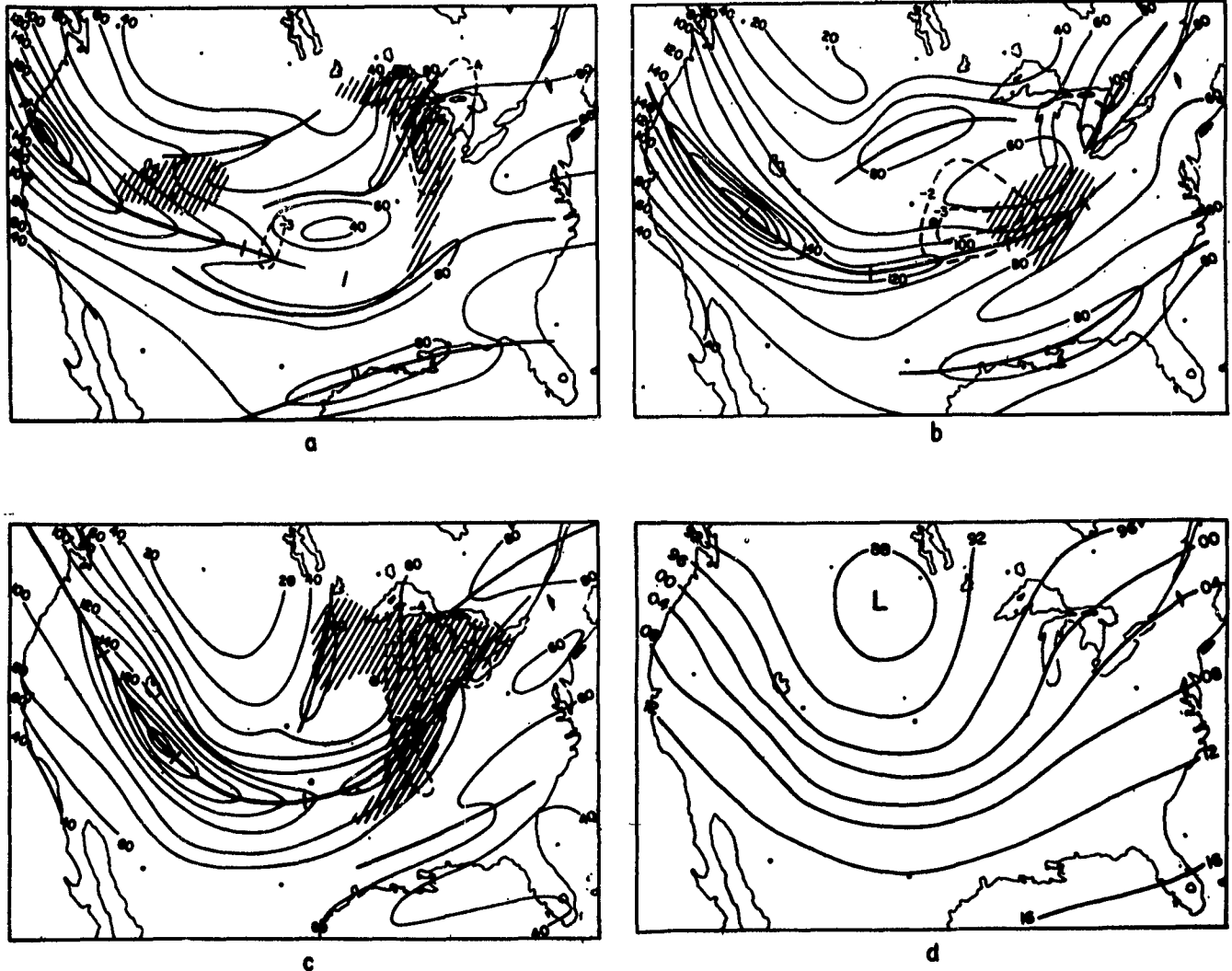
FIG. 4.3: a, b, c show the isotach pattern (thin solid lines) at 300 mb for November 12, 1951, 1500Z, and November 13, 1951, 0300Z and 1500Z. Shaded areas denote regions of precipitation; thick, solid lines join points of highest wind speed; broken lines are isolines of three-hour pressure fall at the surface; and heavy dots indicate the location of the lowest surface pressure. Fig. 4.3d represents the 300-mb contour field (100's feet, first digit omitted) at 1500Z November 13, 1951 [75].
