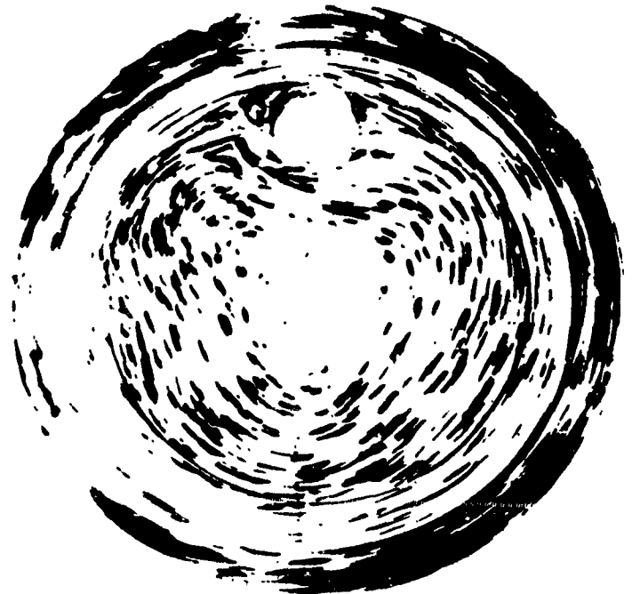
FIG. 7.11: Flow in a hemispheric shell relative to an obstacle, showing a well-defined wave pattern with a wave number of three. The obstacle is centered at lat. 45°. Its rate of rotation is approximately one-tenth of that of the shell. The North Pole is located at the center of the picture. The relative circulation (counter-clockwise) and its speed are indicated by the length of the streaks made by tracer particles. Notice the concentration of higher velocities downstream from obstacle (from records of Hydrodynamics Laboratory, University of Chicago).
