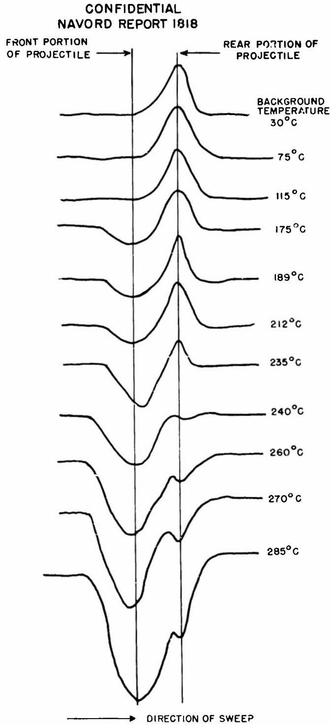
FIG. 6 TYPICAL SERIES OF OSCILLOSCOPE TRACES
